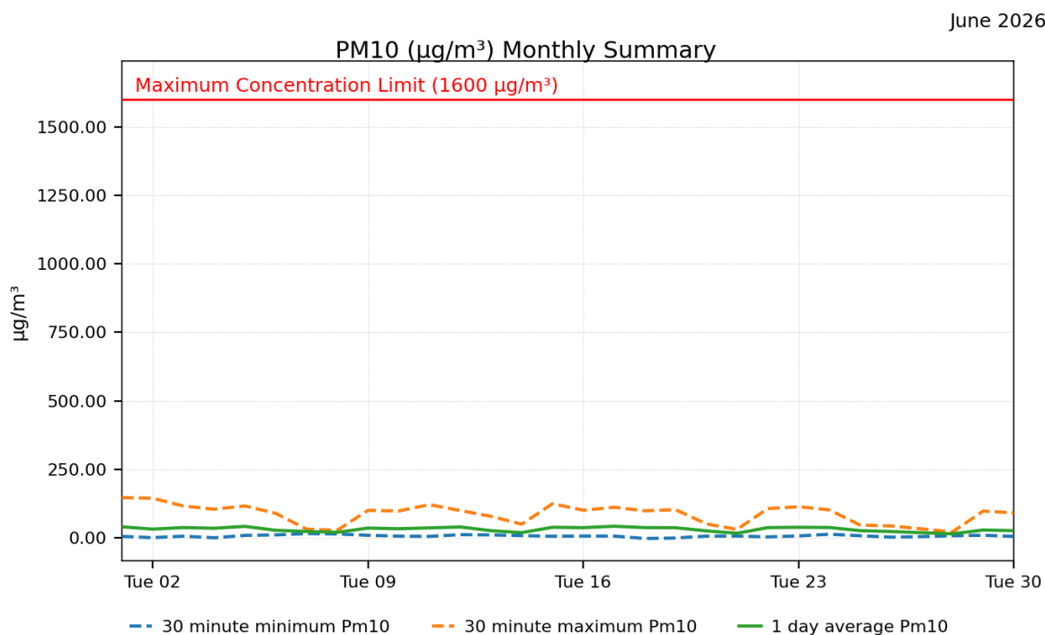
Figure 9. Sirius Rd PM 10 Averages
