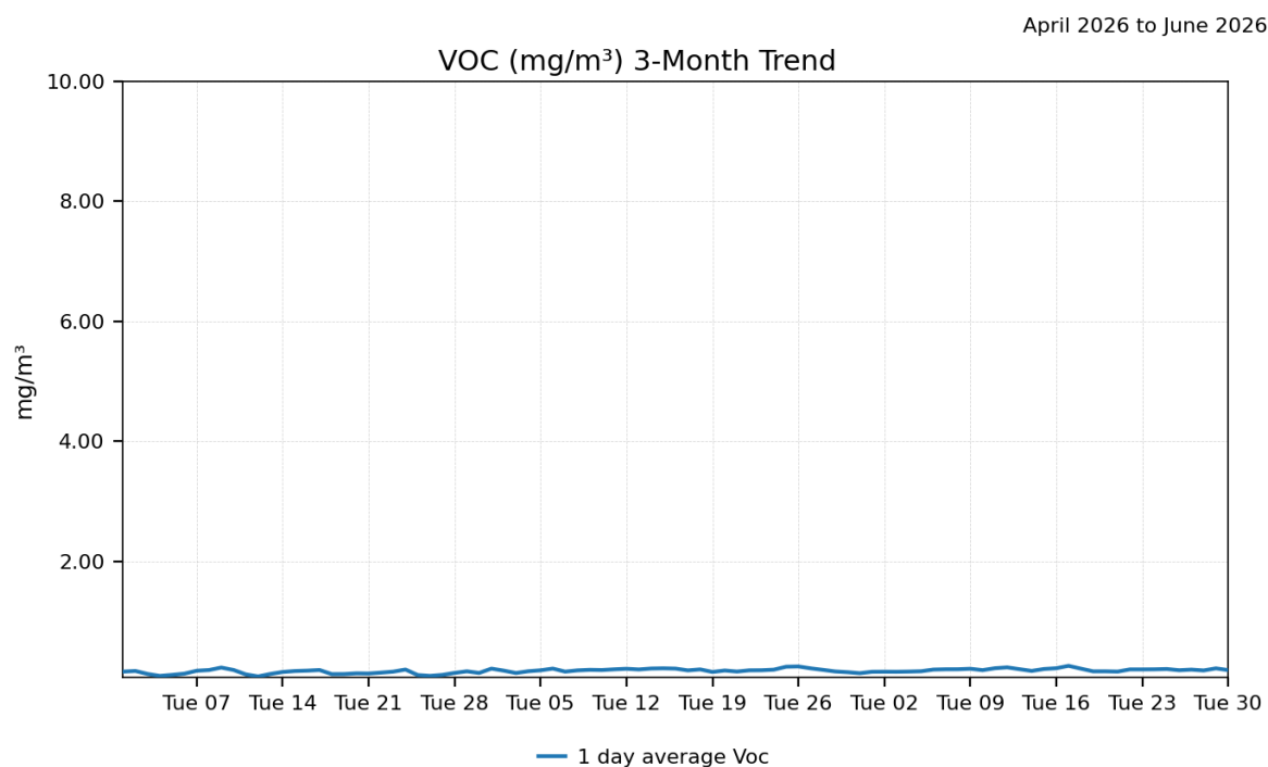
Figure 19. Sirius Rd Three Monthly VOC 1day Averages
