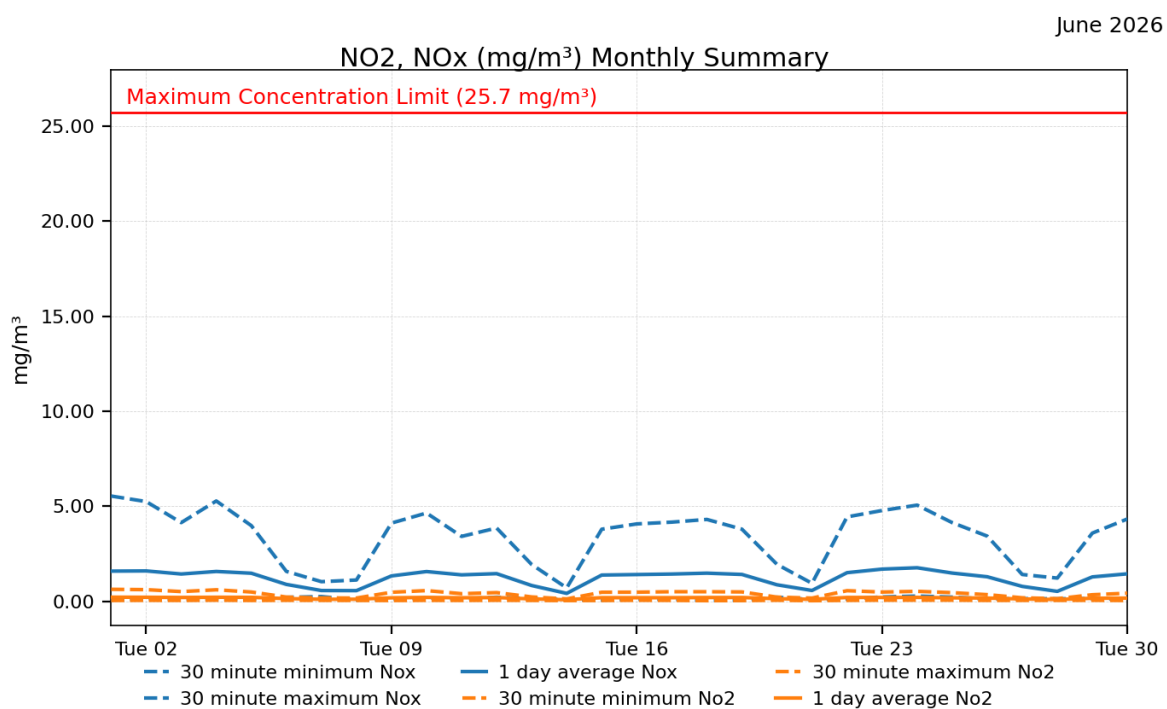
Figure 4. Marden St NO x , NO 2 Averages
