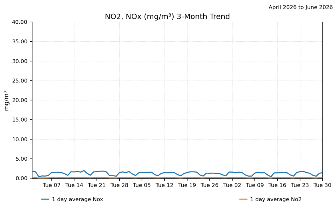
Figure 16. Marden St Three Monthly NO x , NO 2 1day Averages
