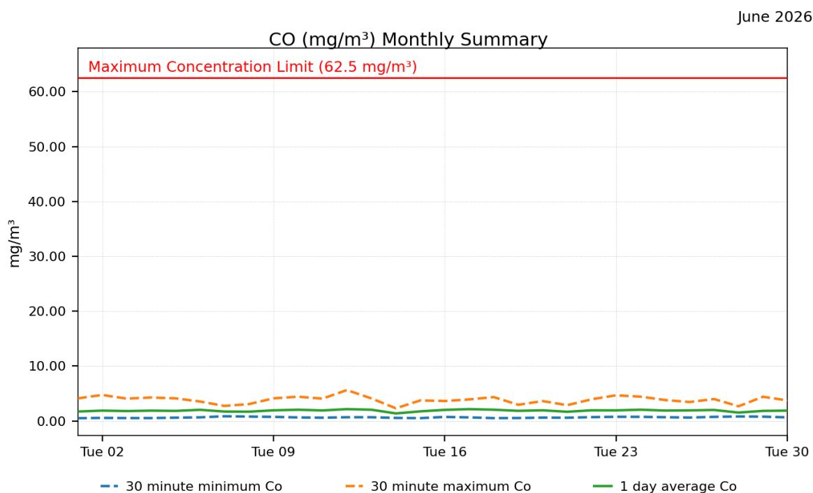
Figure 2. Marden St CO Averages
