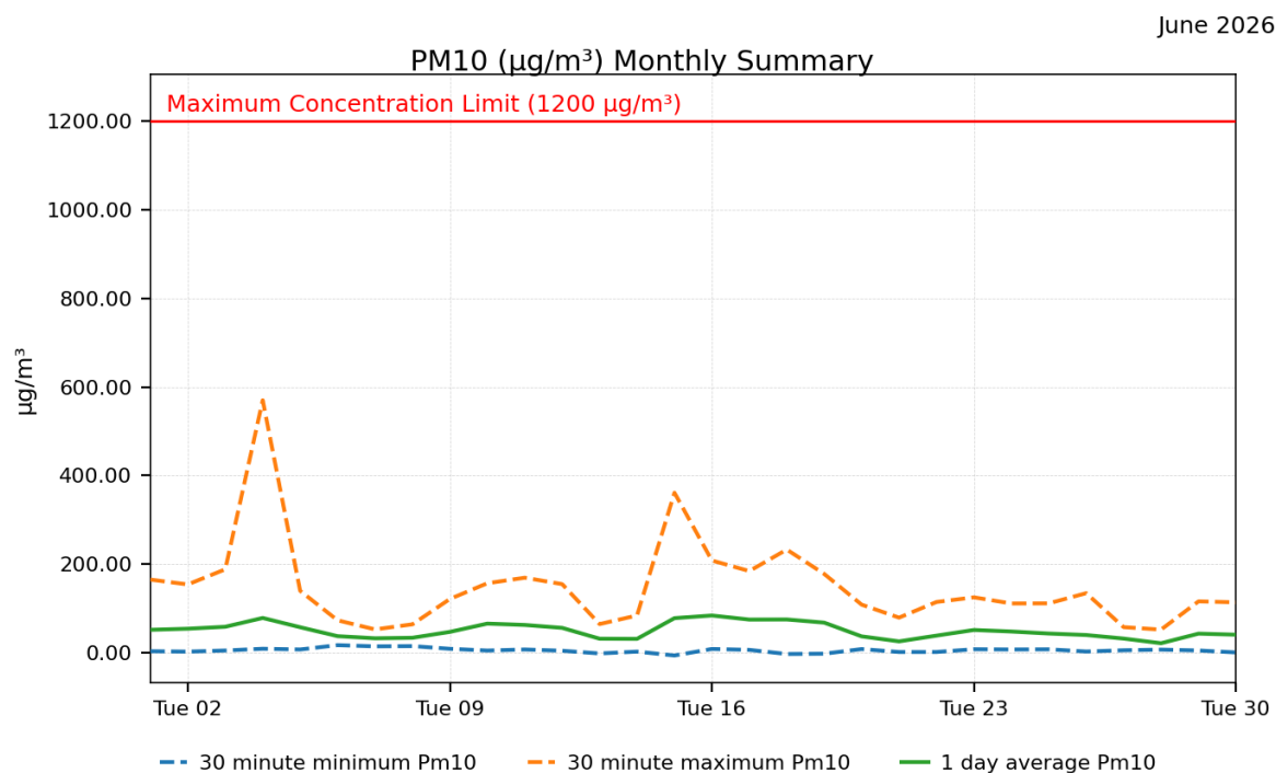
Figure 5. Marden St PM 10 Averages
