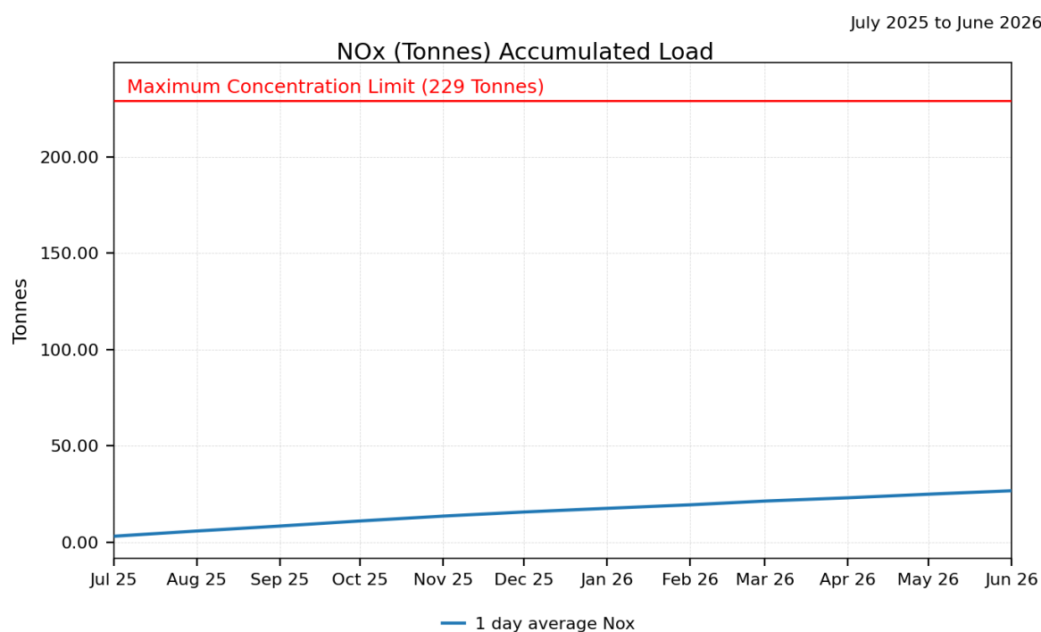
Figure 12. Combined Stacks NO x Accumulative Load
