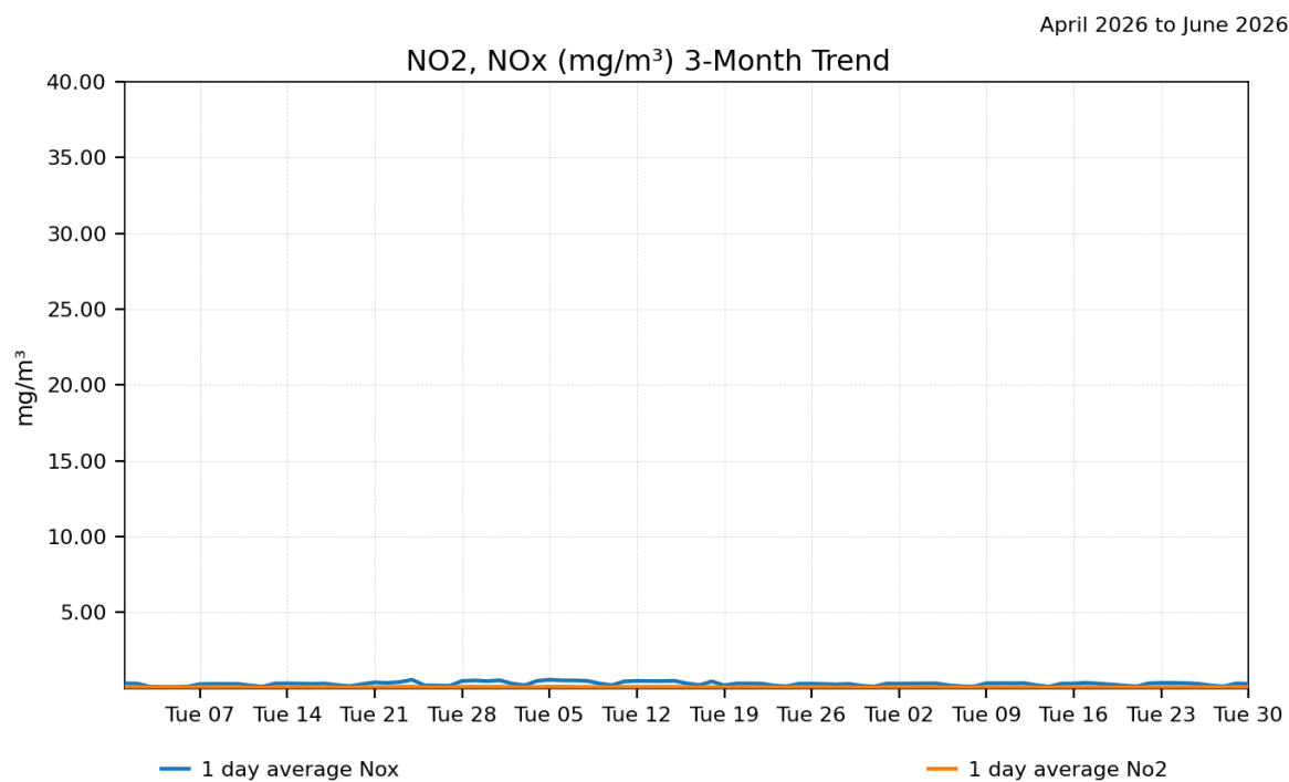
Figure 20. Sirius Rd Three Monthly NO x , NO 2 1day Averages
