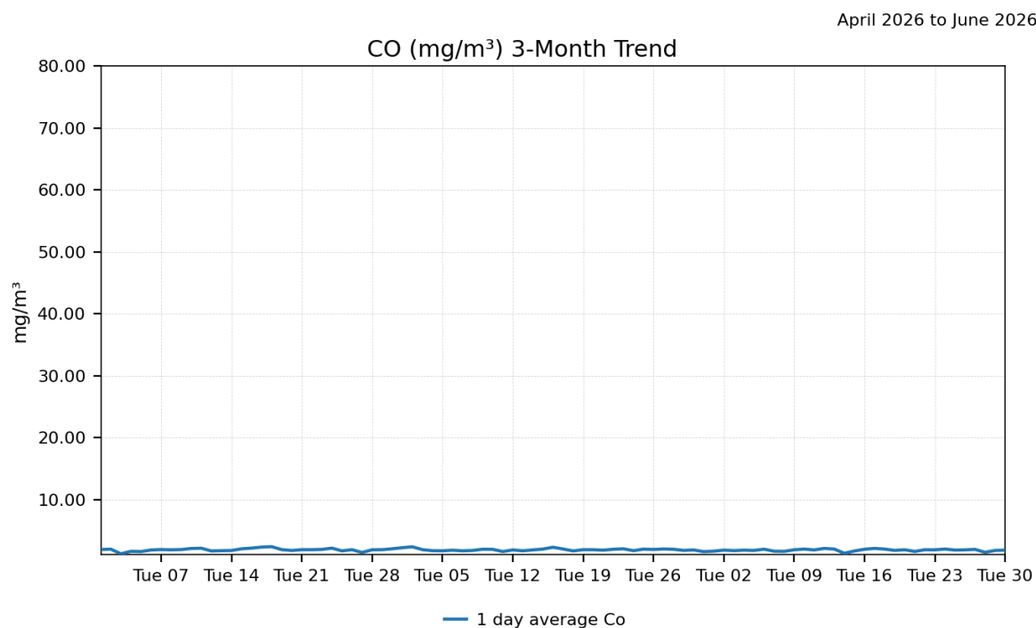
Figure 14. Marden St Three Monthly CO 1day Averages
