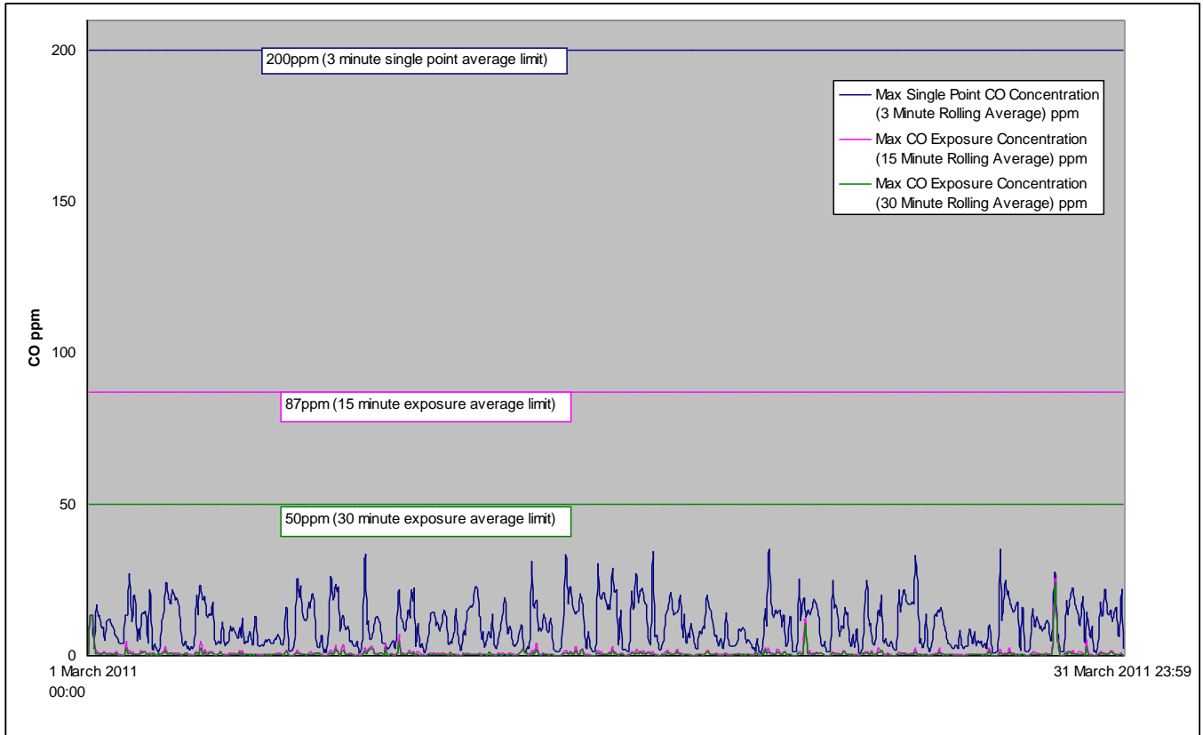
Figure 1: Graph of CO Exposure and Single Point Averages for 1 March 2011 – 31 March 2011.
