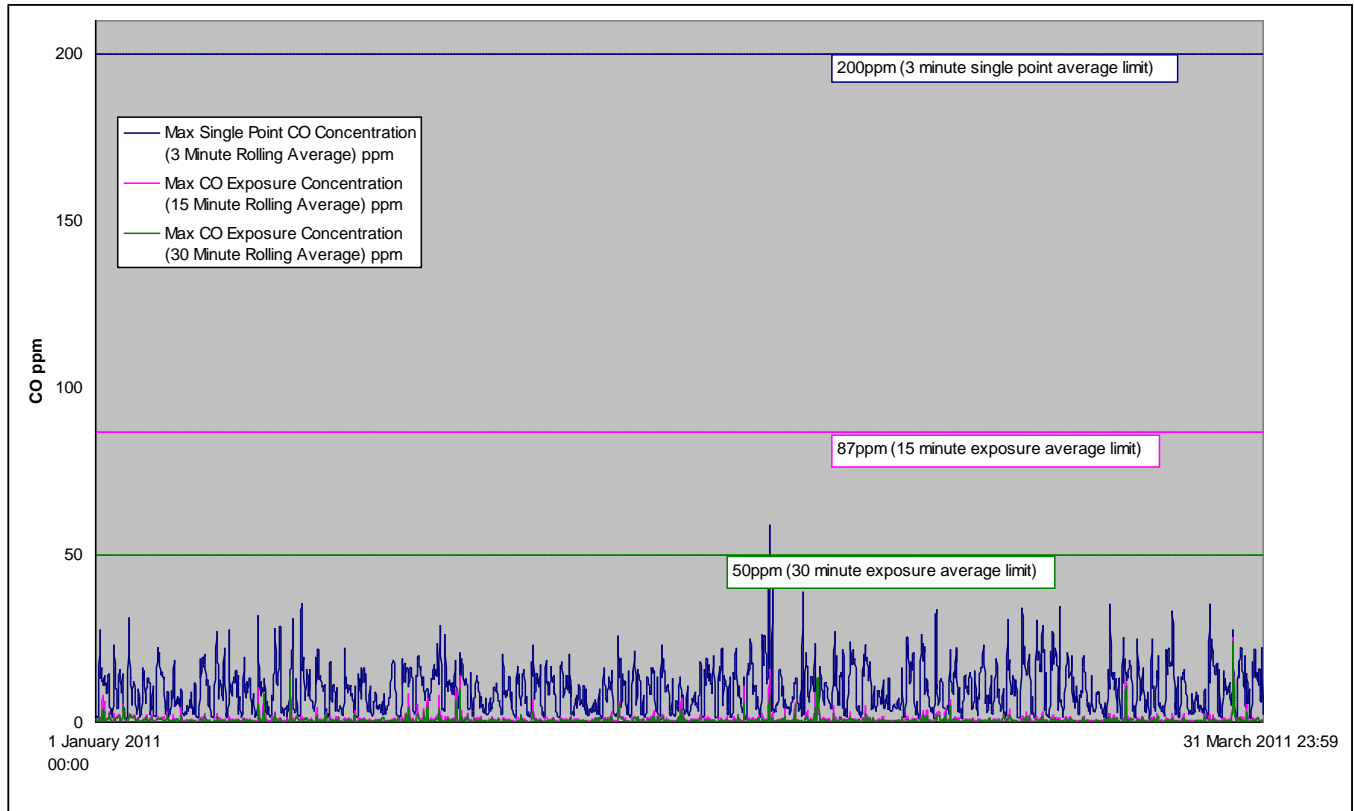
Figure 2: Graph of CO Exposure and Single Point Averages from 1 January 2011 – 31 March 2011.
