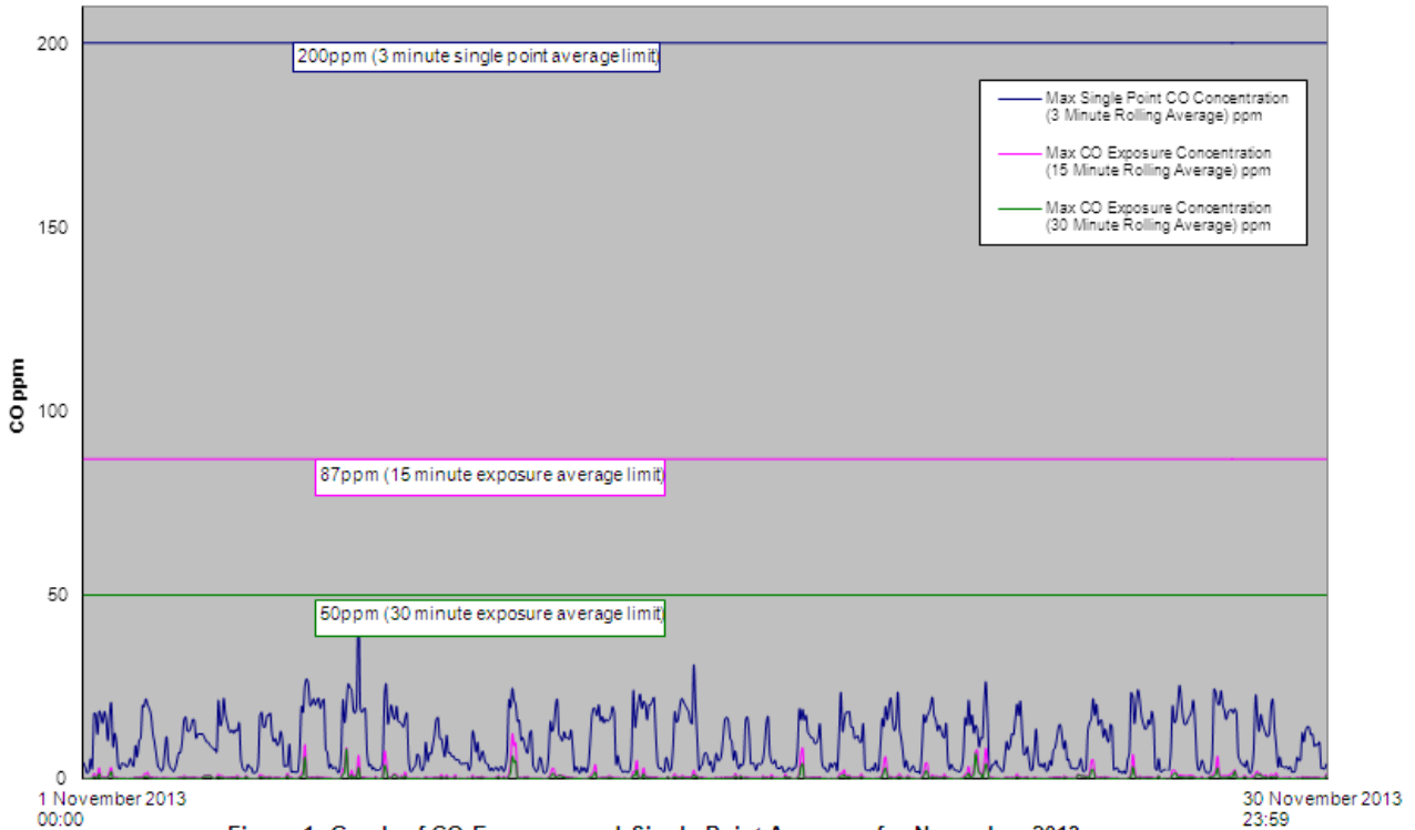
Figure 1: Graph of CO Exposure and Single Point Averages for November 2013
