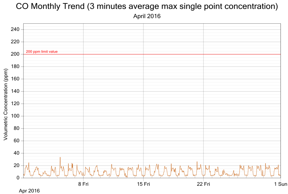
Figure 2: CO exposure and single point 3 minutes rolling averages for April 2016
