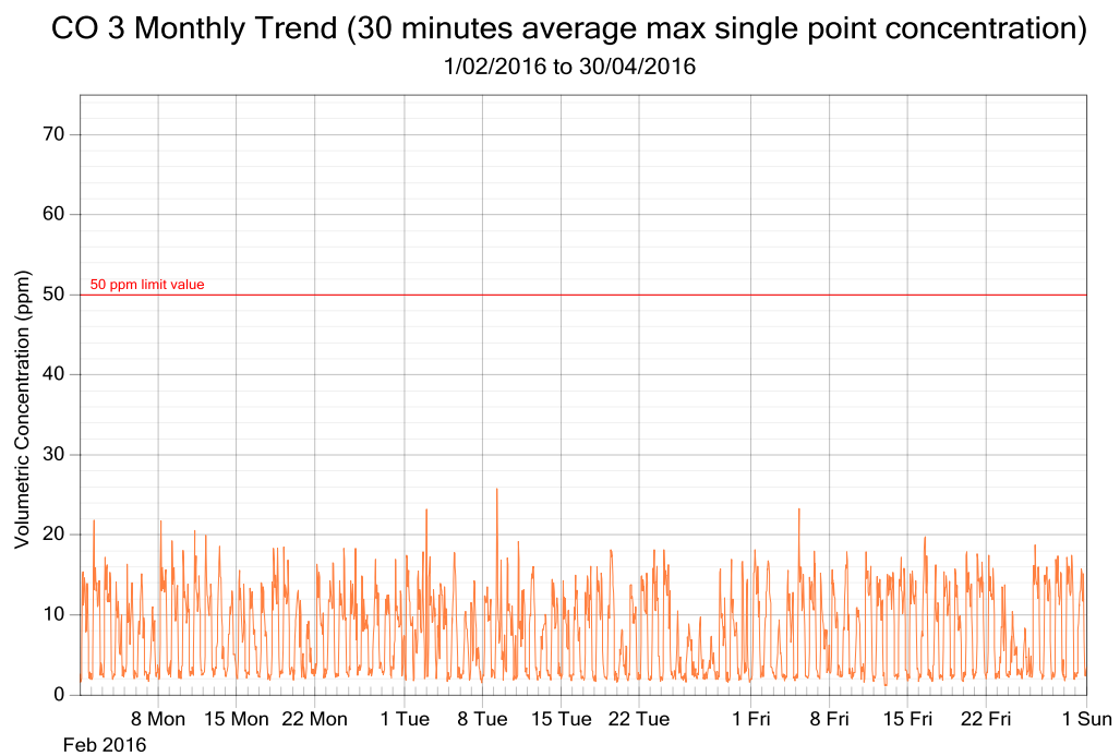
Figure 7: CO exposure and single point 30 minutes rolling averages from February 2016 to April 2016 (3 monthly trend)
