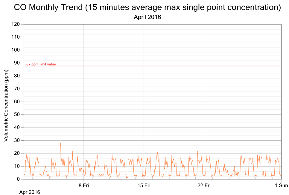
Figure 3: CO exposure and single point 15 minutes rolling averages for April 2016
