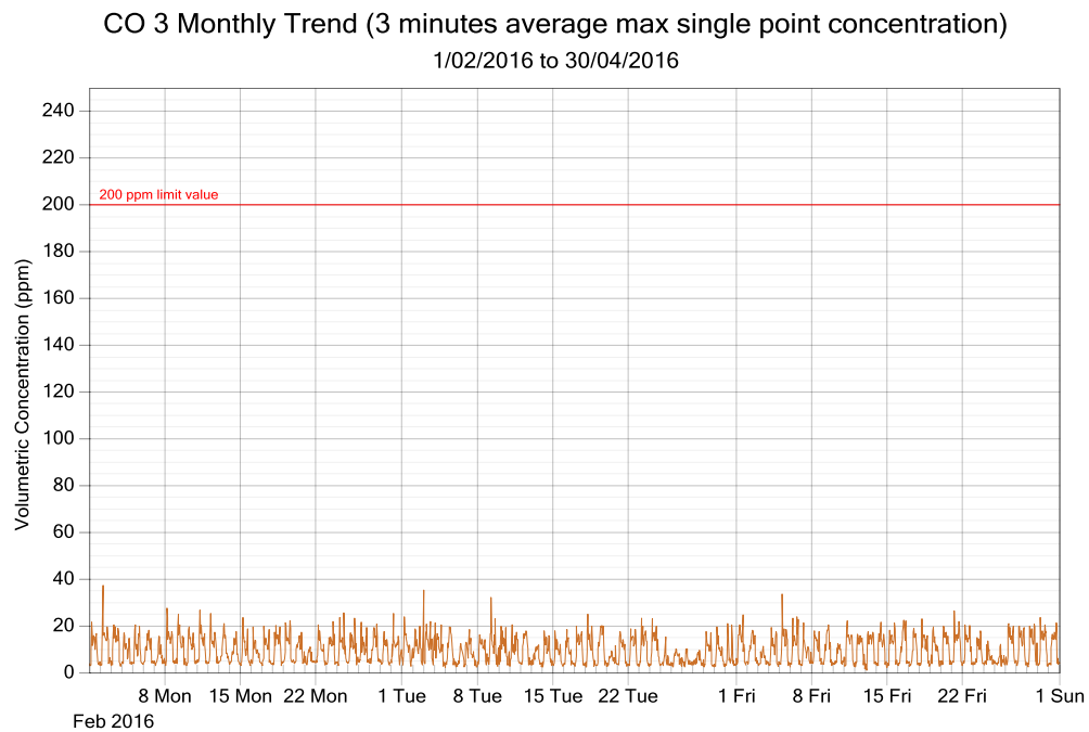
Figure 5: CO exposure and single point 3 minutes rolling averages from February 2016 to April 2016 (3 monthly trend)
