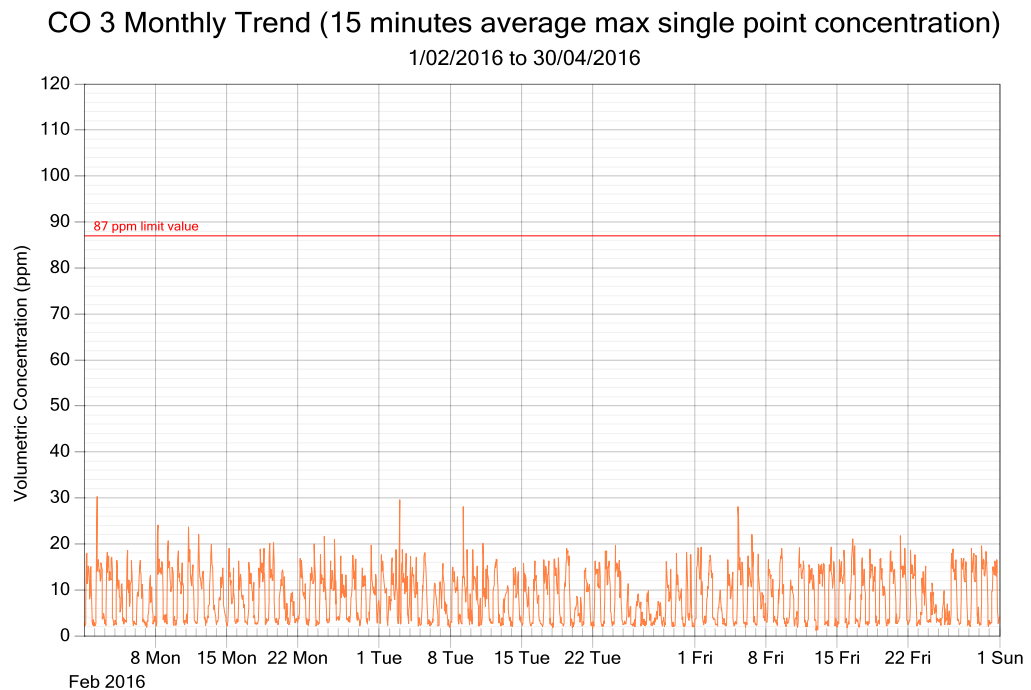
Figure 6: CO exposure and single point 15 minutes rolling averages from February 2016 to April 2016 (3 monthly trend)
