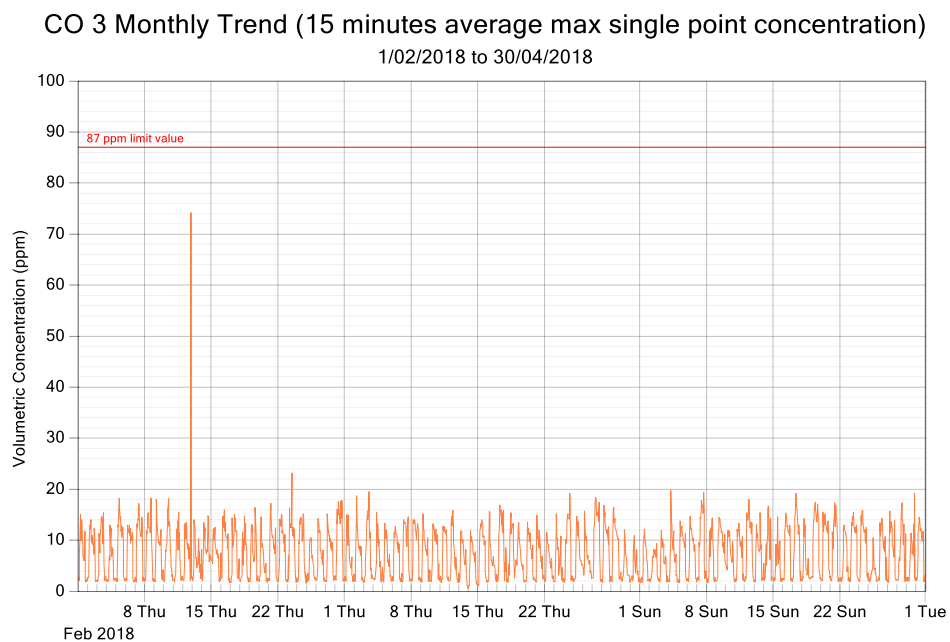
Figure 6: CO exposure and single point 15 minutes rolling averages from February 2018 to April 2018 (3 monthly trend)
