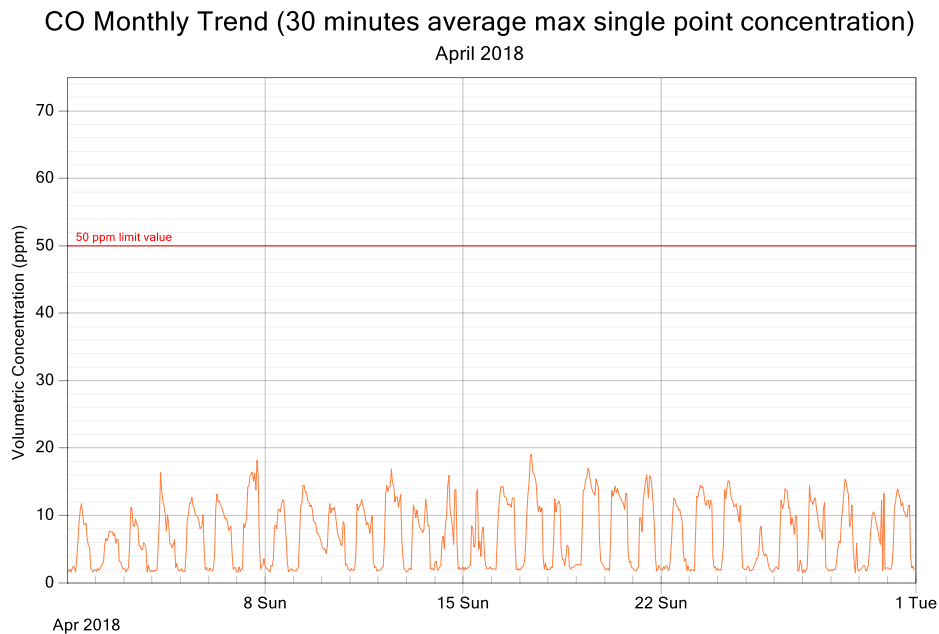
Figure 4: CO exposure and single point 30 minutes rolling averages for April 2018
