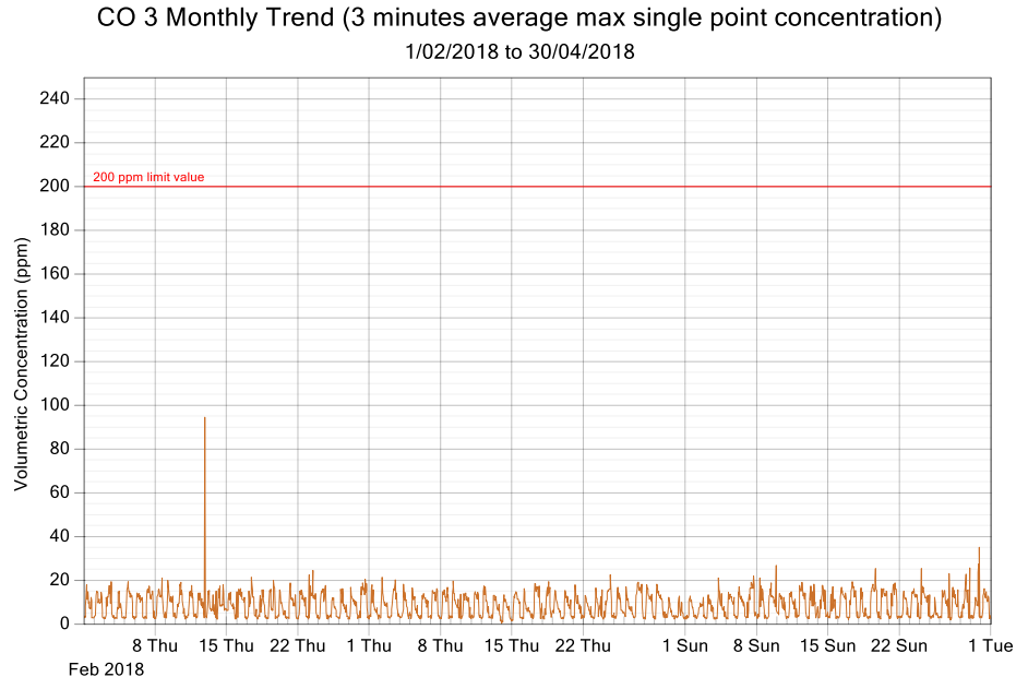
Figure 5: CO exposure and single point 3 minutes rolling averages from February 2018 to April 2018 (3 monthly trend)
