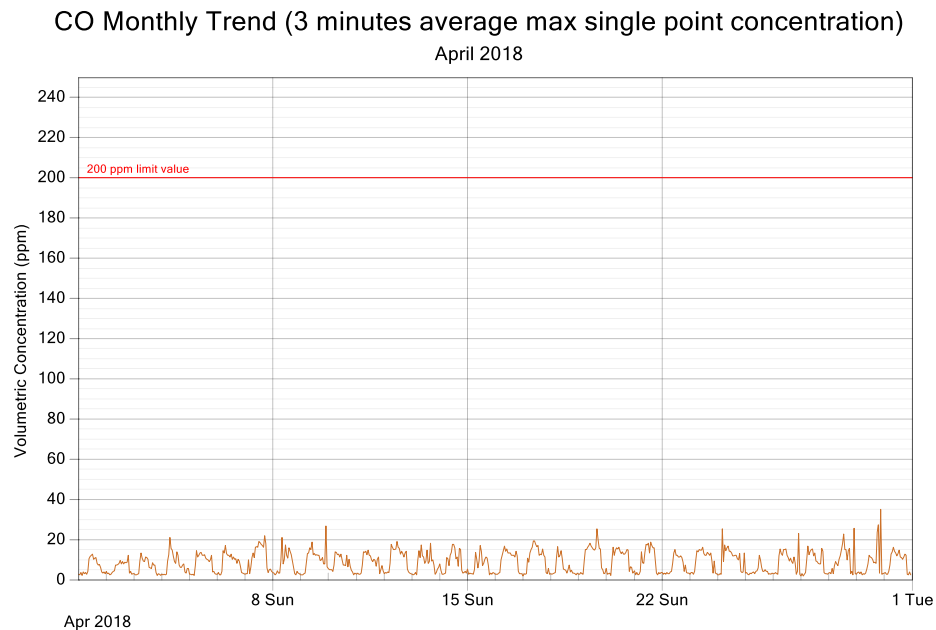
Figure 2: CO exposure and single point 3 minutes rolling averages for April 2018
