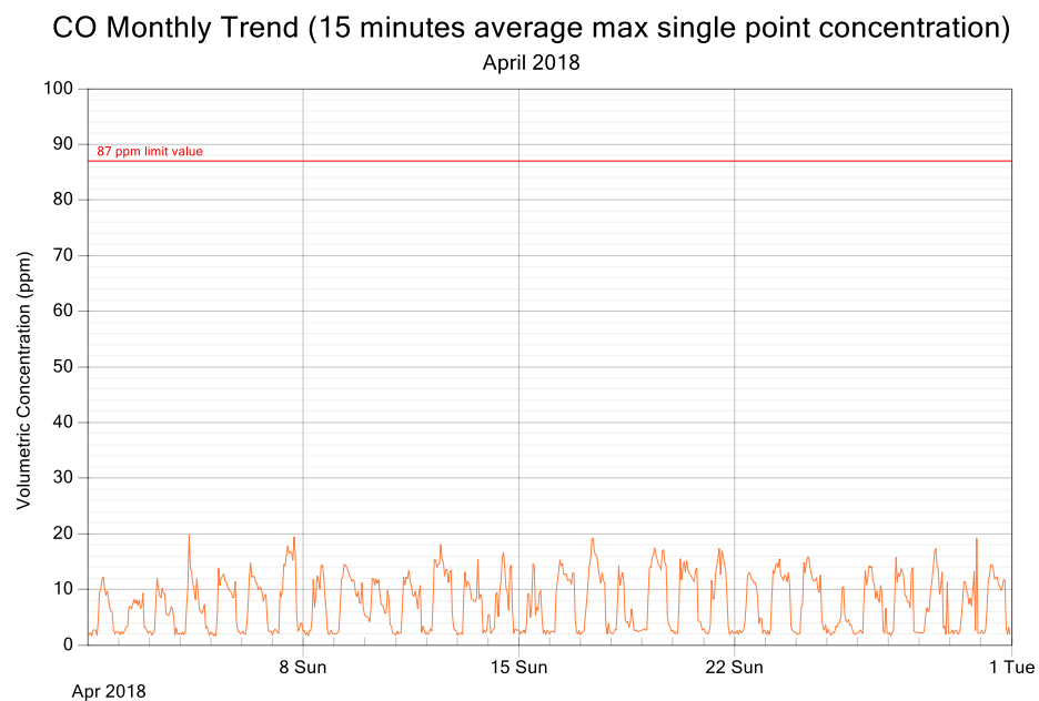
Figure 3: CO exposure and single point 15 minutes rolling averages for April 2018
