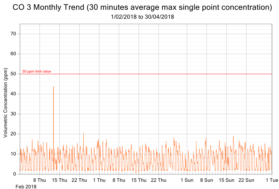
Figure 7: CO exposure and single point 30 minutes rolling averages from February 2018 to April 2018 (3 monthly trend)
