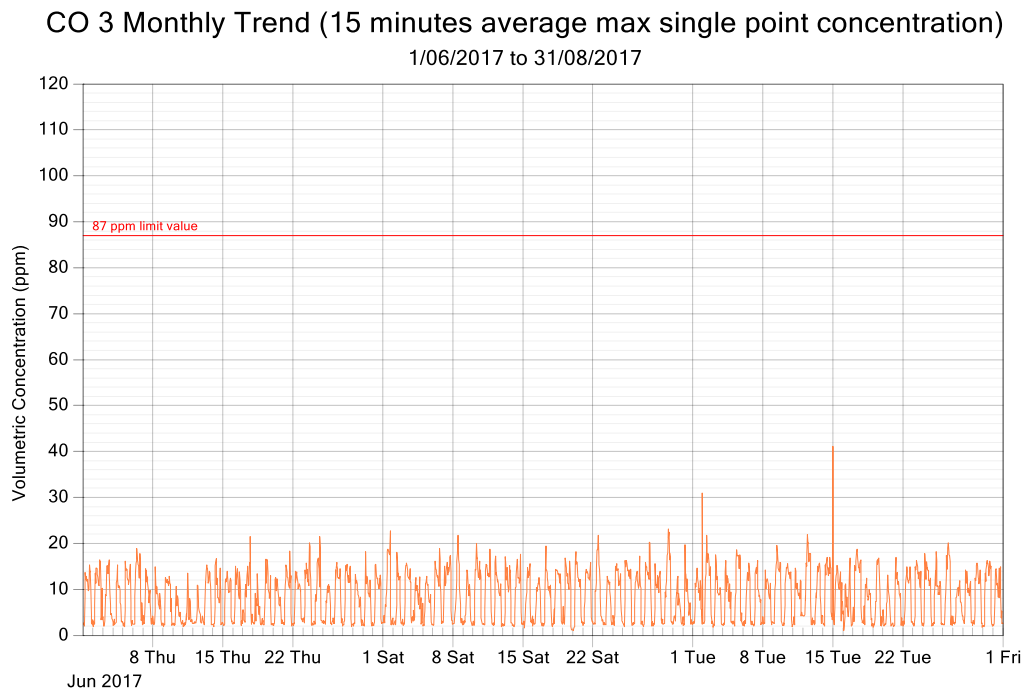
Figure 6: CO exposure and single point 15 minutes rolling averages from June 2017 to August 2017 (3 monthly trend)
