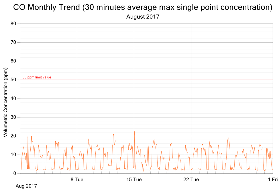
Figure 4: CO exposure and single point 30 minutes rolling averages for August 2017
