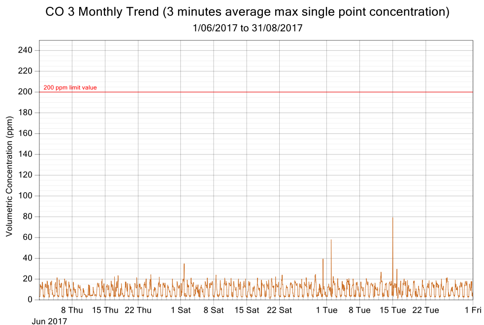
Figure 5: CO exposure and single point 3 minutes rolling averages from June 2017 to August 2017 (3 monthly trend)
