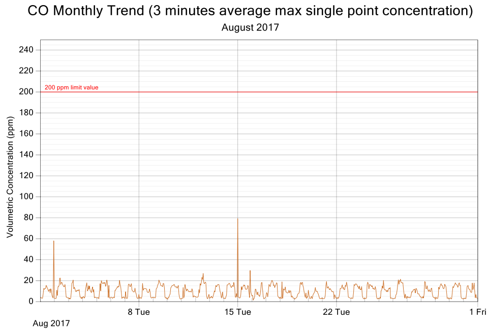
Figure 2: CO exposure and single point 3 minutes rolling averages for August 2017
