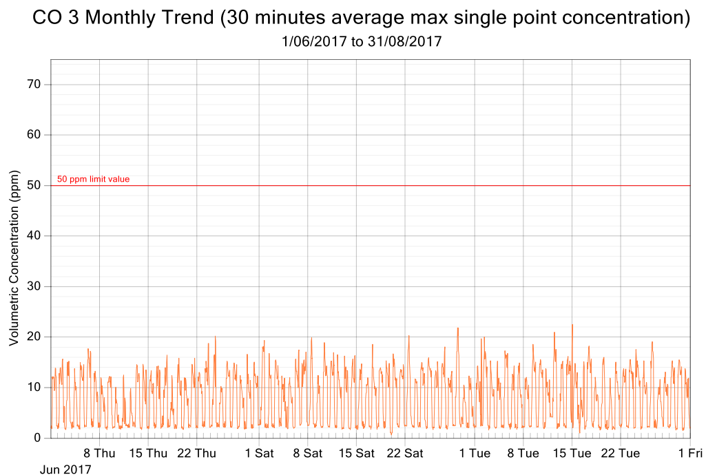
Figure 7: CO exposure and single point 30 minutes rolling averages from June 2017 to August 2017 (3 monthly trend)
