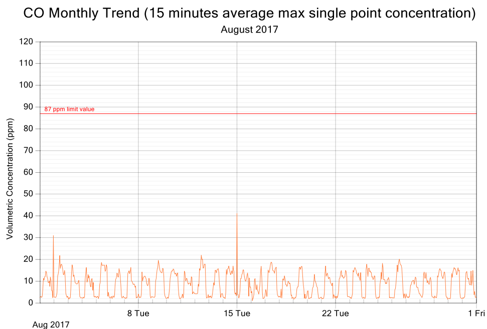
Figure 3: CO exposure and single point 15 minutes rolling averages for August 2017
