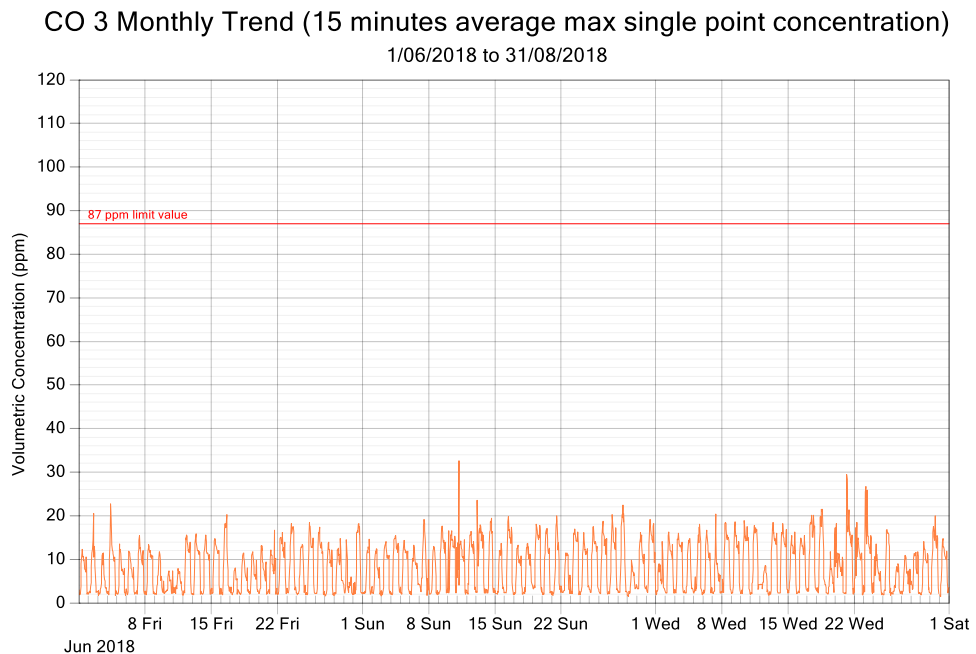
Figure 6: CO exposure and single point 15 minutes rolling averages from June 2018 to August 2018 (3 monthly trend)
