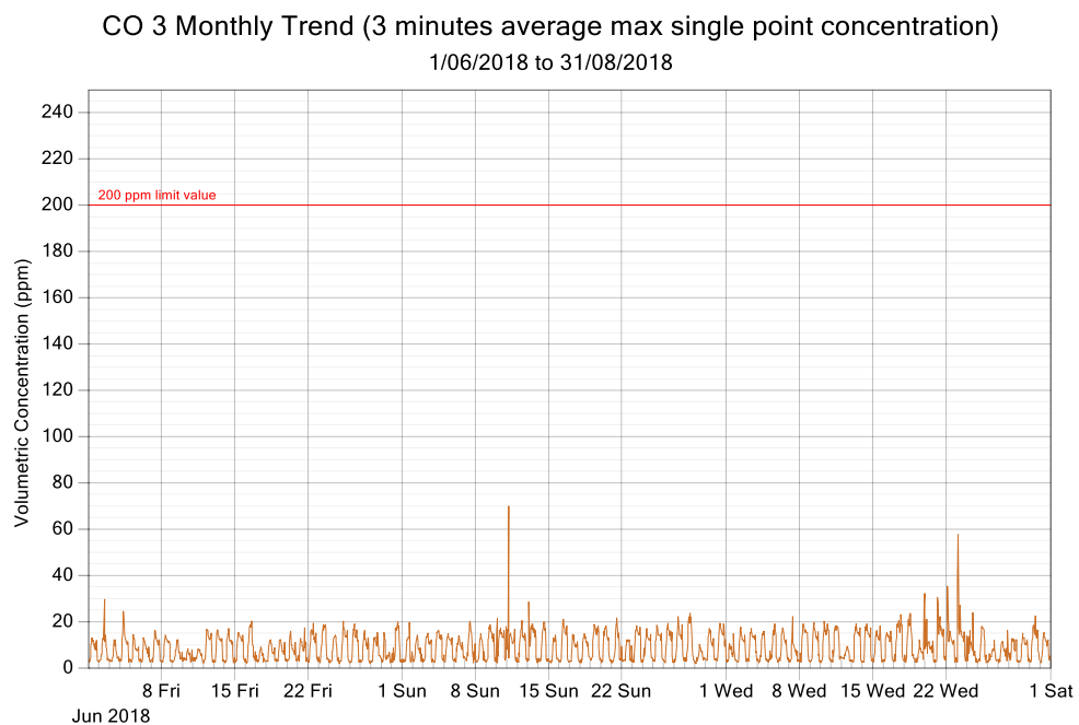
Figure 5: CO exposure and single point 3 minutes rolling averages from June 2018 to August 2018 (3 monthly trend)
