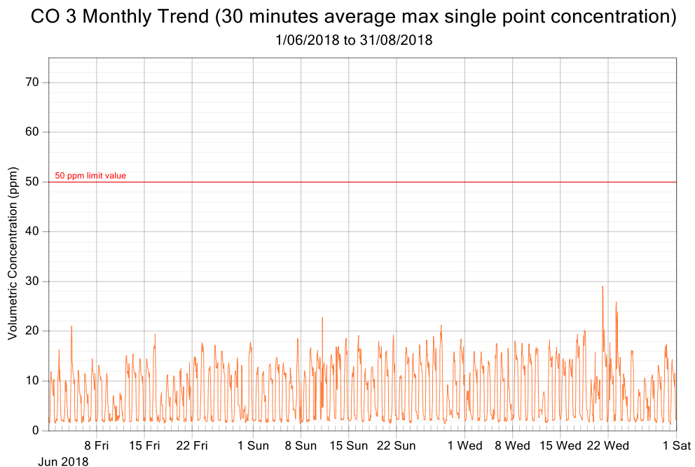
Figure 7: CO exposure and single point 30 minutes rolling averages from June 2018 to August 2018 (3 monthly trend)
