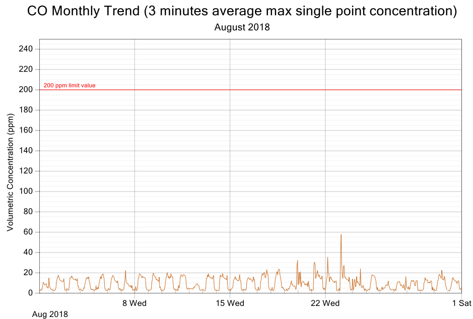
Figure 2: CO exposure and single point 3 minutes rolling averages for August 2018
