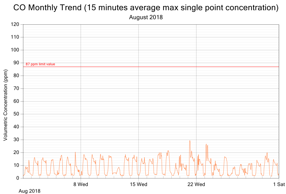
Figure 3: CO exposure and single point 15 minutes rolling averages for August 2018
