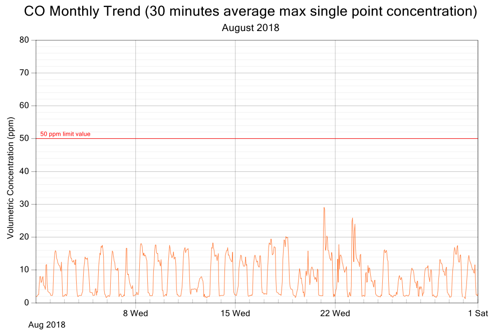
Figure 4: CO exposure and single point 30 minutes rolling averages for August 2018
