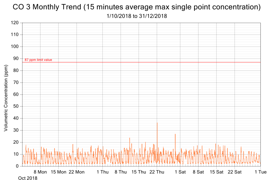
Figure 6: CO exposure and single point 15 minutes rolling averages from October 2018 to December 2018 (3 monthly trend)
