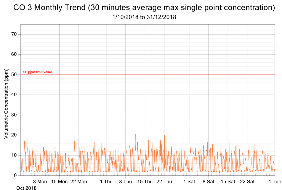
Figure 7: CO exposure and single point 30 minutes rolling averages from October 2018 to December 2018 (3 monthly trend)
