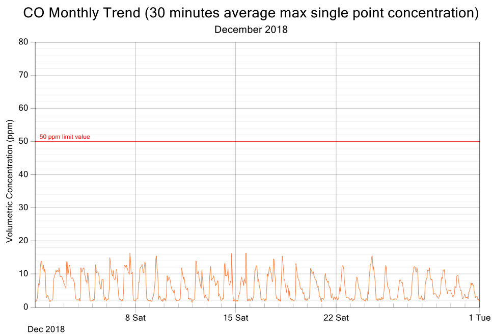
Figure 4: CO exposure and single point 30 minutes rolling averages for December 2018
