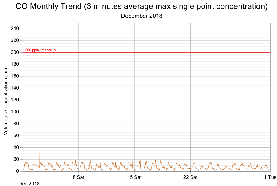
Figure 2: CO exposure and single point 3 minutes rolling averages for December 2018
