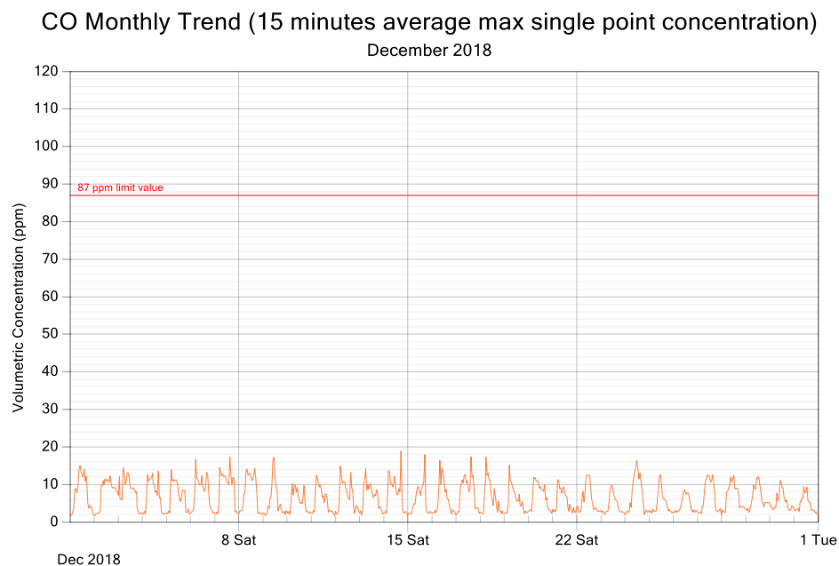
Figure 3: CO exposure and single point 15 minutes rolling averages for December 2018
