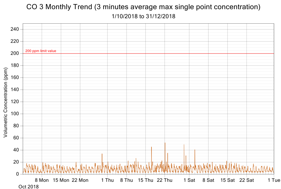
Figure 5: CO exposure and single point 3 minutes rolling averages from October 2018 to December 2018 (3 monthly trend)
