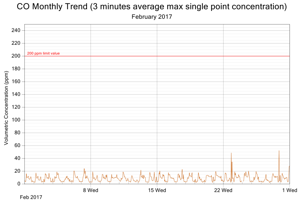
Figure 2: CO exposure and single point 3 minutes rolling averages for February 2017
