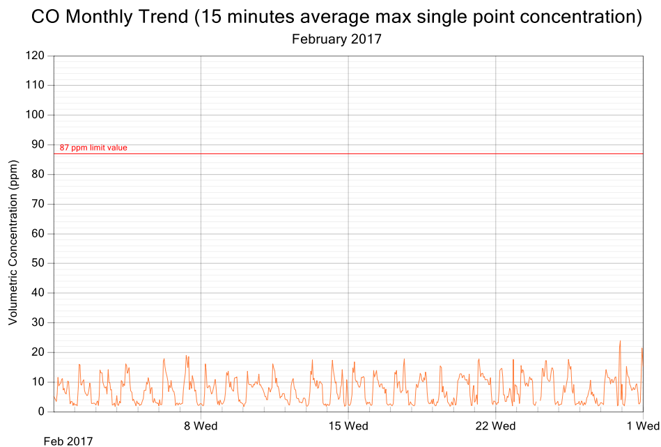
Figure 3: CO exposure and single point 15 minutes rolling averages for February 2017
