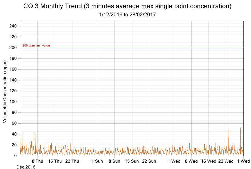
Figure 5: CO exposure and single point 3 minutes rolling averages from December 2017 to February 2017 (3 monthly trend)
