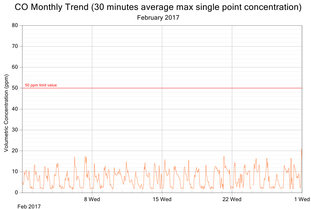
Figure 4: CO exposure and single point 30 minutes rolling averages for February 2017
