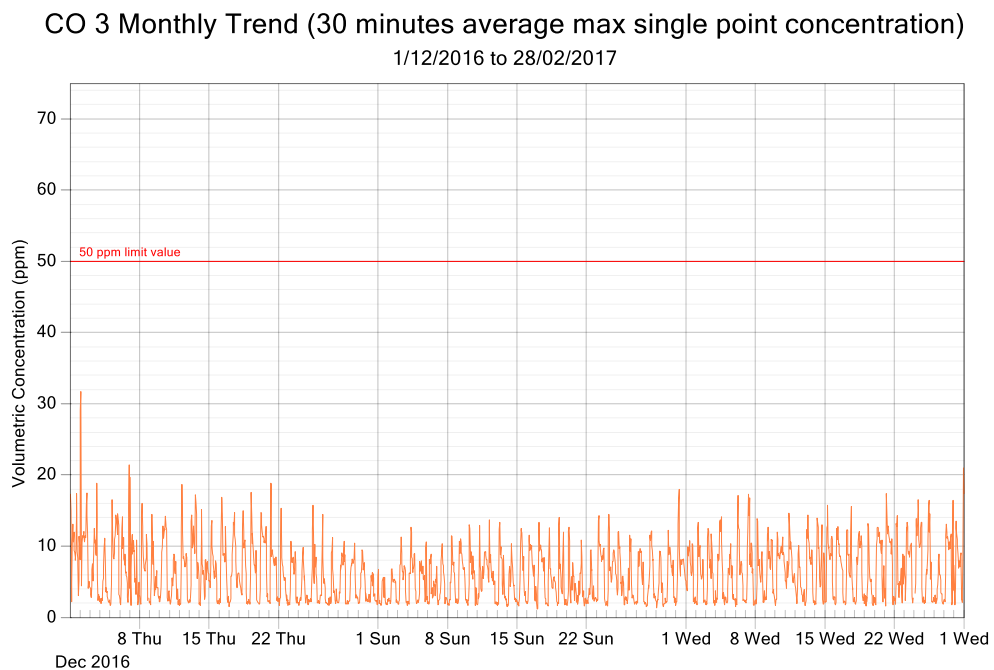
Figure 7: CO exposure and single point 30 minutes rolling averages from December 2017 to February 2017 (3 monthly trend)
