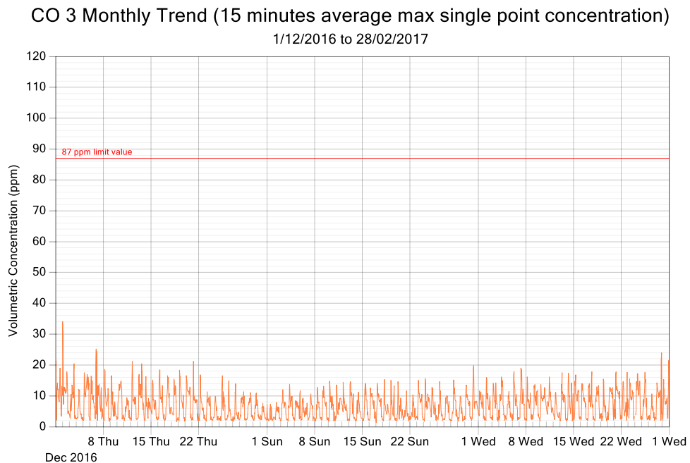
Figure 6: CO exposure and single point 15 minutes rolling averages from December 2017 to February 2017 (3 monthly trend)
