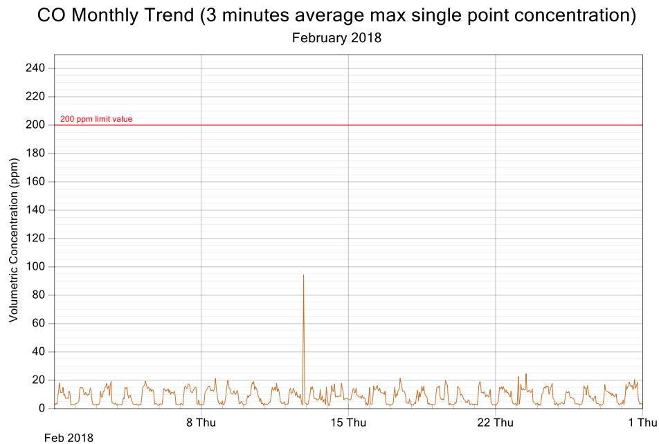
Figure 2: CO exposure and single point 3 minutes rolling averages for February 2018
