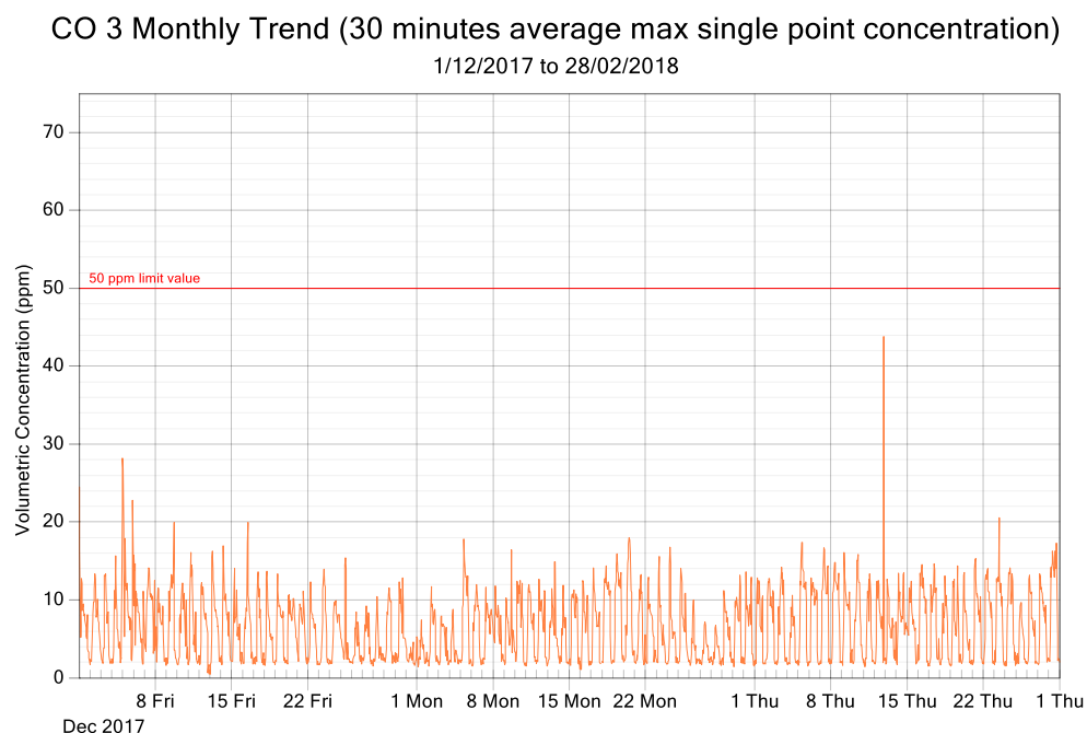
Figure 7: CO exposure and single point 30 minutes rolling averages from December 2017 to February 2018 (3 monthly trend)
