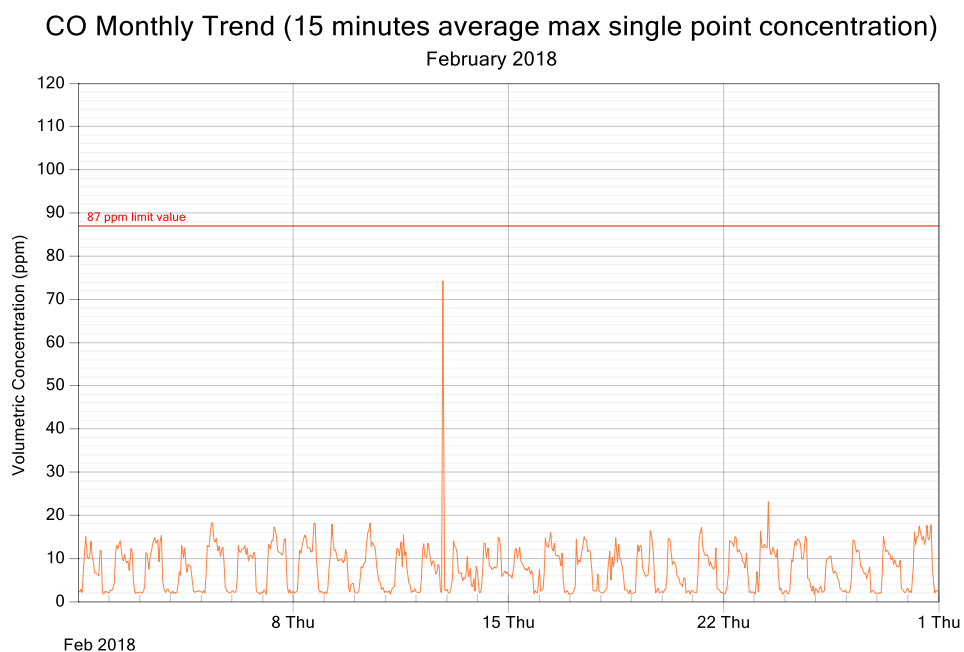
Figure 3: CO exposure and single point 15 minutes rolling averages for February 2018
