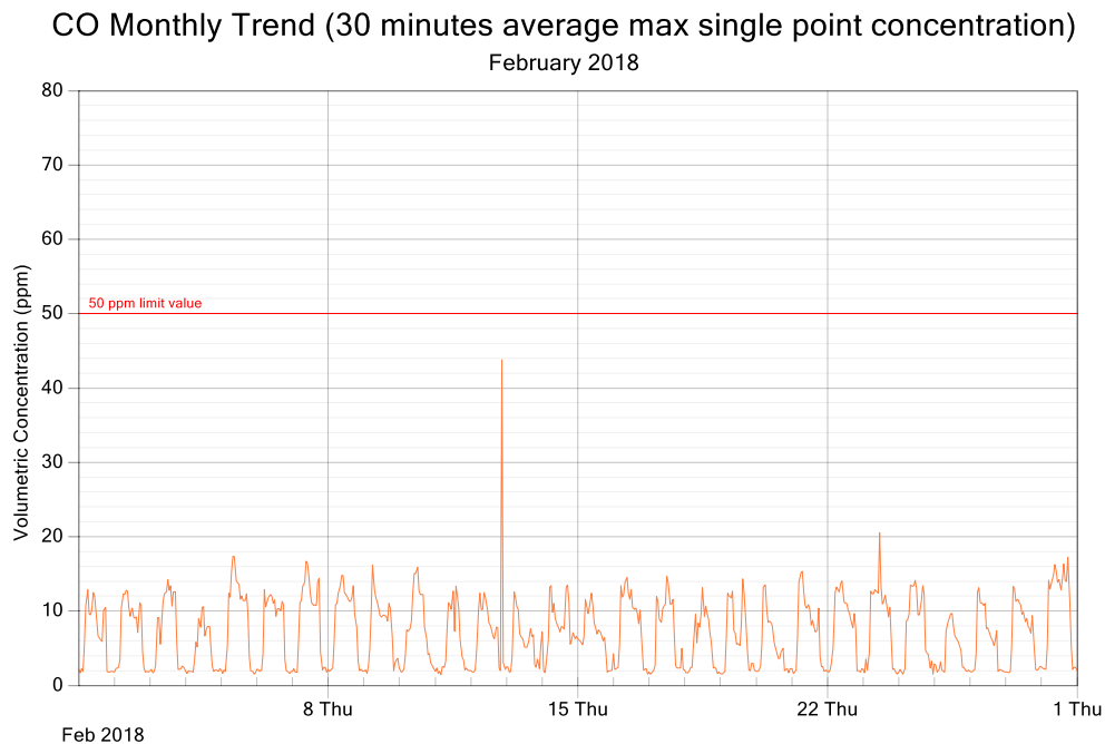
Figure 4: CO exposure and single point 30 minutes rolling averages for February 2018
