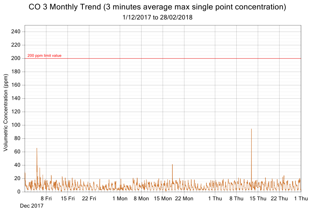
Figure 5: CO exposure and single point 3 minutes rolling averages from December 2017 to February 2018 (3 monthly trend)
