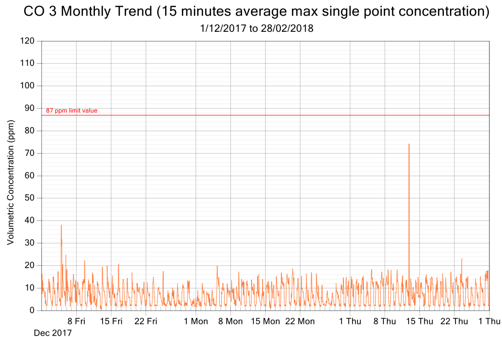
Figure 6: CO exposure and single point 15 minutes rolling averages from December 2017 to February 2018 (3 monthly trend)
