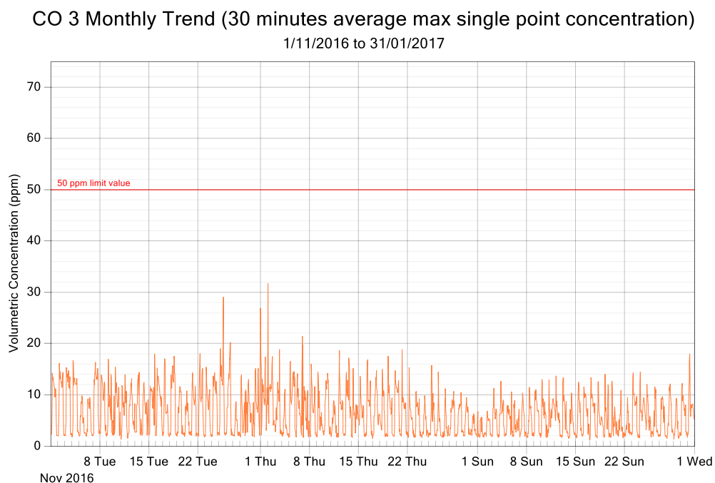
Figure 7: CO exposure and single point 30 minutes rolling averages from November 2016 to January 2017 (3 monthly trend)
