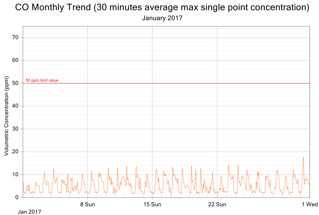
Figure 4: CO exposure and single point 30 minutes rolling averages for January 2017
