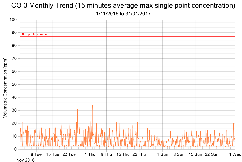
Figure 6: CO exposure and single point 15 minutes rolling averages from November 2016 to January 2017 (3 monthly trend)
