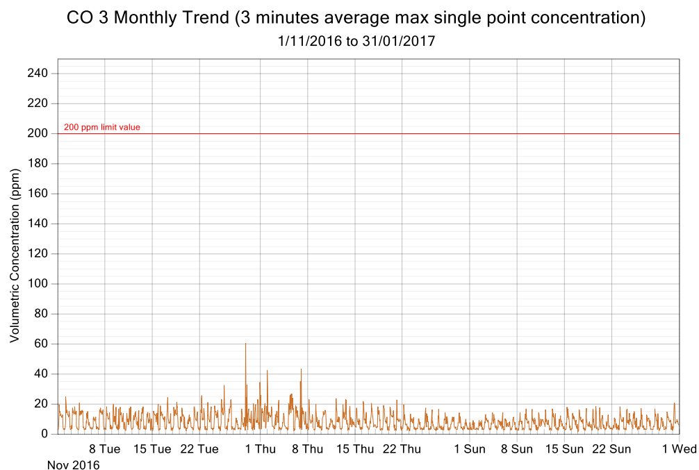
Figure 5: CO exposure and single point 3 minutes rolling averages from November 2016 to January 2017 (3 monthly trend)
