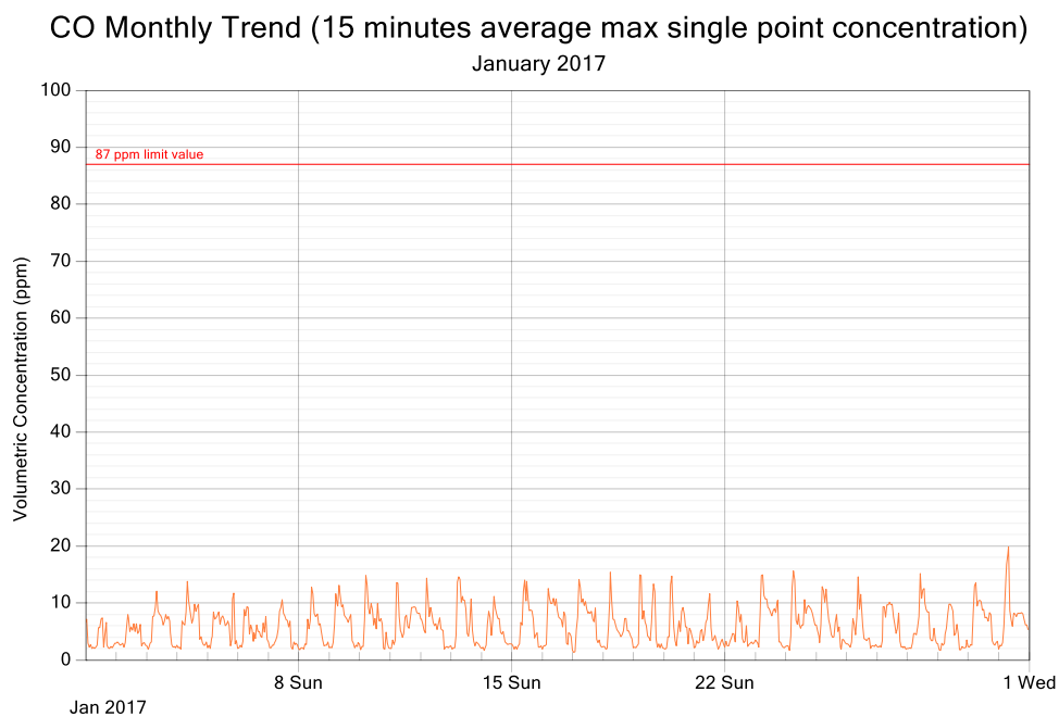
Figure 3: CO exposure and single point 15 minutes rolling averages for January 2017
