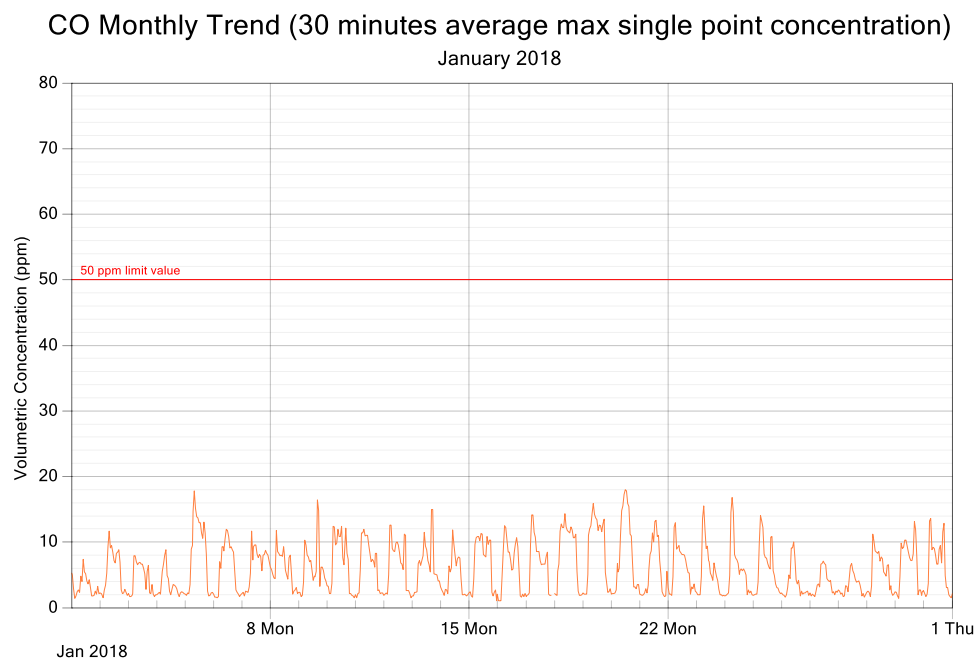
Figure 4: CO exposure and single point 30 minutes rolling averages for January 2018
