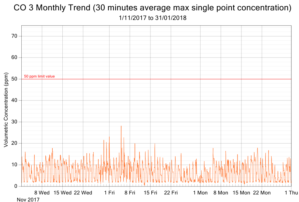
Figure 7: CO exposure and single point 30 minutes rolling averages from November 2017 to January 2018 (3 monthly trend)
