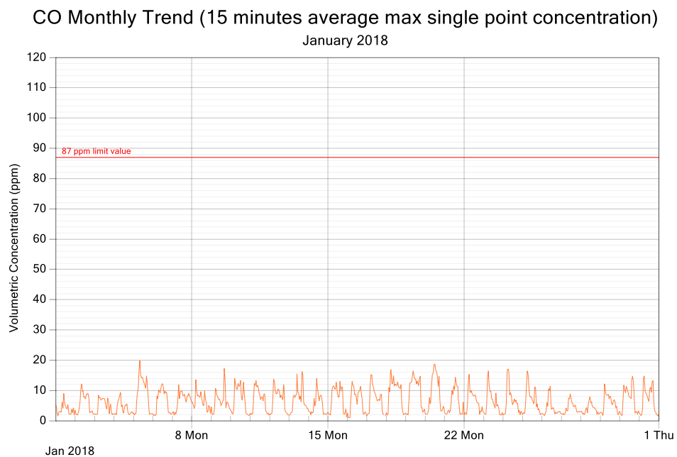
Figure 3: CO exposure and single point 15 minutes rolling averages for January 2018
