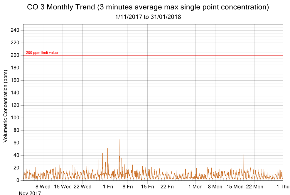
Figure 5: CO exposure and single point 3 minutes rolling averages from November 2017 to January 2018 (3 monthly trend)
