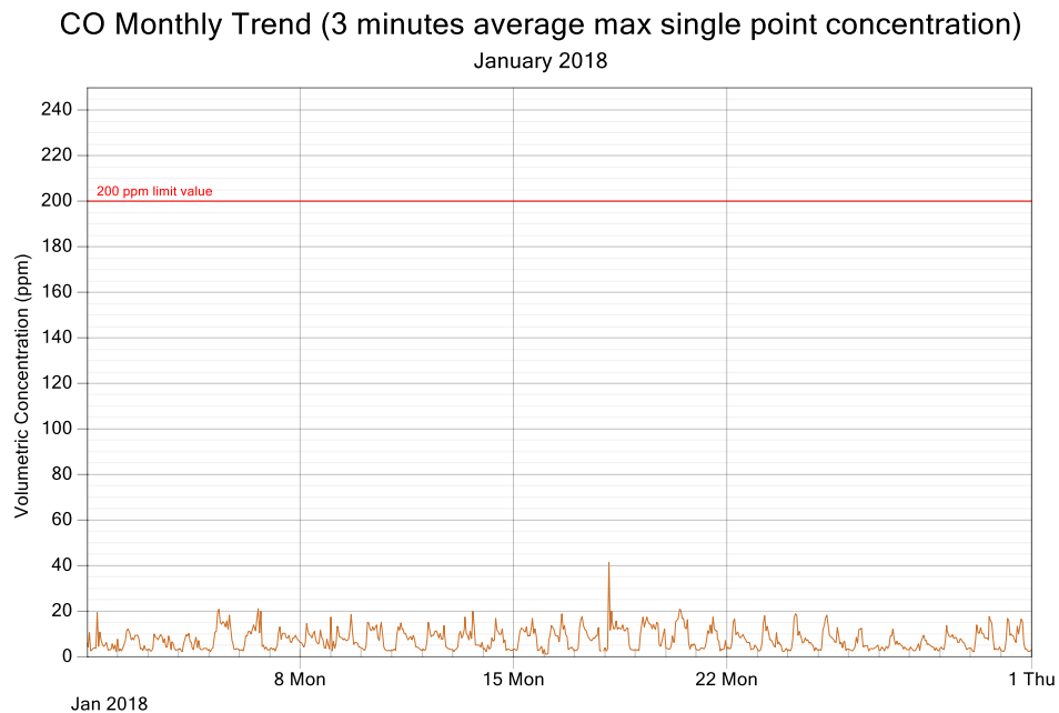
Figure 2: CO exposure and single point 3 minutes rolling averages for January 2018
