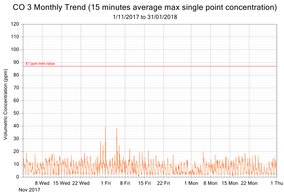
Figure 6: CO exposure and single point 15 minutes rolling averages from November 2017 to January 2018 (3 monthly trend)
