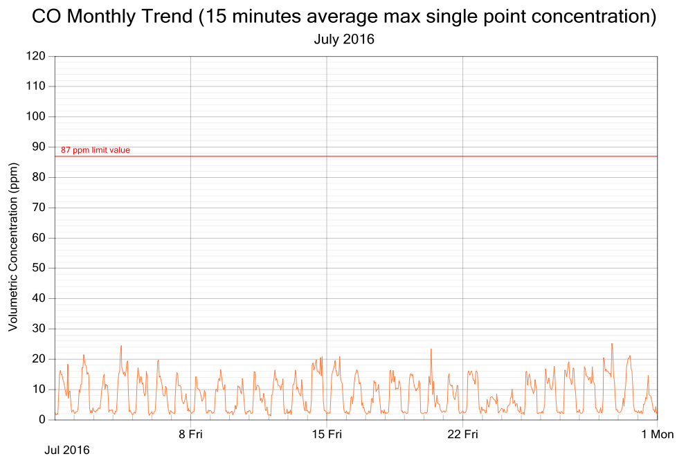
Figure 3: CO exposure and single point 15 minutes rolling averages for July 2016
