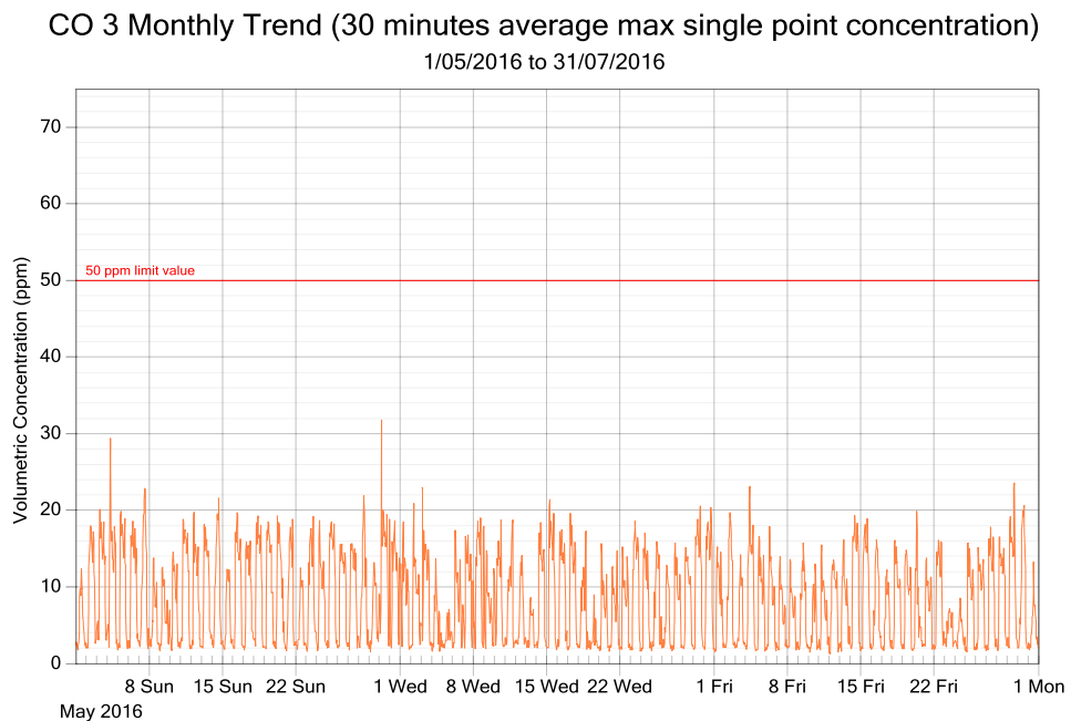
Figure 7: CO exposure and single point 30 minutes rolling averages from May 2016 to July 2016 (3 monthly trend)
