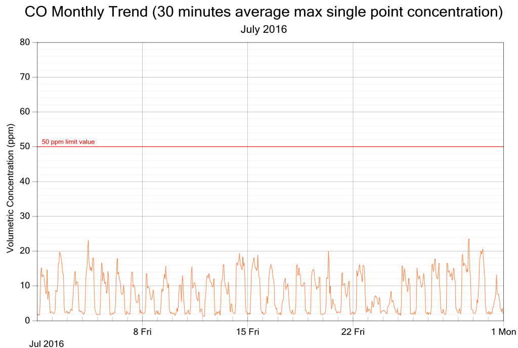
Figure 4: CO exposure and single point 30 minutes rolling averages for July 2016
