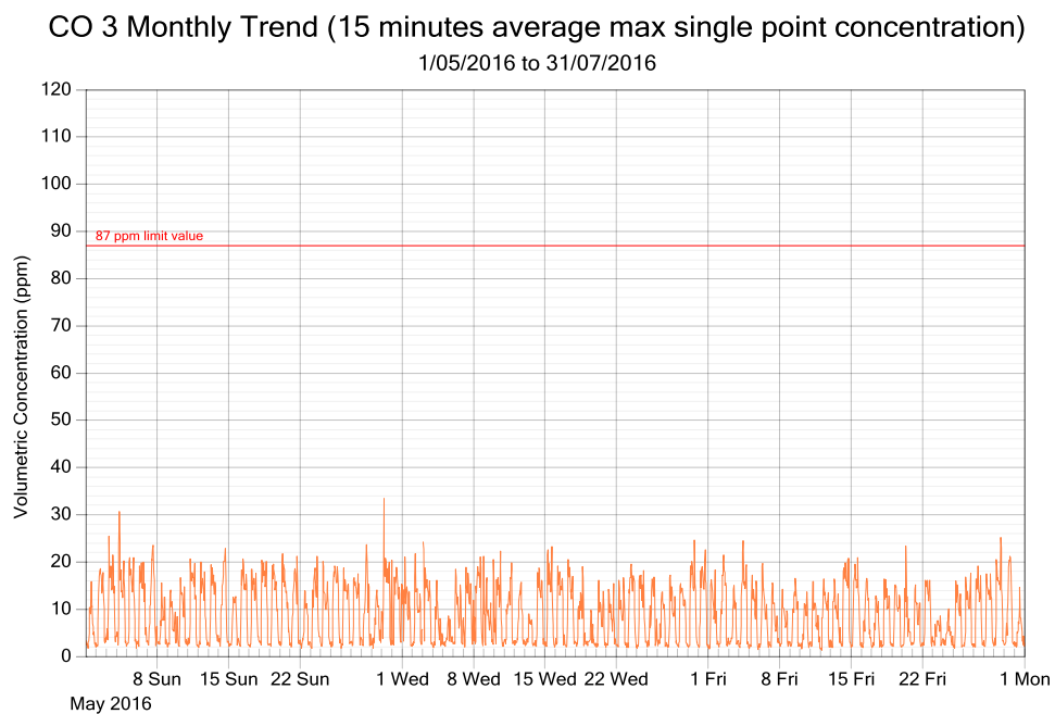
Figure 6: CO exposure and single point 15 minutes rolling averages from May 2016 to July 2016 (3 monthly trend)
