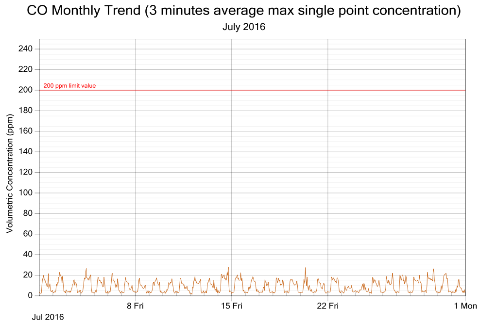
Figure 2: CO exposure and single point 3 minutes rolling averages for July 2016
