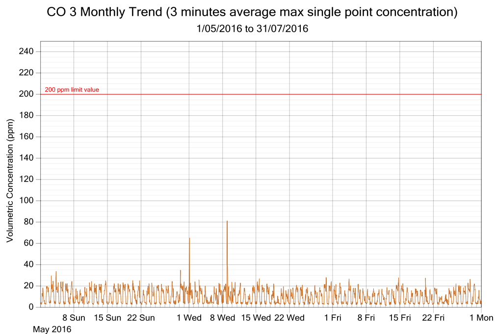
Figure 5: CO exposure and single point 3 minutes rolling averages from May 2016 to July 2016 (3 monthly trend)
