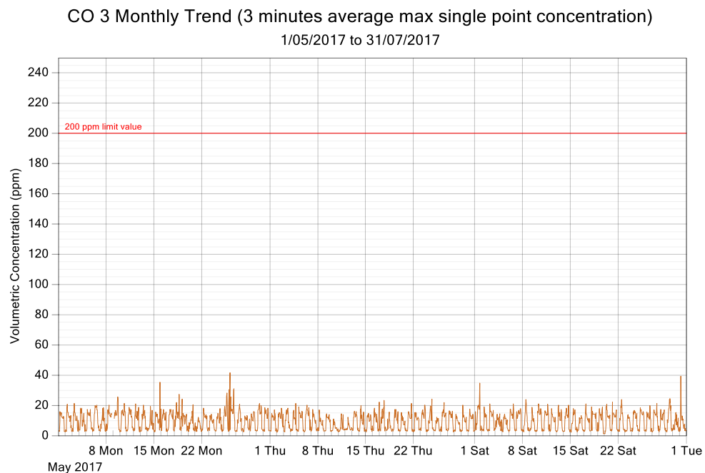
Figure 5: CO exposure and single point 3 minutes rolling averages from May 2017 to July 2017 (3 monthly trend)
