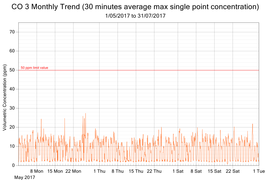
Figure 7: CO exposure and single point 30 minutes rolling averages from May 2017 to July 2017 (3 monthly trend)
