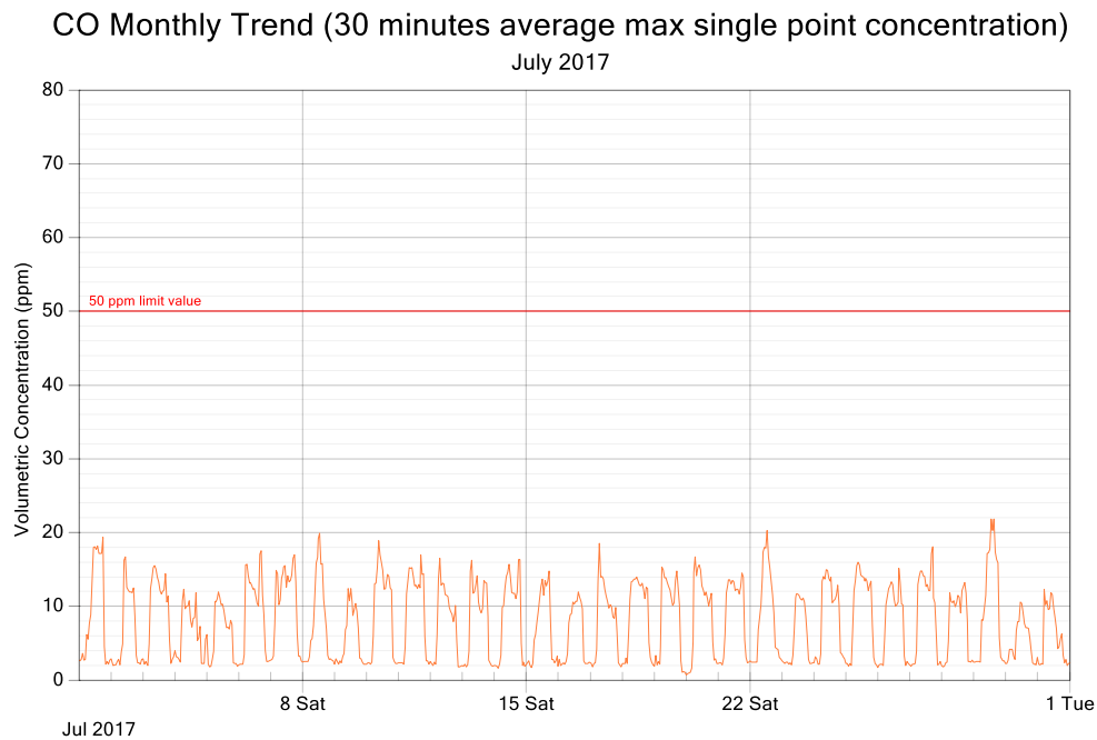
Figure 4: CO exposure and single point 30 minutes rolling averages for July 2017
