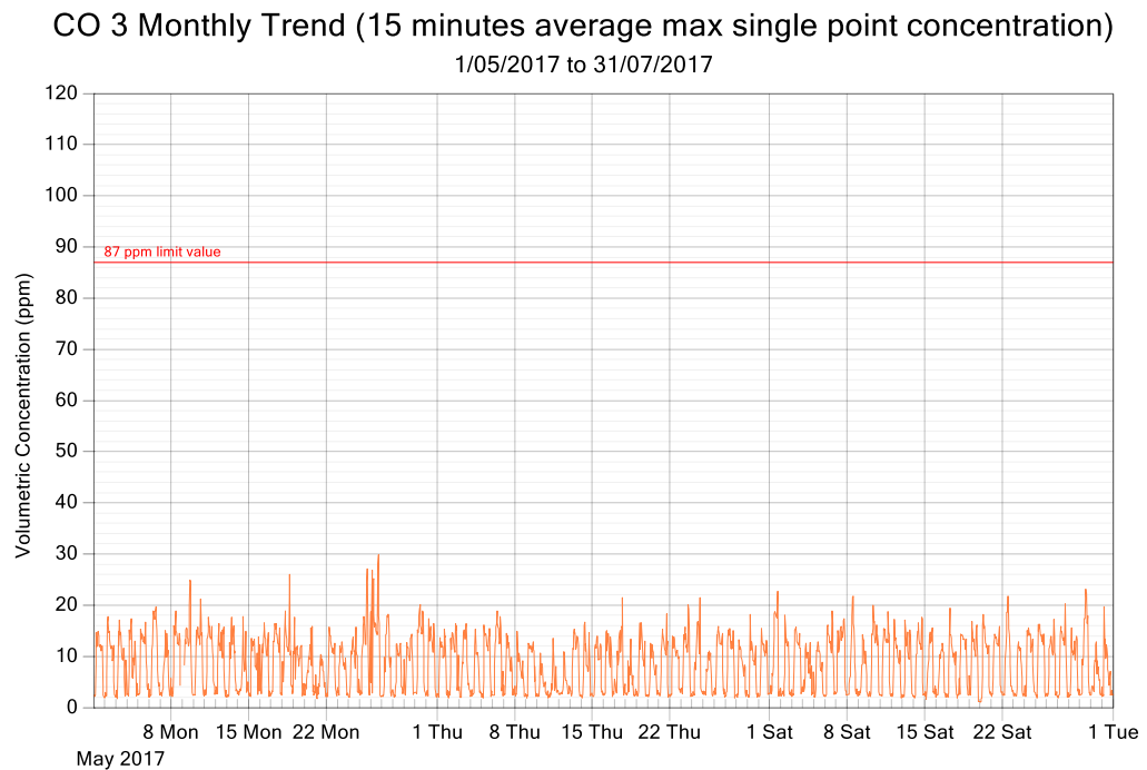
Figure 6: CO exposure and single point 15 minutes rolling averages from May 2017 to July 2017 (3 monthly trend)
