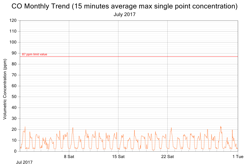
Figure 3: CO exposure and single point 15 minutes rolling averages for July 2017
