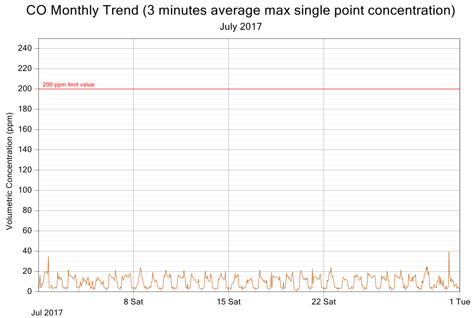
Figure 2: CO exposure and single point 3 minutes rolling averages for July 2017
