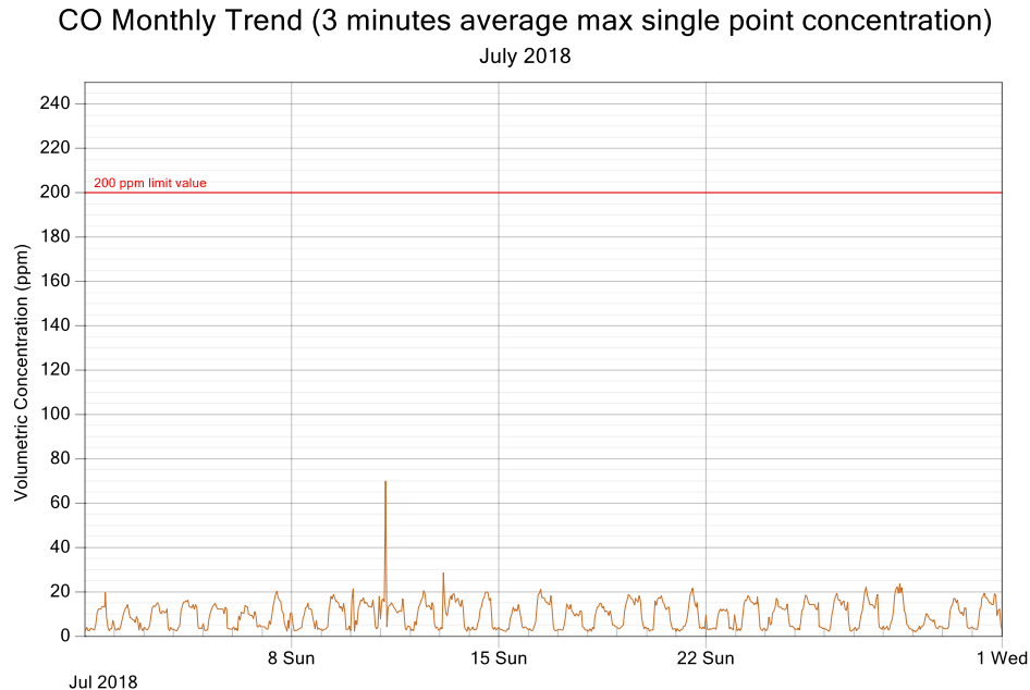
Figure 2: CO exposure and single point 3 minutes rolling averages for July 2018
