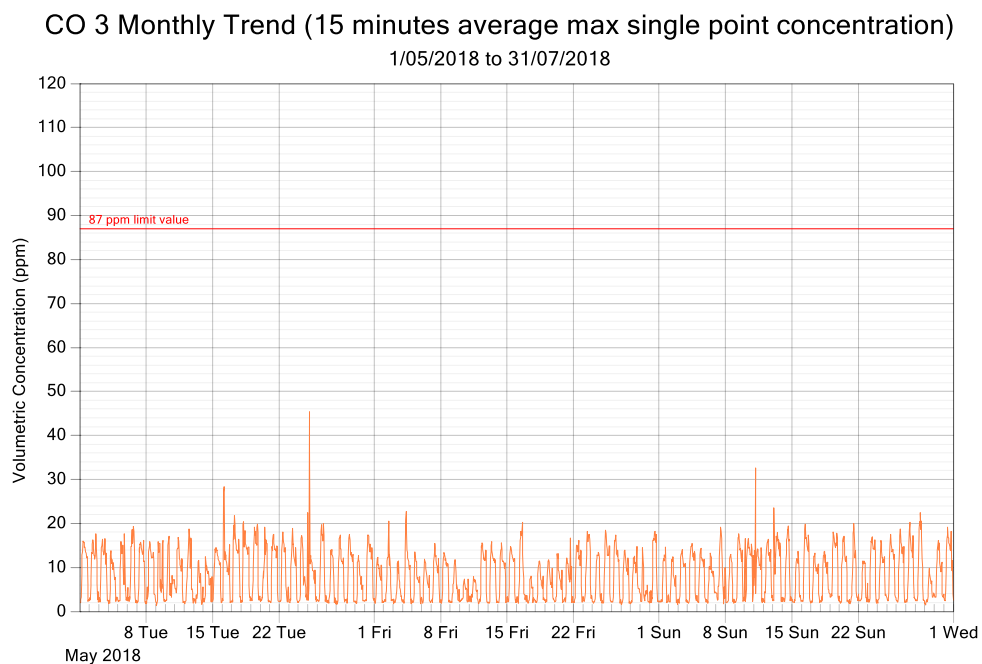
Figure 6: CO exposure and single point 15 minutes rolling averages from May 2018 to July 2018 (3 monthly trend)
