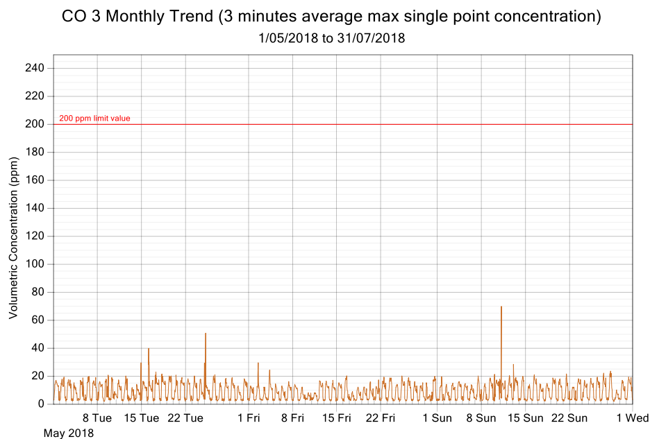
Figure 5: CO exposure and single point 3 minutes rolling averages from May 2018 to July 2018 (3 monthly trend)
