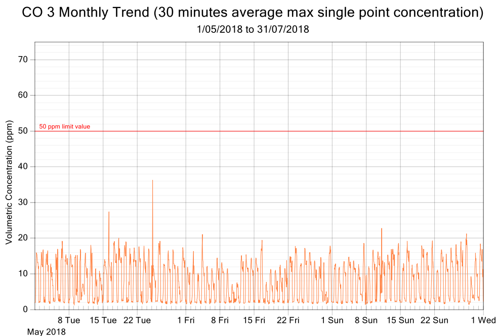
Figure 7: CO exposure and single point 30 minutes rolling averages from May 2018 to July 2018 (3 monthly trend)
