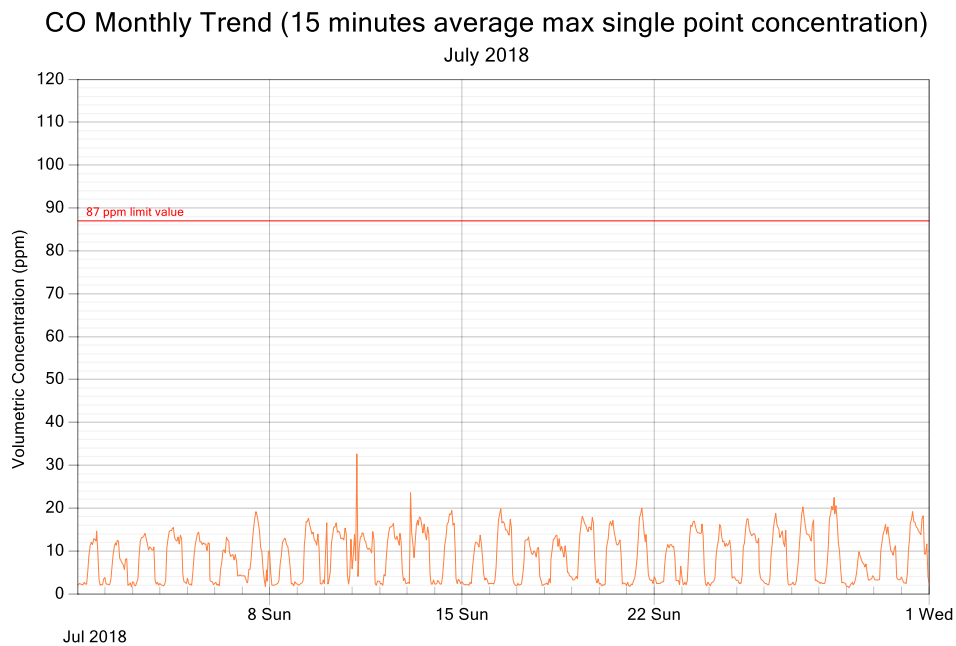
Figure 3: CO exposure and single point 15 minutes rolling averages for July 2018
