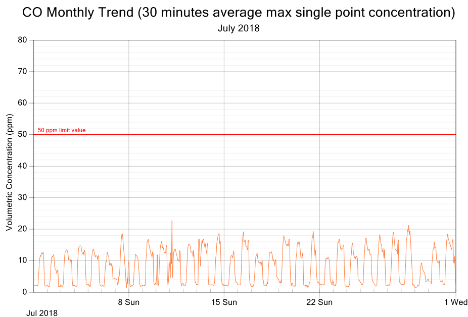
Figure 4: CO exposure and single point 30 minutes rolling averages for July 2018
