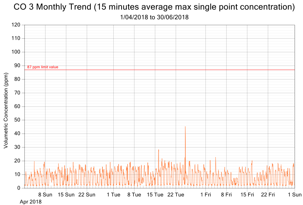
Figure 6: CO exposure and single point 15 minutes rolling averages from April 2018 to June 2018 (3 monthly trend)
