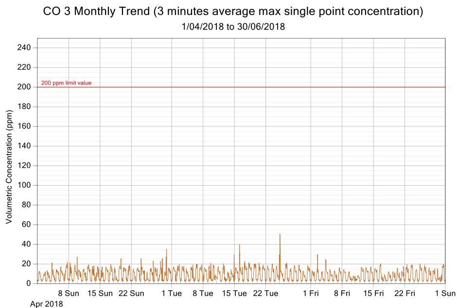
Figure 5: CO exposure and single point 3 minutes rolling averages from April 2018 to June 2018 (3 monthly trend)
