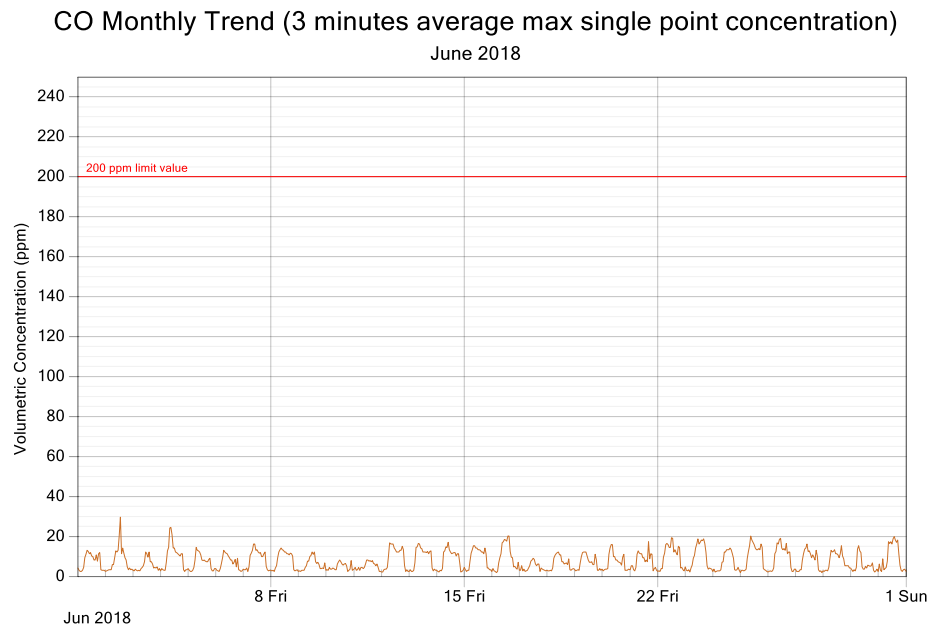
Figure 2: CO exposure and single point 3 minutes rolling averages for June 2018
