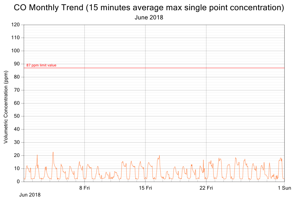
Figure 3: CO exposure and single point 15 minutes rolling averages for June 2018
