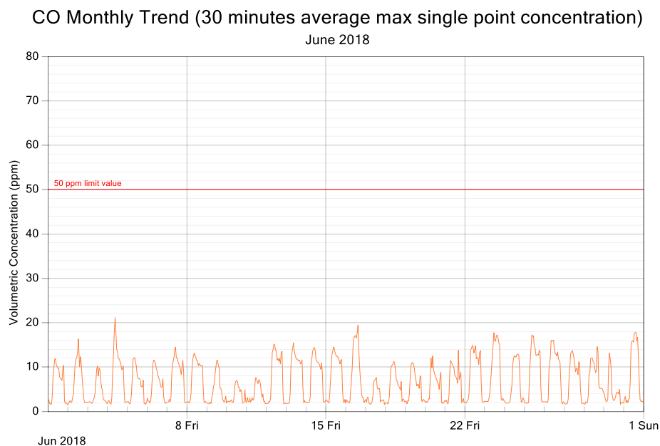
Figure 4: CO exposure and single point 30 minutes rolling averages for June 2018
