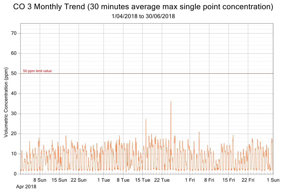
Figure 7: CO exposure and single point 30 minutes rolling averages from April 2018 to June 2018 (3 monthly trend)
