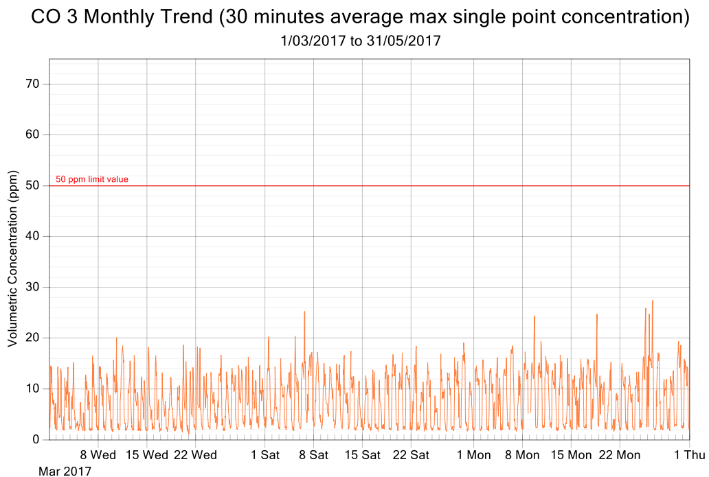
Figure 7: CO exposure and single point 30 minutes rolling averages from March 2017 to May 2017 (3 monthly trend)
