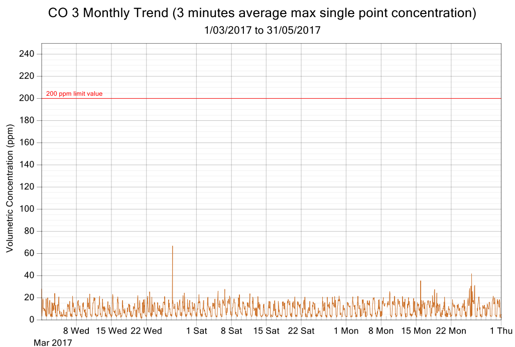
Figure 5: CO exposure and single point 3 minutes rolling averages from March 2017 to May 2017 (3 monthly trend)
