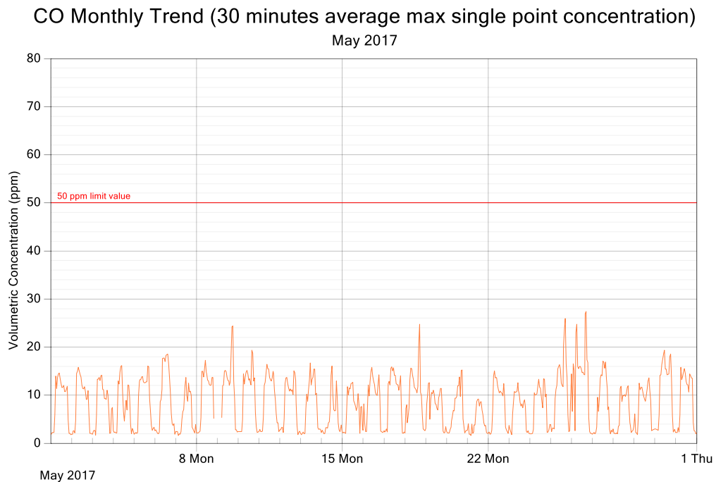
Figure 4: CO exposure and single point 30 minutes rolling averages for May 2017
