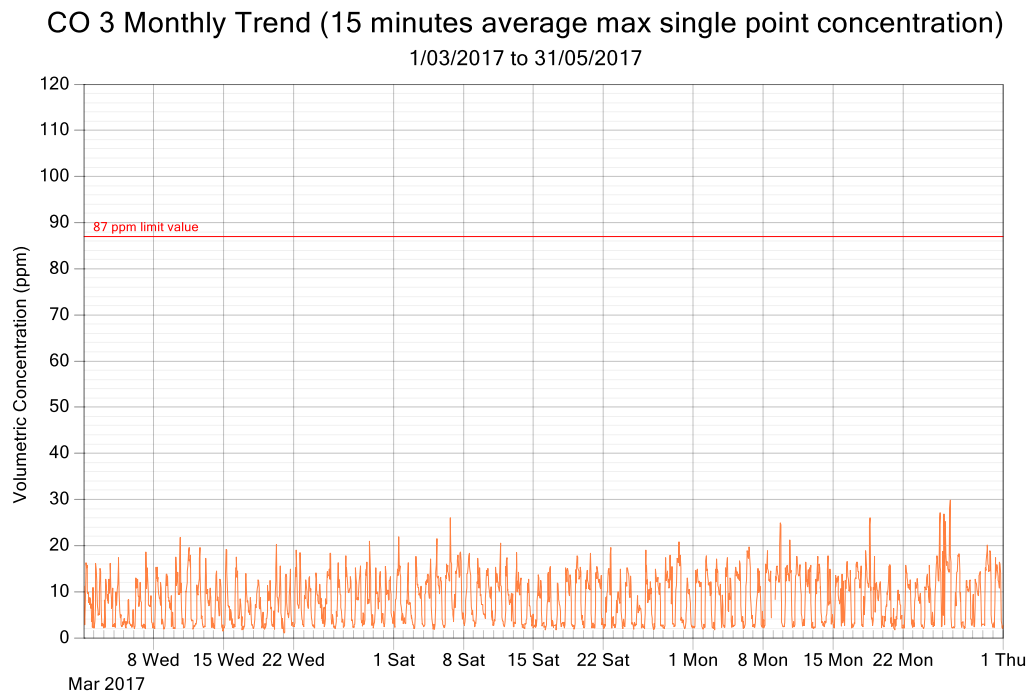
Figure 6: CO exposure and single point 15 minutes rolling averages from March 2017 to May 2017 (3 monthly trend)
