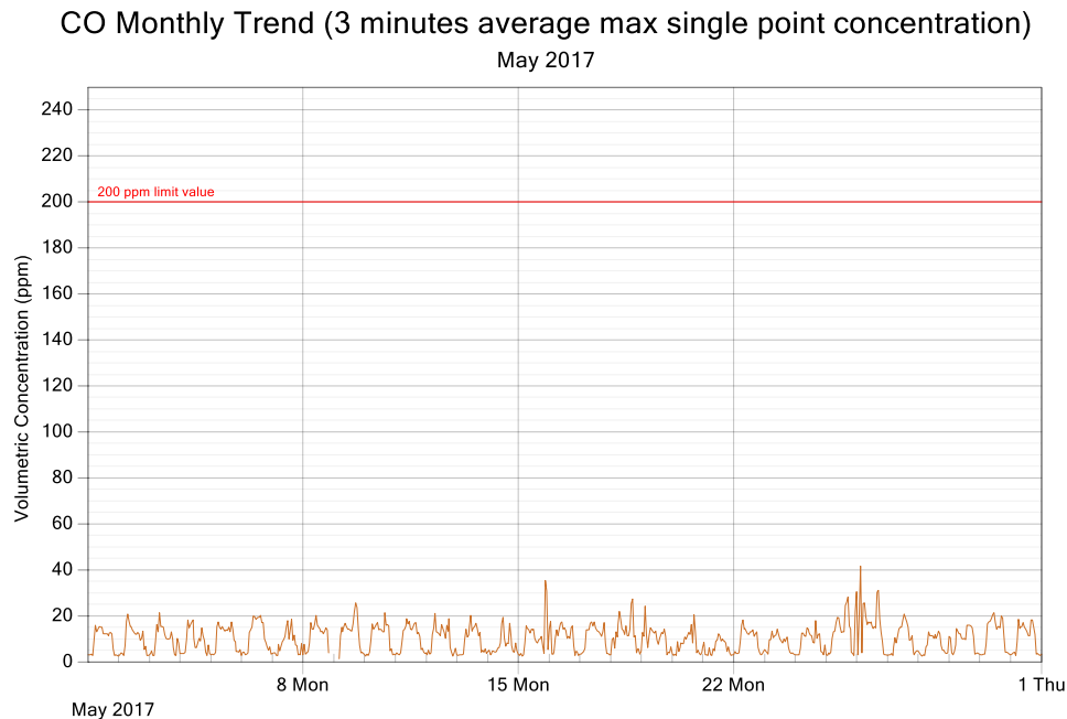
Figure 2: CO exposure and single point 3 minutes rolling averages for May 2017
