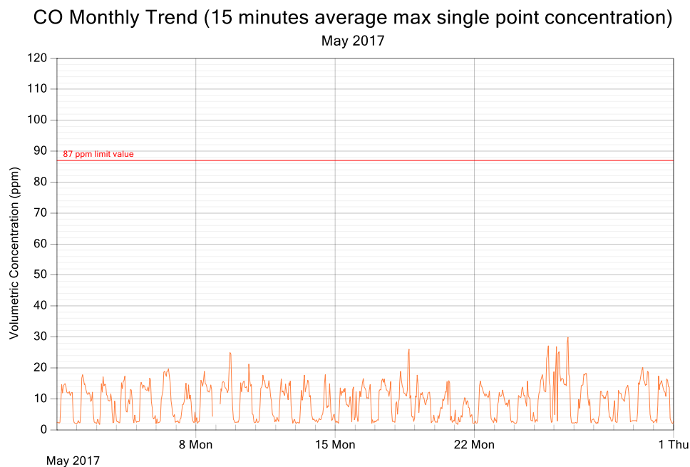
Figure 3: CO exposure and single point 15 minutes rolling averages for May 2017
