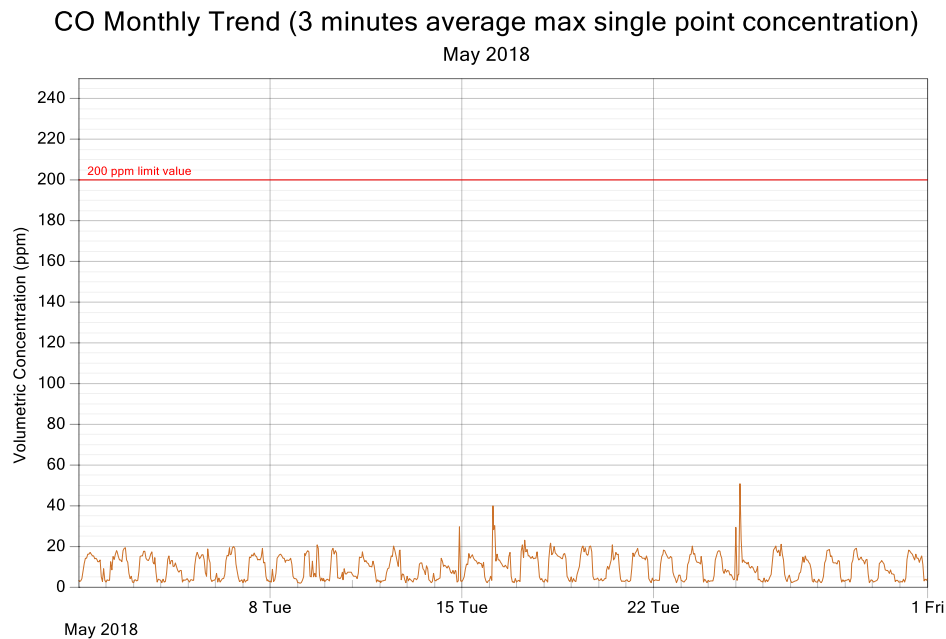
Figure 2: CO exposure and single point 3 minutes rolling averages for May 2018
