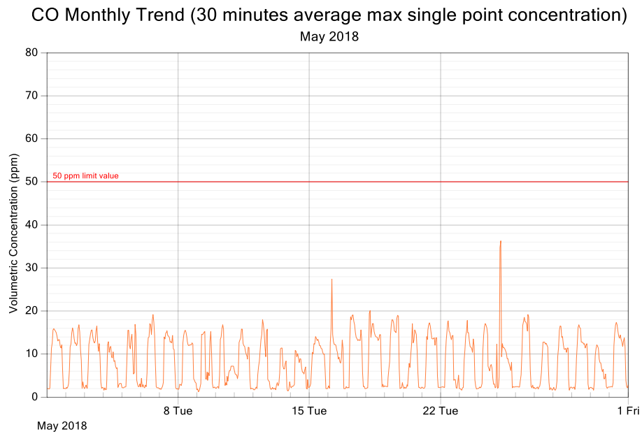
Figure 4: CO exposure and single point 30 minutes rolling averages for May 2018
