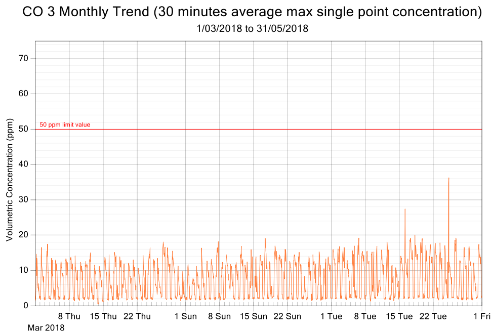
Figure 7: CO exposure and single point 30 minutes rolling averages from March 2018 to May 2018 (3 monthly trend)
