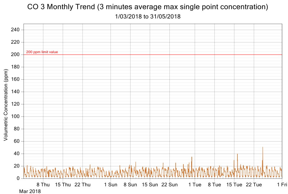
Figure 5: CO exposure and single point 3 minutes rolling averages from March 2018 to May 2018 (3 monthly trend)
