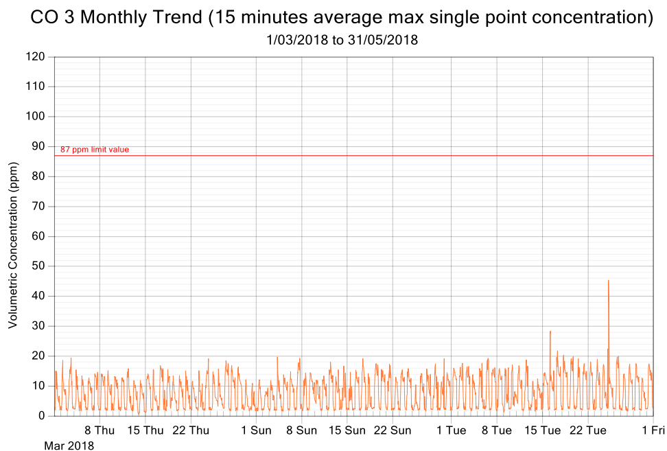
Figure 6: CO exposure and single point 15 minutes rolling averages from March 2018 to May 2018 (3 monthly trend)
