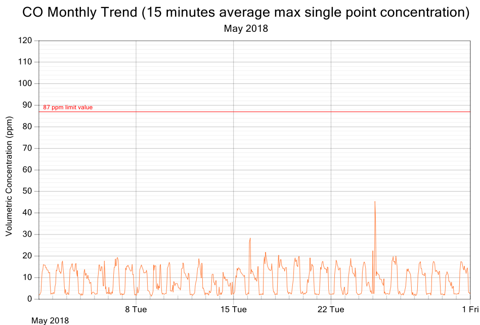
Figure 3: CO exposure and single point 15 minutes rolling averages for May 2018
