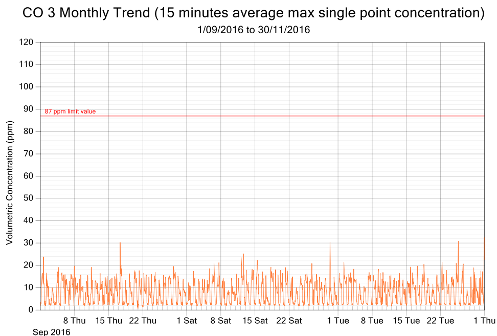
Figure 6: CO exposure and single point 15 minutes rolling averages from September 2016 to November 2016 (3 monthly trend)
