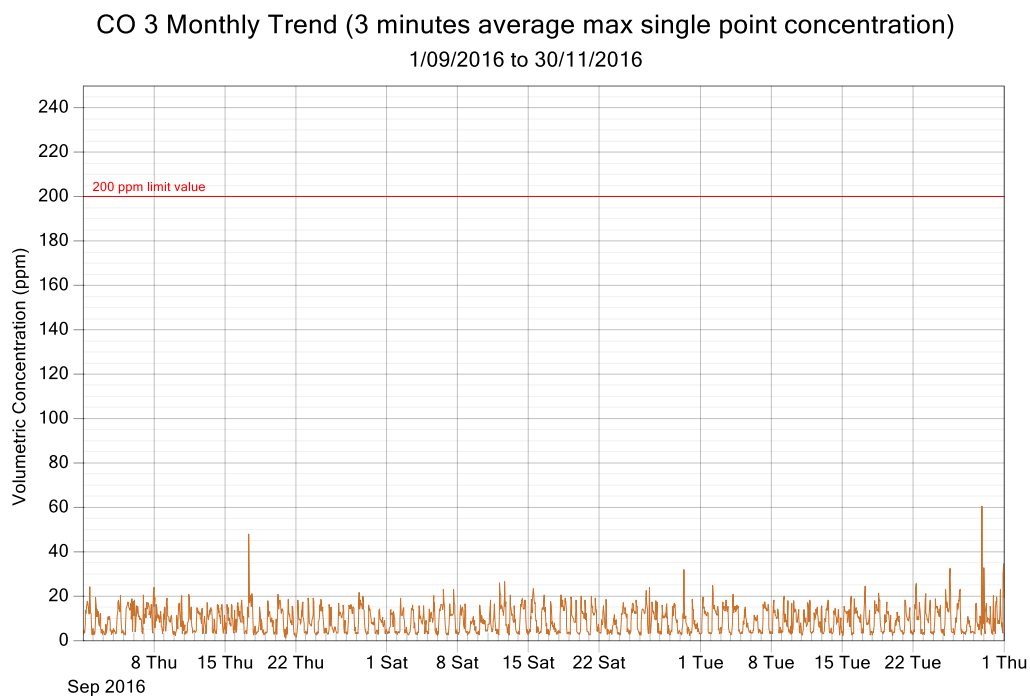
Figure 5: CO exposure and single point 3 minutes rolling averages from September 2016 to November 2016 (3 monthly trend)
