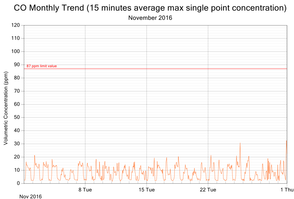
Figure 3: CO exposure and single point 15 minutes rolling averages for November 2016
