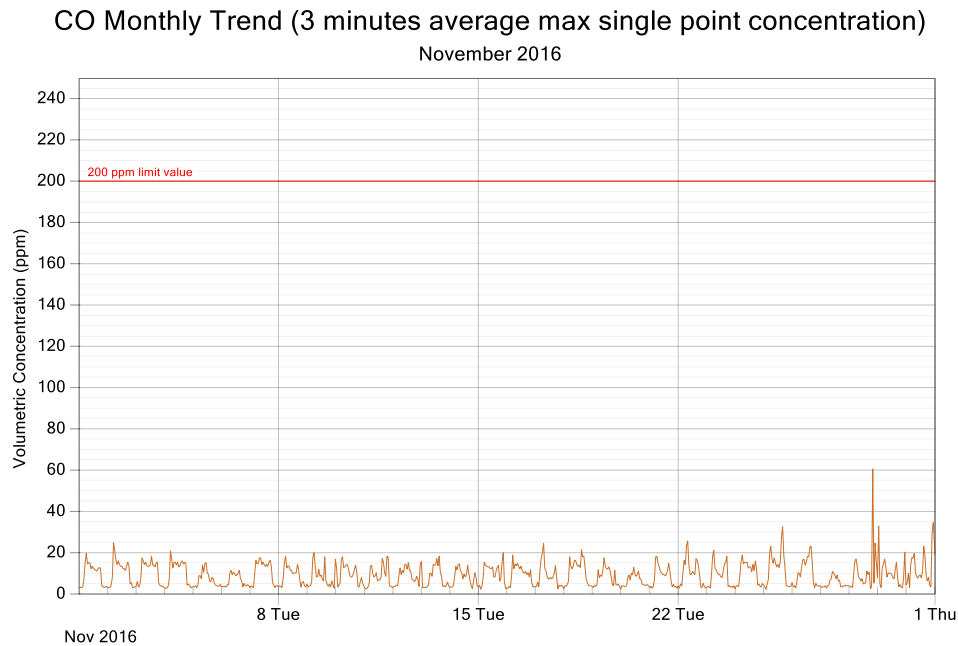
Figure 2: CO exposure and single point 3 minutes rolling averages for November 2016
