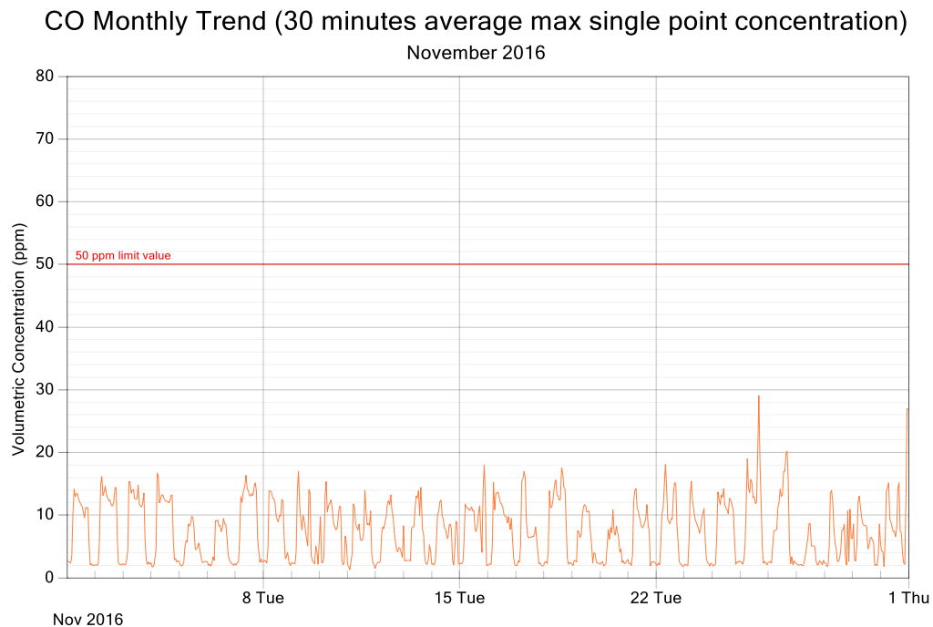
Figure 4: CO exposure and single point 30 minutes rolling averages for November 2016
