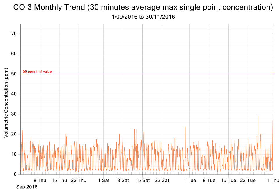
Figure 7: CO exposure and single point 30 minutes rolling averages from September 2016 to November 2016 (3 monthly trend)
