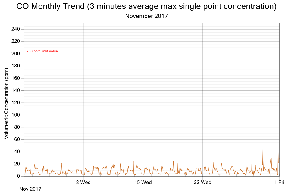
Figure 2: CO exposure and single point 3 minutes rolling averages for November 2017
