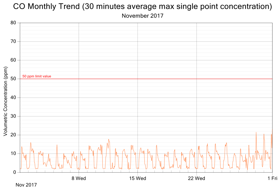
Figure 4: CO exposure and single point 30 minutes rolling averages for November 2017
