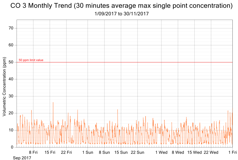
Figure 7: CO exposure and single point 30 minutes rolling averages from September 2017 to November 2017 (3 monthly trend)
