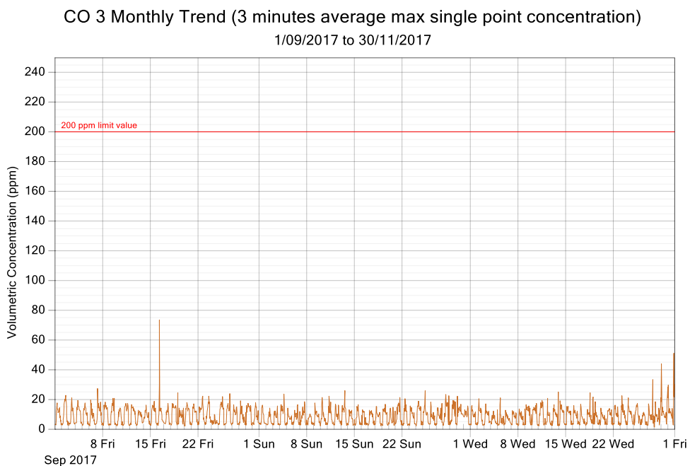
Figure 5: CO exposure and single point 3 minutes rolling averages from September 2017 to November 2017 (3 monthly trend)
