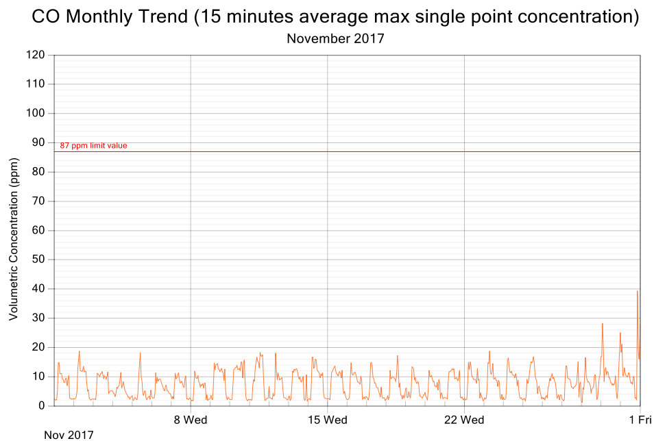
Figure 3: CO exposure and single point 15 minutes rolling averages for November 2017
