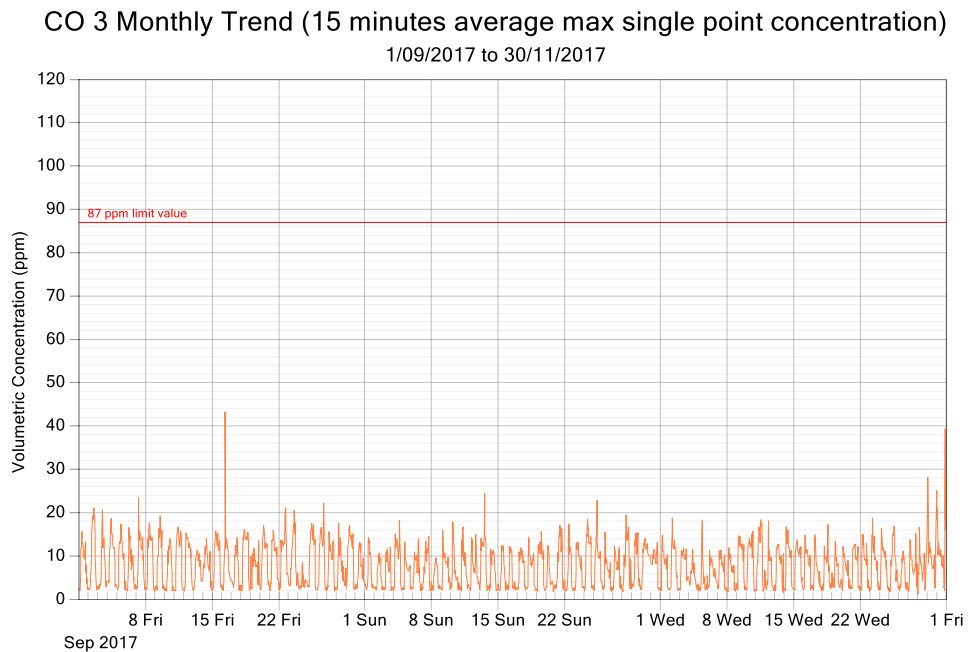
Figure 6: CO exposure and single point 15 minutes rolling averages from September 2017 to November 2017 (3 monthly trend)
