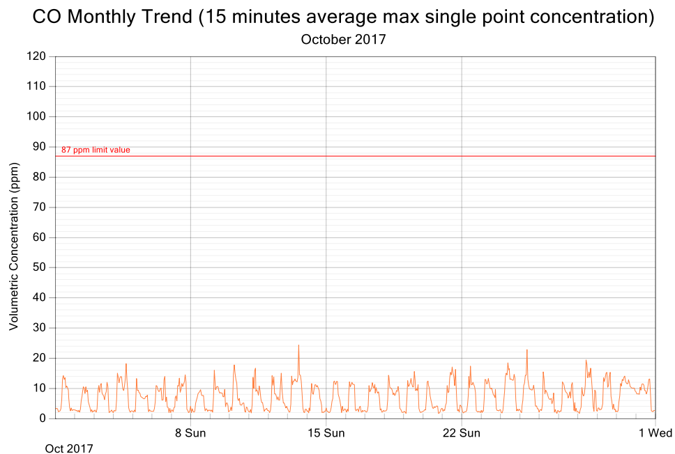
Figure 3: CO exposure and single point 15 minutes rolling averages for October 2017
