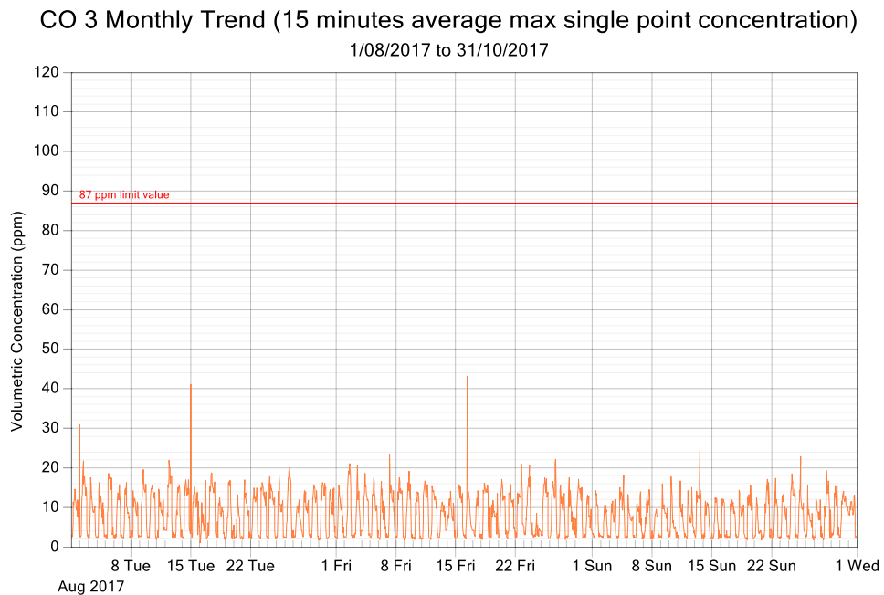
Figure 6: CO exposure and single point 15 minutes rolling averages from August 2017 to October 2017 (3 monthly trend)
