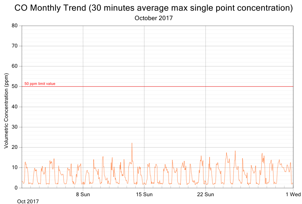
Figure 4: CO exposure and single point 30 minutes rolling averages for October 2017
