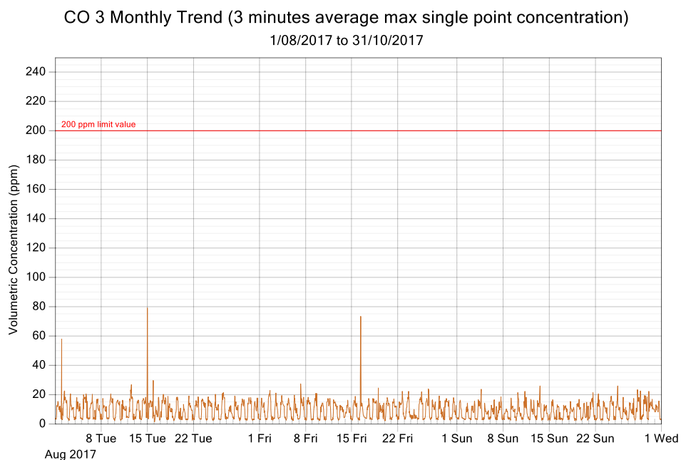
Figure 5: CO exposure and single point 3 minutes rolling averages from August 2017 to October 2017 (3 monthly trend)
