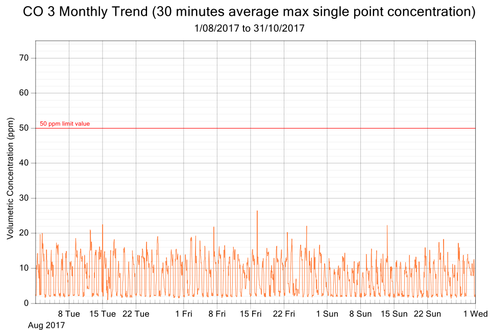
Figure 7: CO exposure and single point 30 minutes rolling averages from August 2017 to October 2017 (3 monthly trend)
