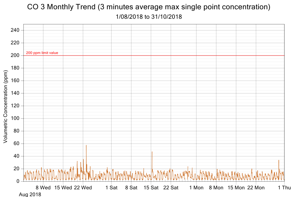
Figure 5: CO exposure and single point 3 minutes rolling averages from August 2018 to October 2018 (3 monthly trend)
