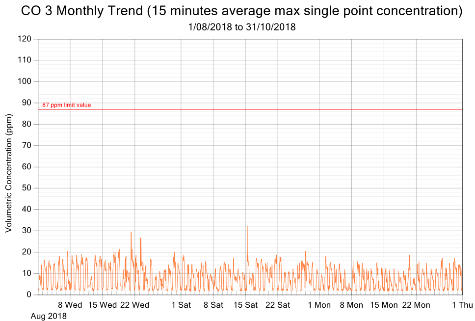
Figure 6: CO exposure and single point 15 minutes rolling averages from August 2018 to October 2018 (3 monthly trend)
