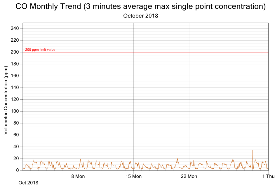
Figure 2: CO exposure and single point 3 minutes rolling averages for October 2018
