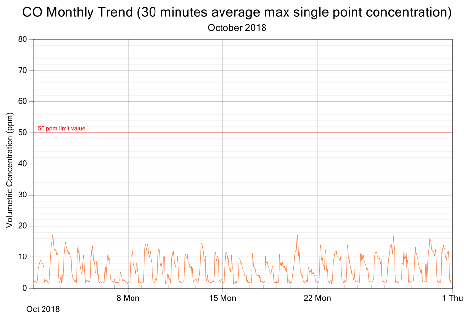
Figure 4: CO exposure and single point 30 minutes rolling averages for October 2018
