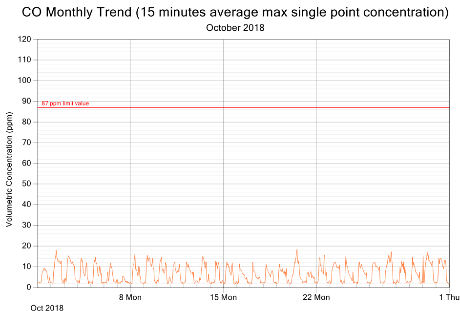
Figure 3: CO exposure and single point 15 minutes rolling averages for October 2018
