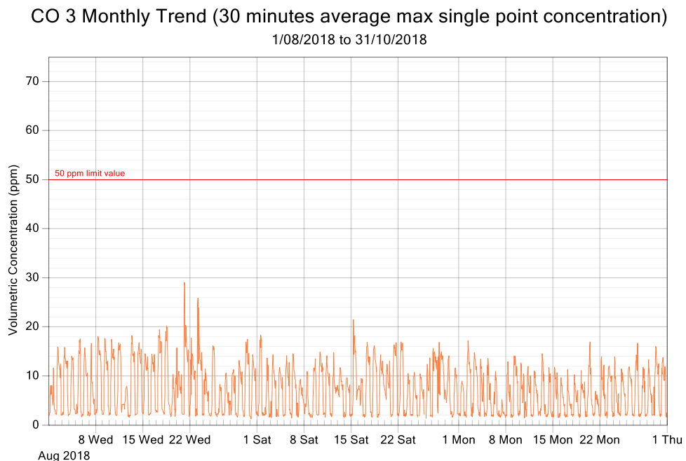
Figure 7: CO exposure and single point 30 minutes rolling averages from August 2018 to October 2018 (3 monthly trend)
