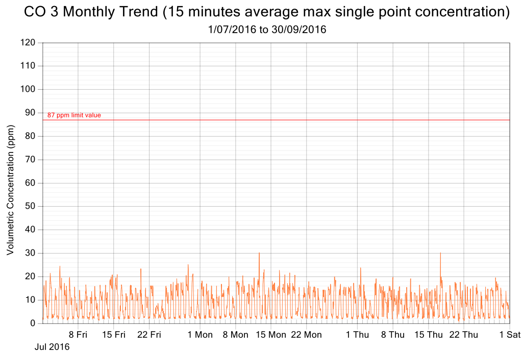
Figure 6: CO exposure and single point 15 minutes rolling averages from July 2016 to September 2016 (3 monthly trend)
