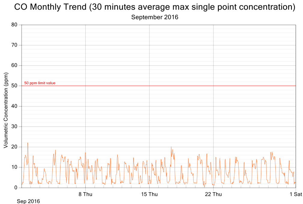
Figure 4: CO exposure and single point 30 minutes rolling averages for September 2016
