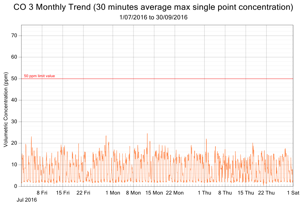
Figure 7: CO exposure and single point 30 minutes rolling averages from July 2016 to September 2016 (3 monthly trend)
