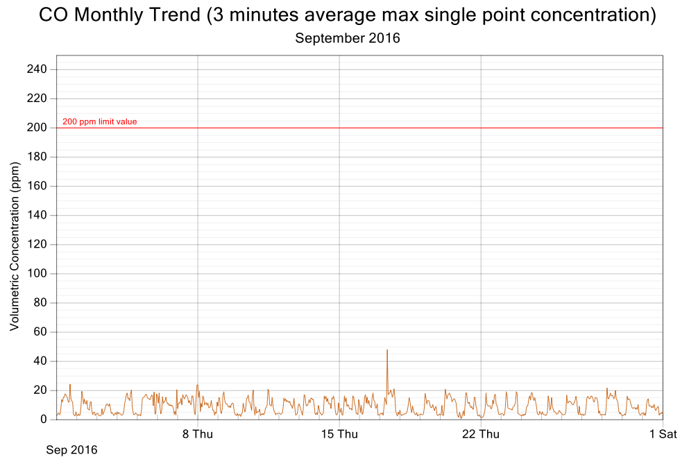
Figure 2: CO exposure and single point 3 minutes rolling averages for September 2016
