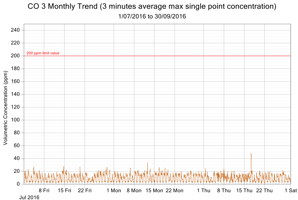
Figure 5: CO exposure and single point 3 minutes rolling averages from July 2016 to September 2016 (3 monthly trend)
