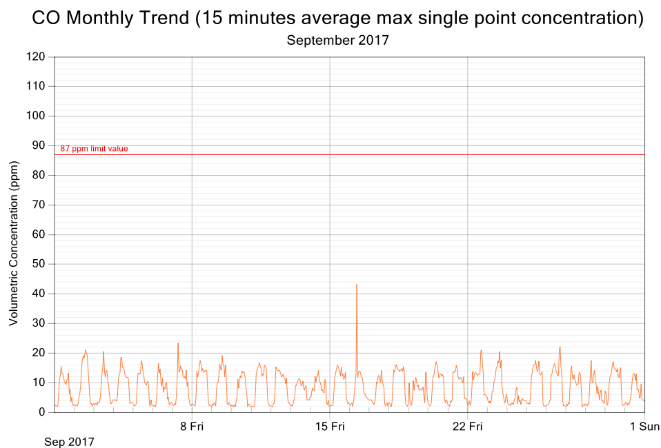
Figure 3: CO exposure and single point 15 minutes rolling averages for September 2017
