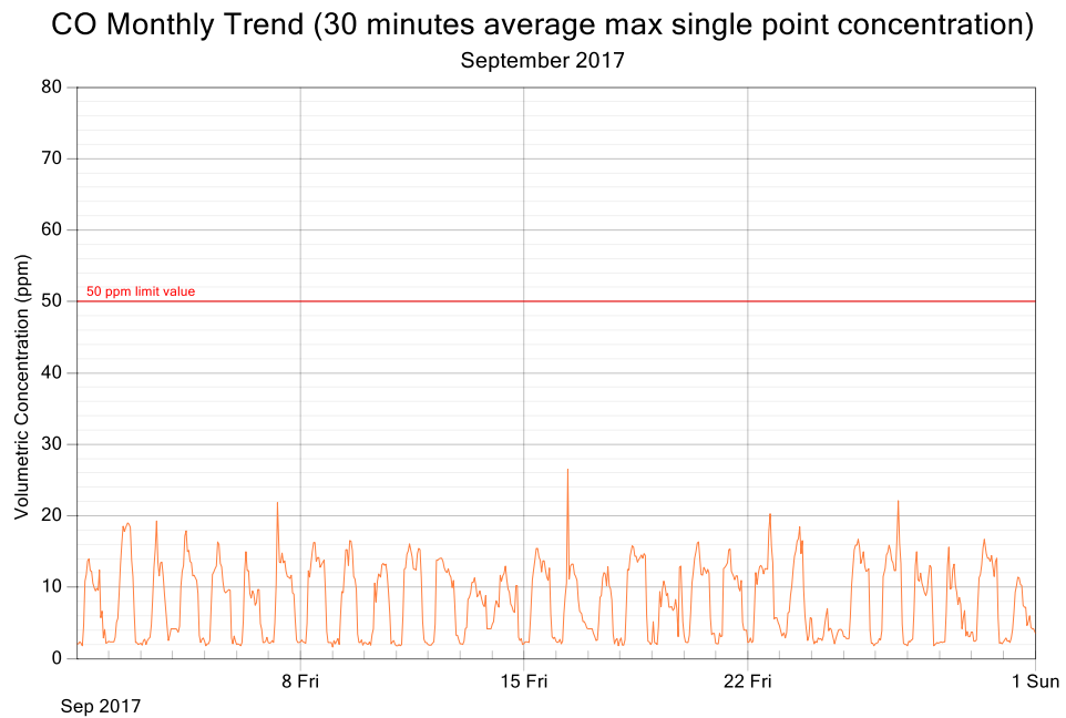
Figure 4: CO exposure and single point 30 minutes rolling averages for September 2017
