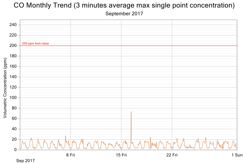
Figure 2: CO exposure and single point 3 minutes rolling averages for September 2017
