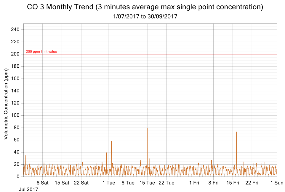
Figure 5: CO exposure and single point 3 minutes rolling averages from July 2017 to September 2017 (3 monthly trend)
