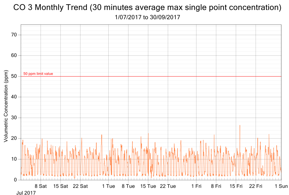
Figure 7: CO exposure and single point 30 minutes rolling averages from July 2017 to September 2017 (3 monthly trend)
