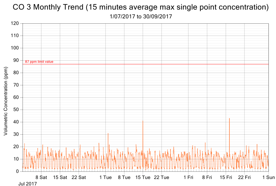
Figure 6: CO exposure and single point 15 minutes rolling averages from July 2017 to September 2017 (3 monthly trend)
