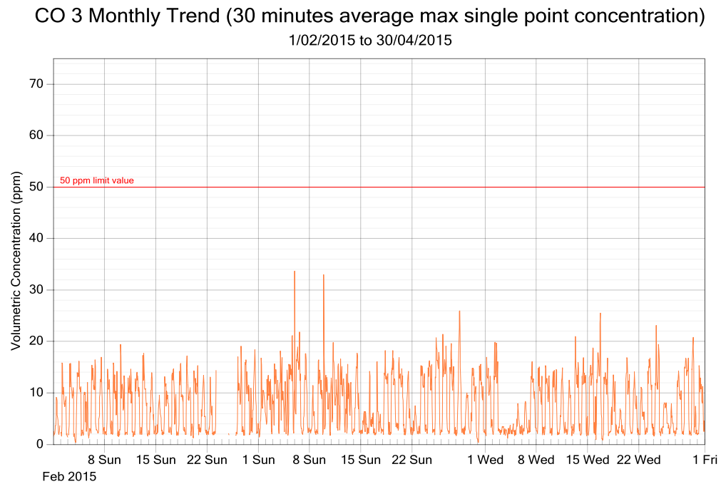
Figure 7: CO exposure and single point 30 minutes rolling averages from February 2015 to April 2015 (3 monthly trend)
