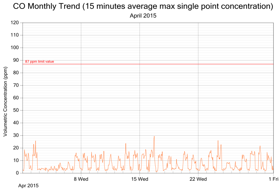
Figure 3: CO exposure and single point 15 minutes rolling averages for April 2015
