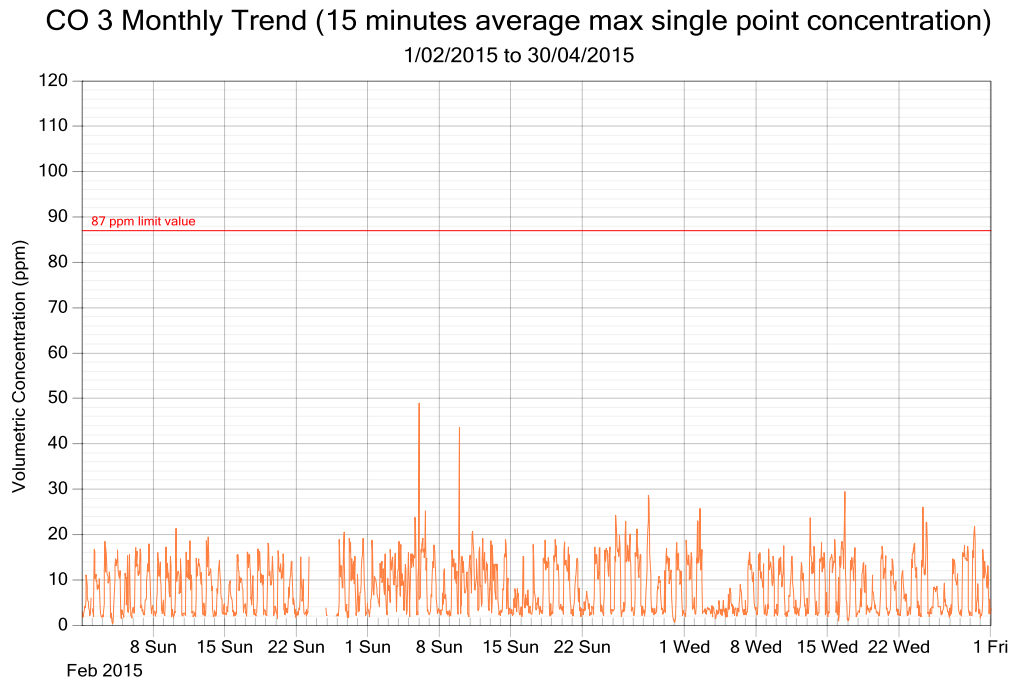
Figure 6: CO exposure and single point 15 minutes rolling averages from February 2015 to April 2015 (3 monthly trend)
