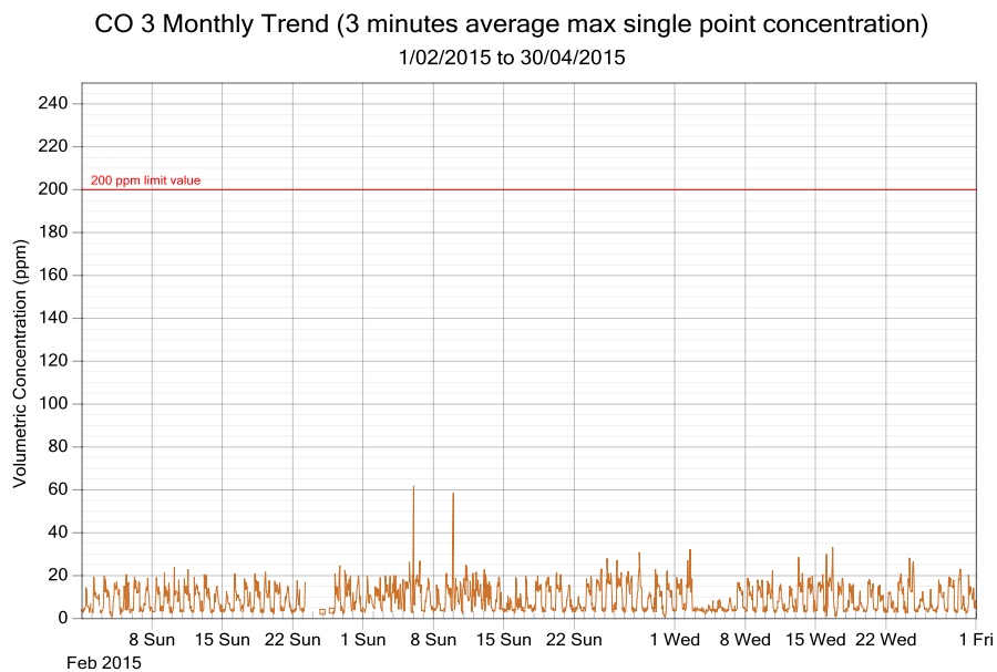
Figure 5: CO exposure and single point 3 minutes rolling averages from February 2015 to April 2015 (3 monthly trend)
