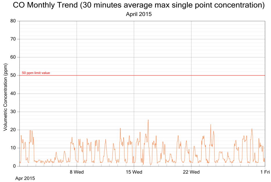
Figure 4: CO exposure and single point 30 minutes rolling averages for April 2015
