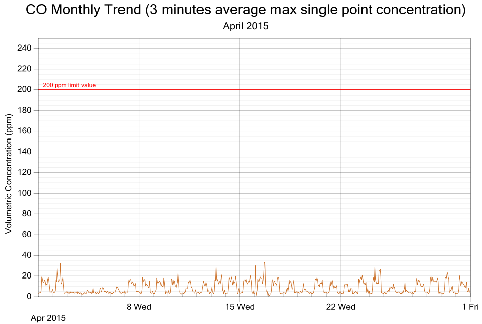
Figure 2: CO exposure and single point 3 minutes rolling averages for April 2015
