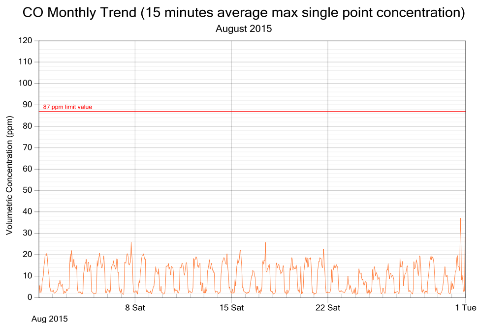
Figure 3: CO exposure and single point 15 minutes rolling averages for August 2015
