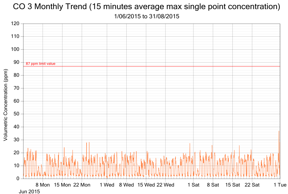
Figure 6: CO exposure and single point 15 minutes rolling averages from May 2015 to August 2015 (3 monthly trend)
