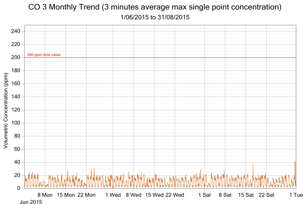
Figure 5: CO exposure and single point 3 minutes rolling averages from May 2015 to August 2015 (3 monthly trend)
