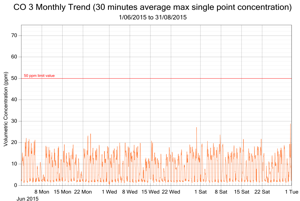
Figure 7: CO exposure and single point 30 minutes rolling averages from May 2015 to August 2015 (3 monthly trend)
