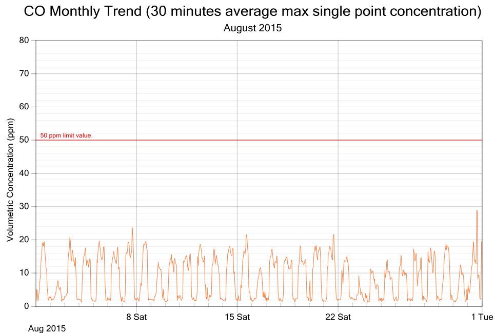
Figure 4: CO exposure and single point 30 minutes rolling averages for August 2015
