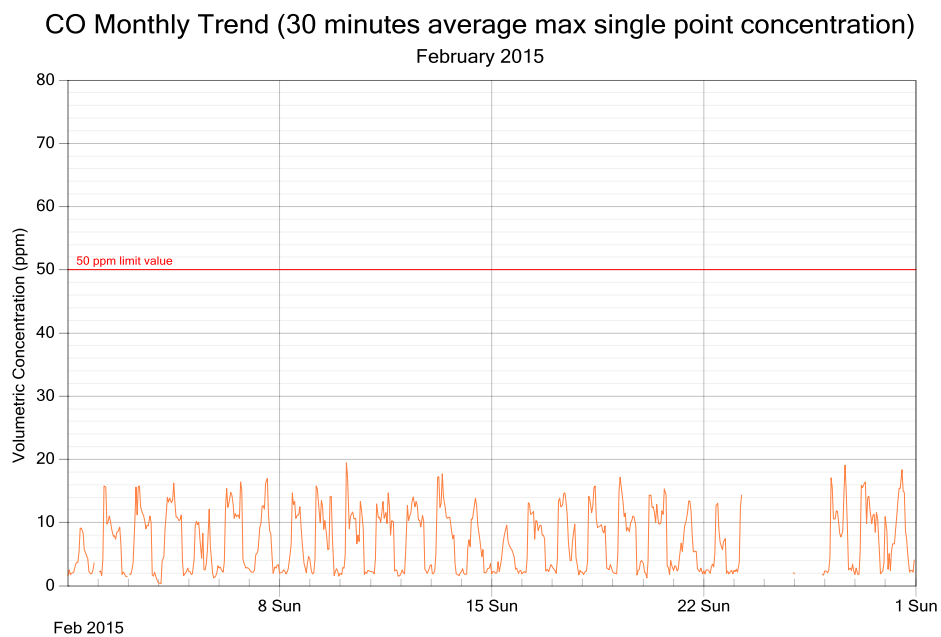
Figure 4: CO exposure and single point 30 minutes rolling averages for February 2015
