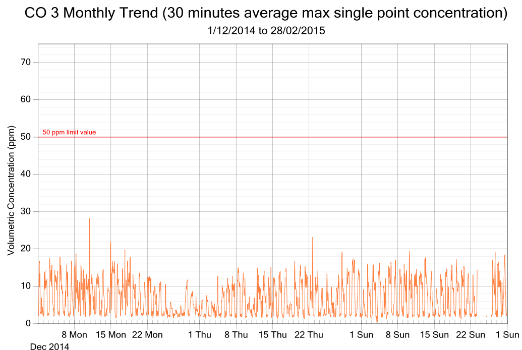
Figure 7: CO exposure and single point 30 minutes rolling averages from December 2015 to February 2015 (3 monthly trend)
