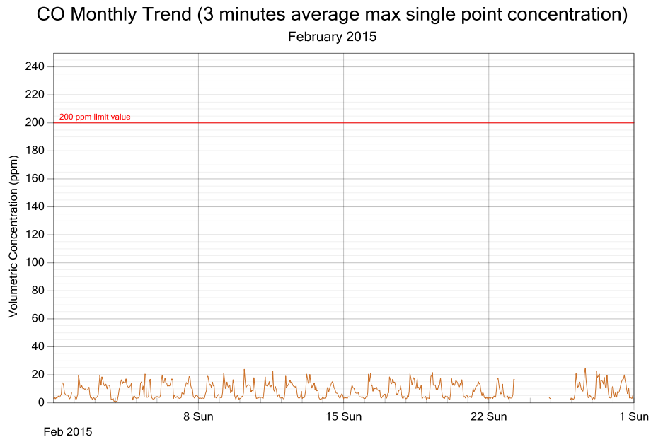
Figure 2: CO exposure and single point 3 minutes rolling averages for February 2015
