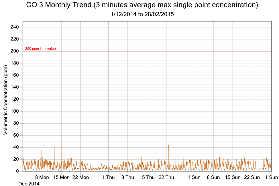
Figure 5: CO exposure and single point 3 minutes rolling averages from December 2014 to February 2015 (3 monthly trend)
