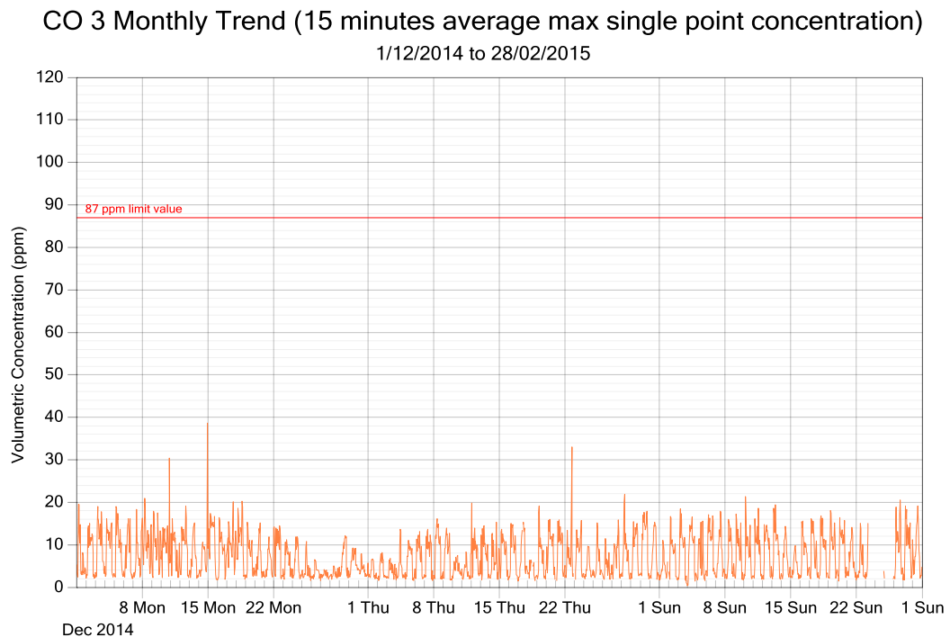
Figure 6: CO exposure and single point 15 minutes rolling averages from December 2014 to February 2015 (3 monthly trend)
