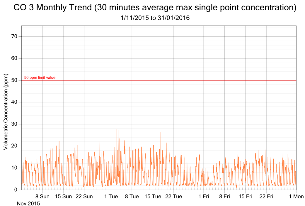
Figure 7: CO exposure and single point 30 minutes rolling averages from November 2015 to January 2016 (3 monthly trend)
