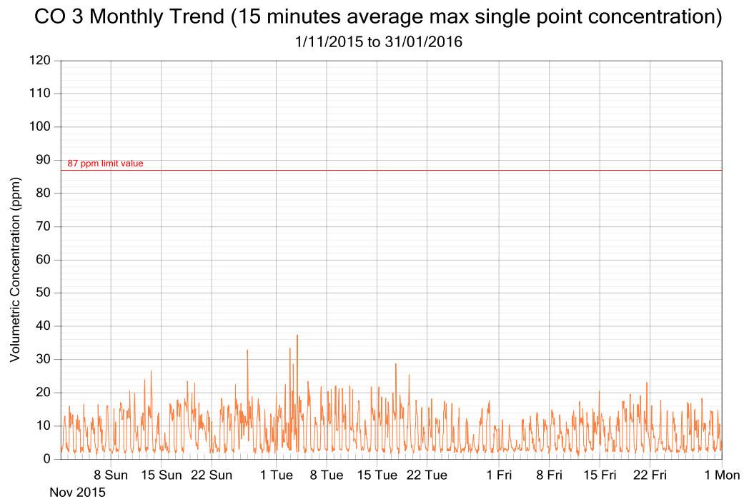
Figure 6: CO exposure and single point 15 minutes rolling averages from November 2015 to January 2016 (3 monthly trend)
