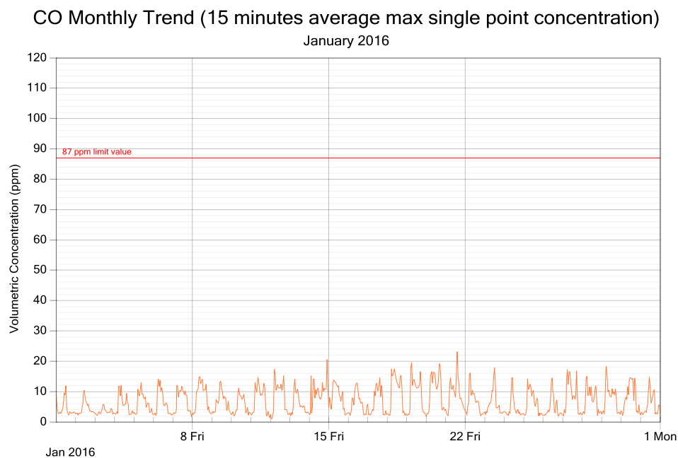
Figure 3: CO exposure and single point 15 minutes rolling averages for January 2016
