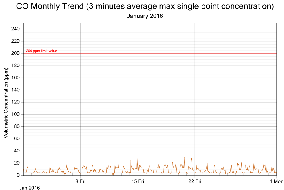
Figure 2: CO exposure and single point 3 minutes rolling averages for January 2016
