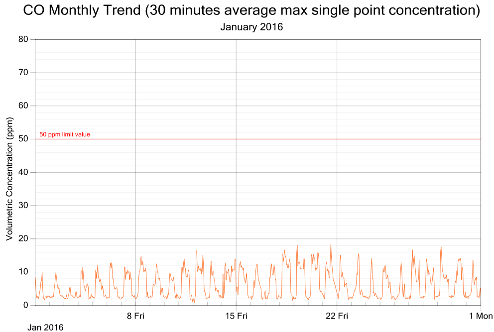
Figure 4: CO exposure and single point 30 minutes rolling averages for January 2016
