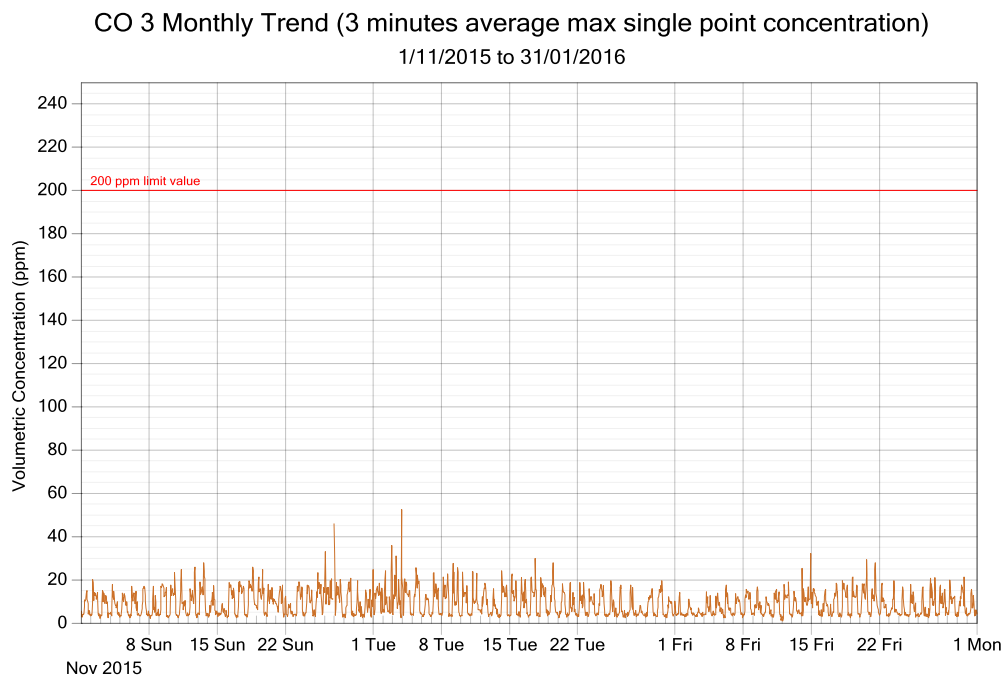
Figure 5: CO exposure and single point 3 minutes rolling averages from November 2015 to January 2016 (3 monthly trend)
