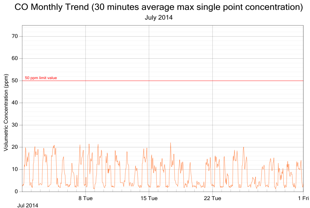
Figure 4: CO exposure and single point 30 minutes rolling averages for July 2014
