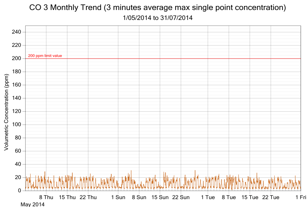
Figure 5: CO exposure and single point 3 minutes rolling averages from May to July 2014 (3 monthly trend)
