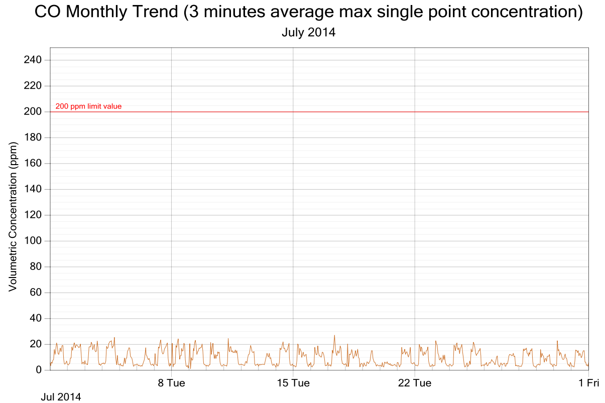
Figure 2: CO exposure and single point 3 minutes rolling averages for July 2014
