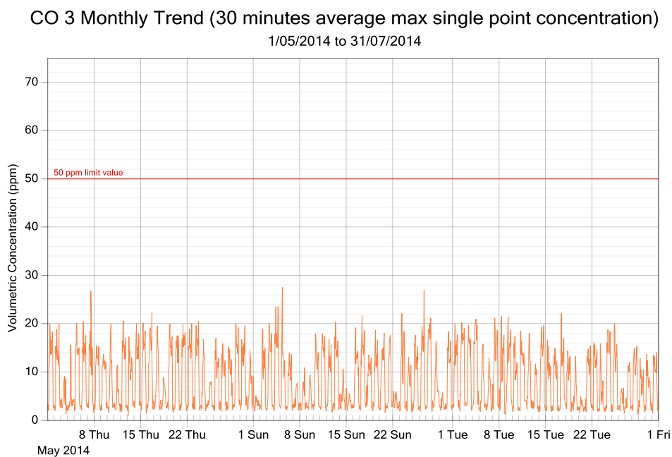
Figure 7: CO exposure and single point 30 minutes rolling averages from May to July 2014 (3 monthly trend)
