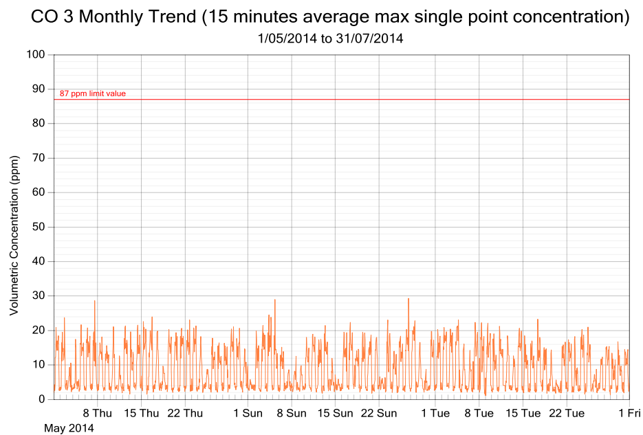
Figure 6: CO exposure and single point 15 minutes rolling averages from May to July 2014 (3 monthly trend)
