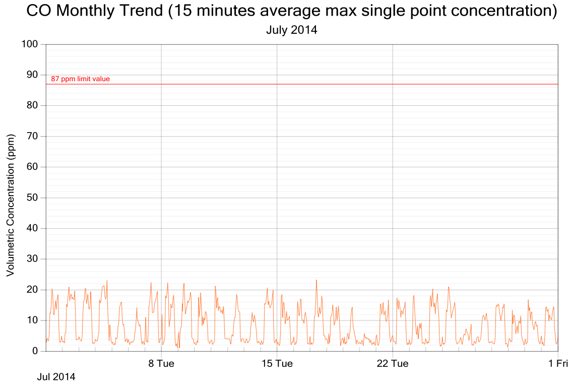
Figure 3: CO exposure and single point 15 minutes rolling averages for July 2014
