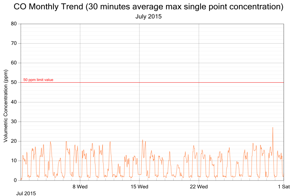
Figure 4: CO exposure and single point 30 minutes rolling averages for July 2015
