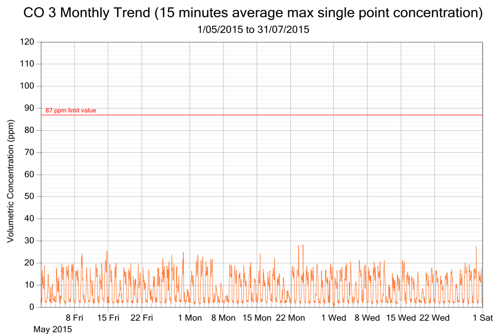
Figure 6: CO exposure and single point 15 minutes rolling averages from May 2015 to July 2015 (3 monthly trend)
