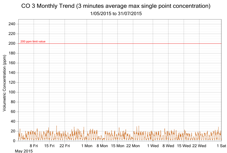
Figure 5: CO exposure and single point 3 minutes rolling averages from May 2015 to July 2015 (3 monthly trend)
