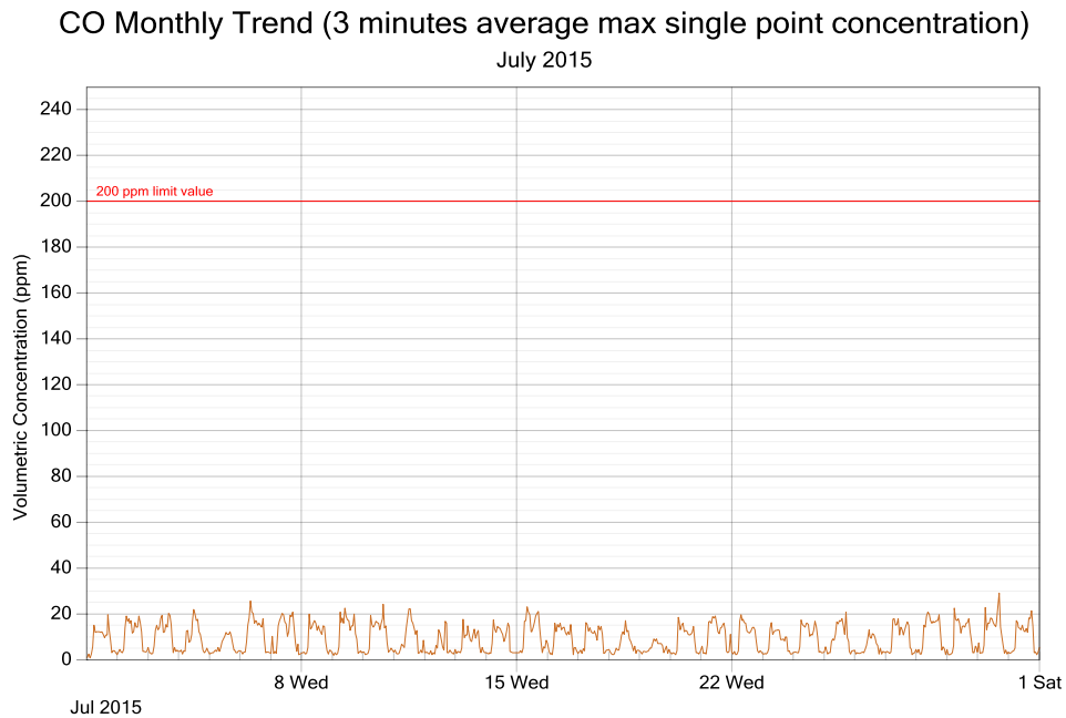
Figure 2: CO exposure and single point 3 minutes rolling averages for July 2015
