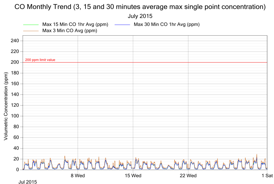
Figure 7: CO exposure and single point 30 minutes rolling averages from May 2015 to July 2015 (3 monthly trend)
