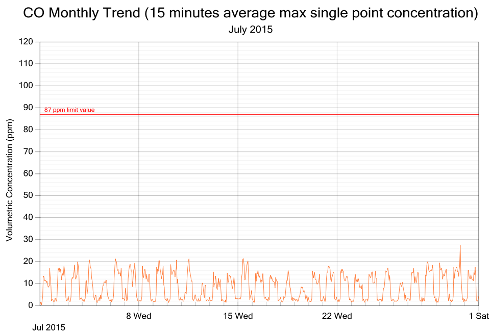
Figure 3: CO exposure and single point 15 minutes rolling averages for July 2015
