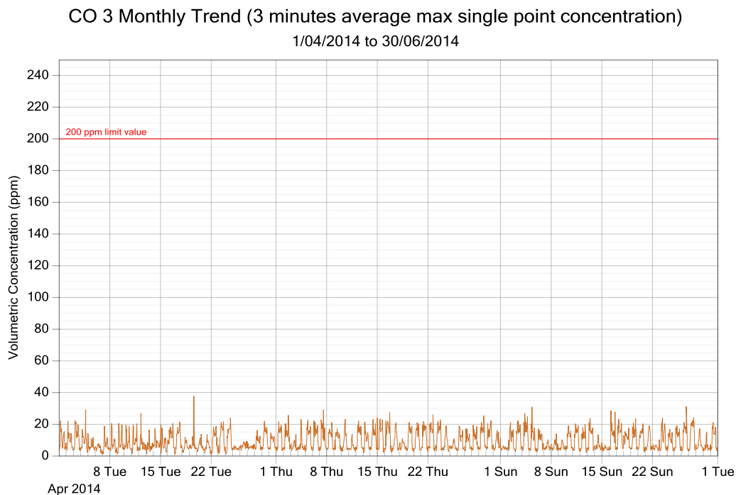
Figure 5: CO exposure and single point 3 minutes rolling averages from April to June 2014 (3 monthly trend)
