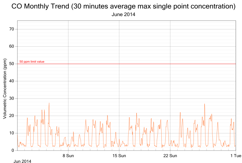
Figure 4: CO exposure and single point 30 minutes rolling averages for June 2014
