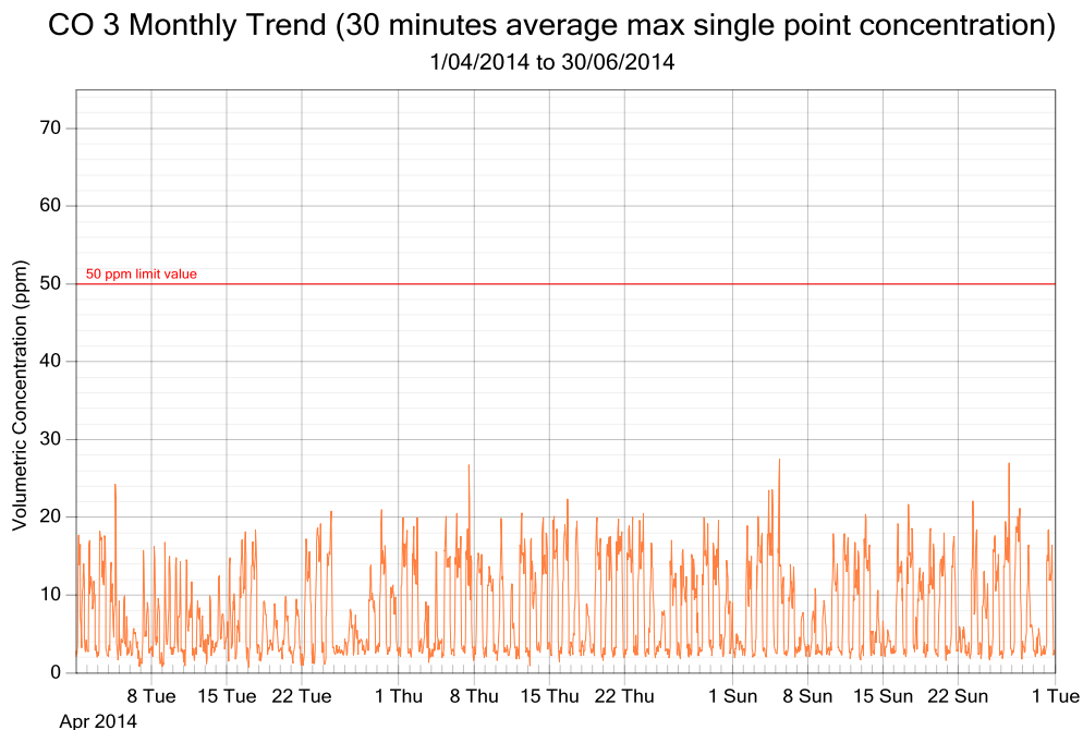
Figure 7: CO exposure and single point 30 minutes rolling averages from April to June 2014 (3 monthly trend)
