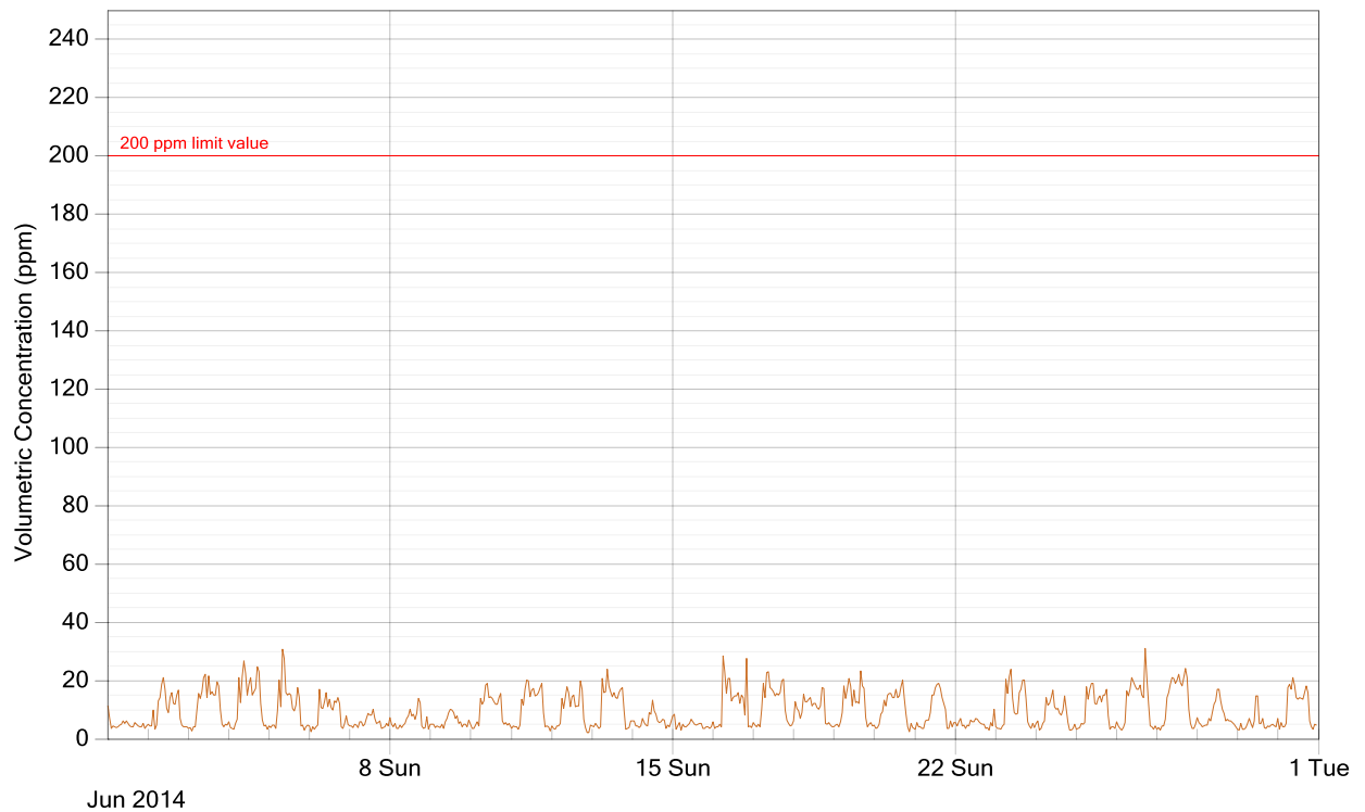
Figure 2: CO exposure and single point 3 minutes rolling averages for June 2014
