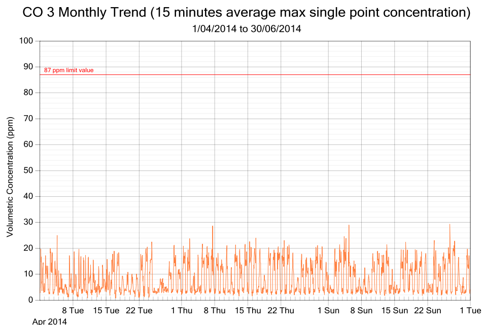
Figure 6: CO exposure and single point 15 minutes rolling averages from April to June 2014 (3 monthly trend)
