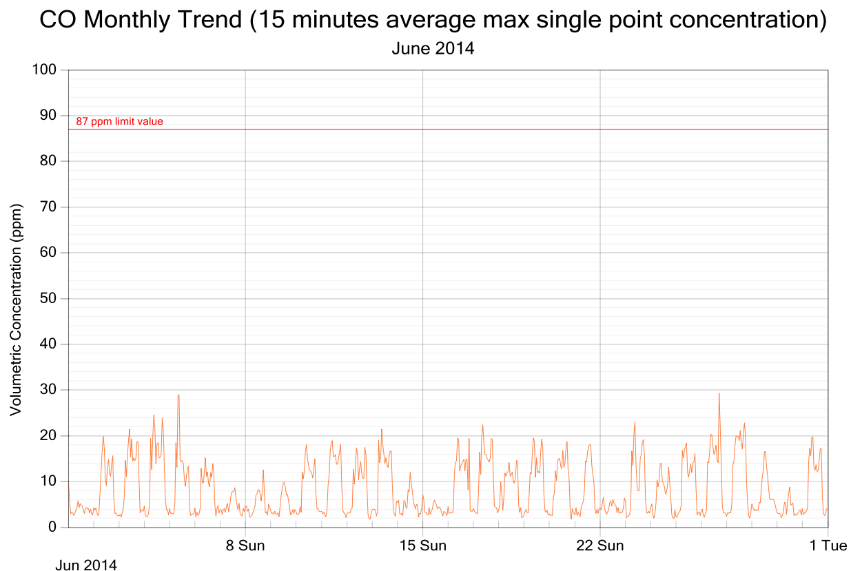
Figure 3: CO exposure and single point 15 minutes rolling averages for June 2014
