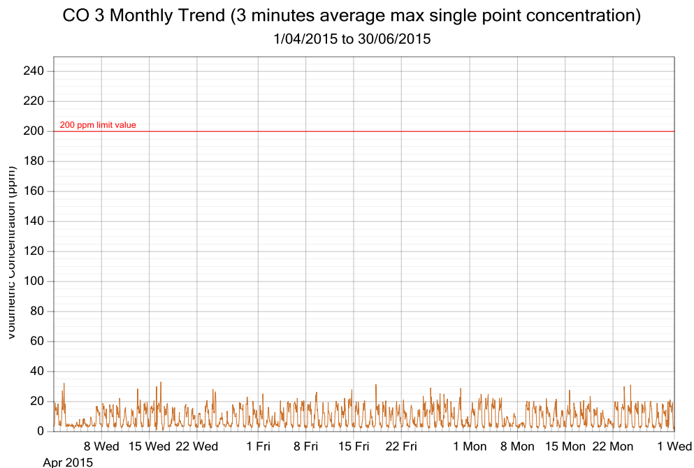
Figure 5: CO exposure and single point 3 minutes rolling averages from April 2015 to June 2015 (3 monthly trend)
