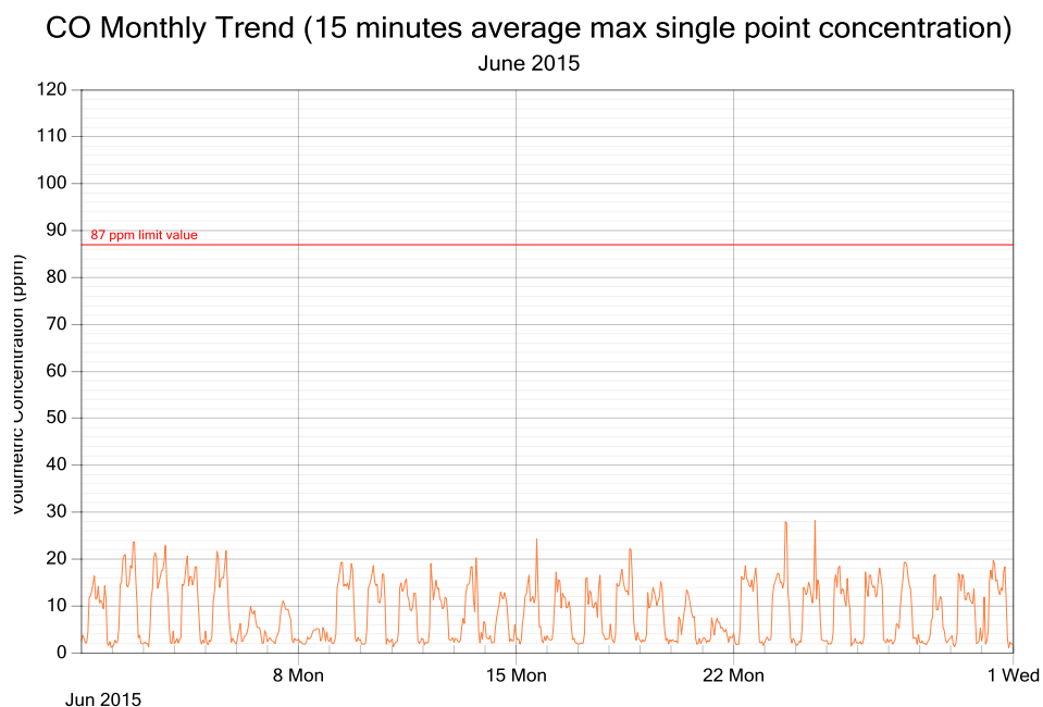
Figure 3: CO exposure and single point 15 minutes rolling averages for June 2015
