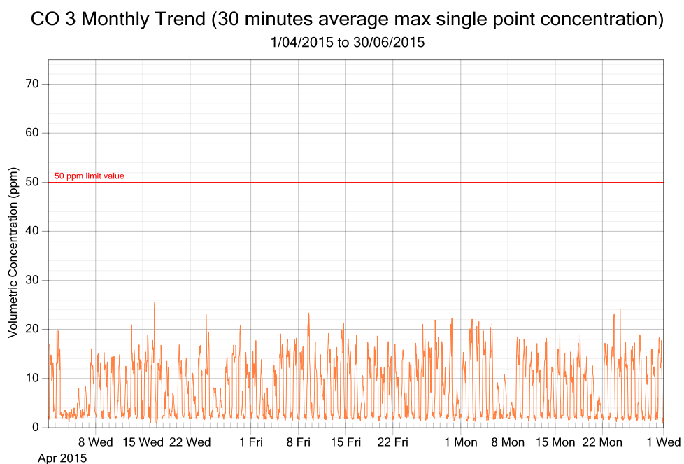
Figure 7: CO exposure and single point 30 minutes rolling averages from April 2015 to June 2015 (3 monthly trend)
