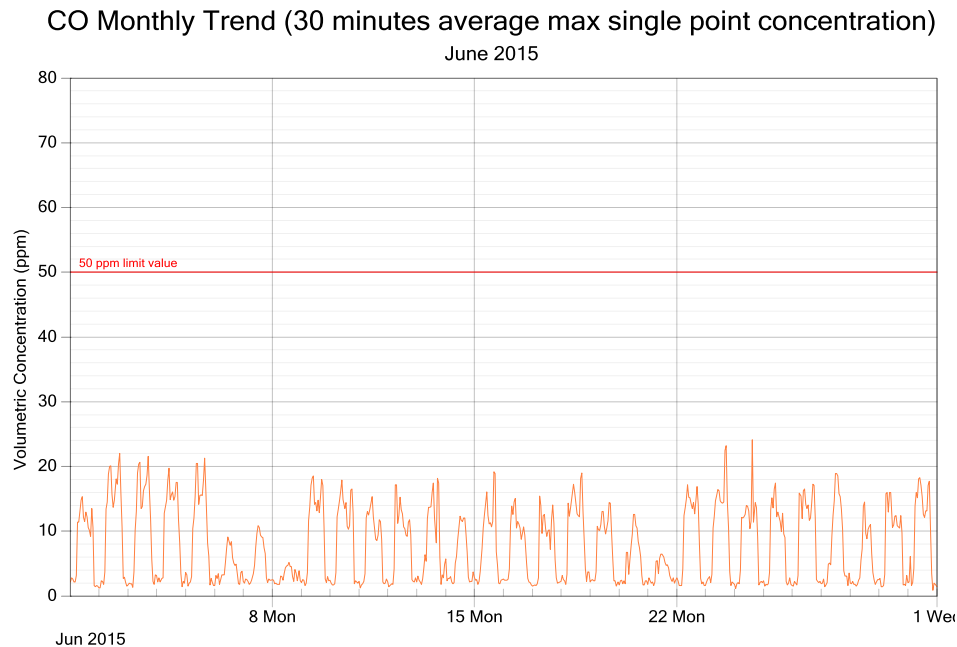
Figure 4: CO exposure and single point 30 minutes rolling averages for June 2015
