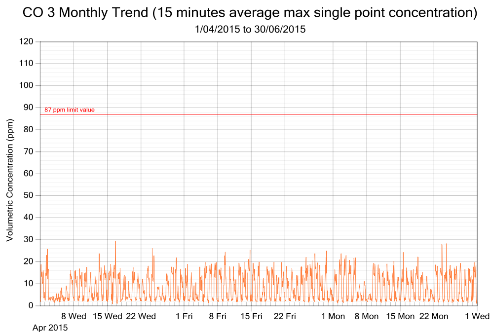
Figure 6: CO exposure and single point 15 minutes rolling averages from April 2015 to June 2015 (3 monthly trend)
