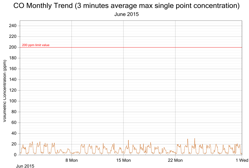
Figure 2: CO exposure and single point 3 minutes rolling averages for June 2015
