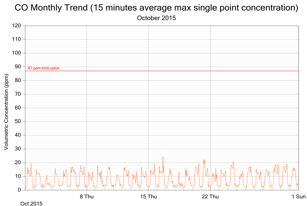
Figure 3: CO exposure and single point 15 minutes rolling averages for October 2015
