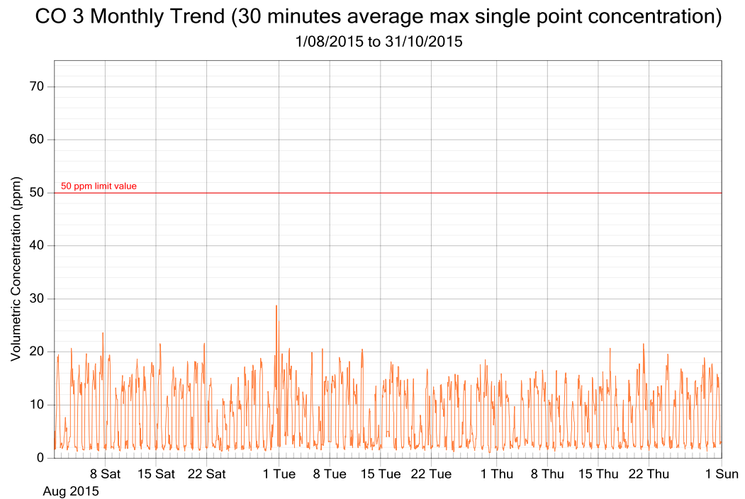
Figure 7: CO exposure and single point 30 minutes rolling averages from August 2015 to October 2015 (3 monthly trend)
