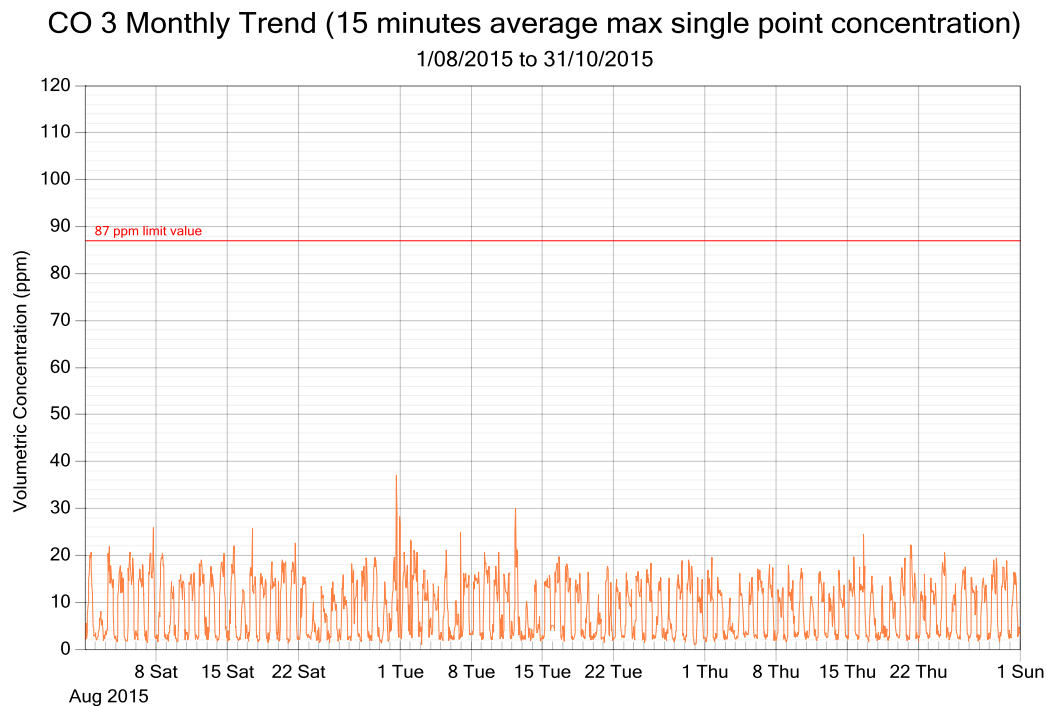
Figure 6: CO exposure and single point 15 minutes rolling averages from August 2015 to October 2015 (3 monthly trend)
