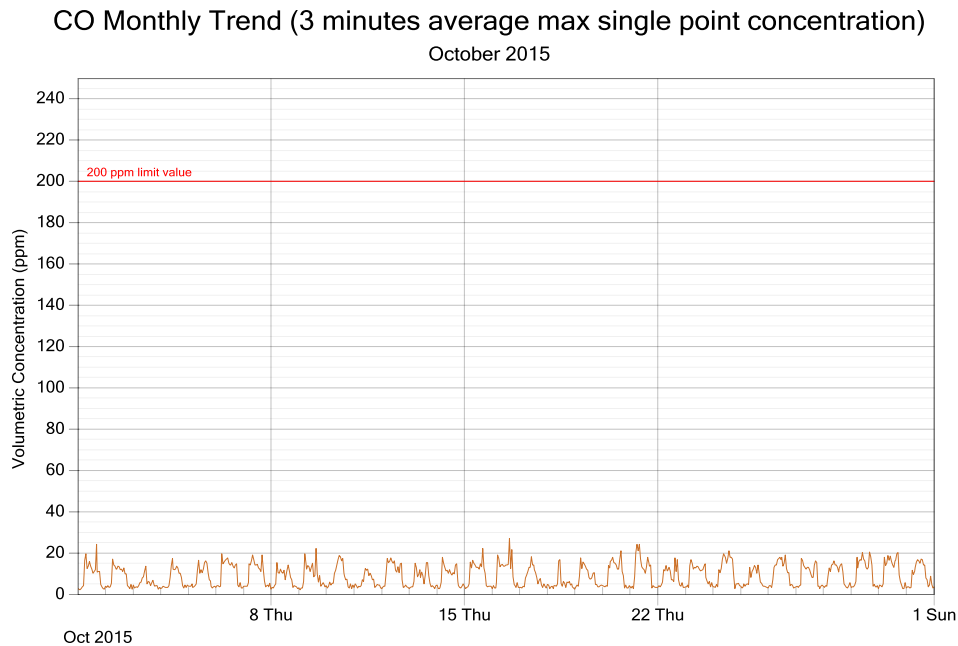
Figure 2: CO exposure and single point 3 minutes rolling averages for October 2015
