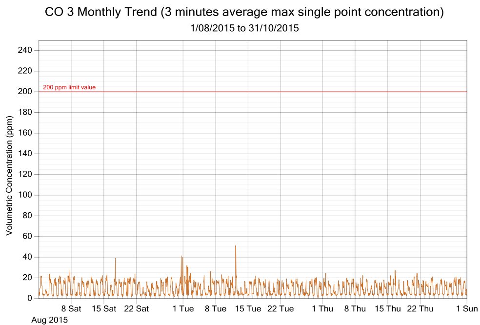
Figure 5: CO exposure and single point 3 minutes rolling averages from August 2015 to October 2015 (3 monthly trend)
