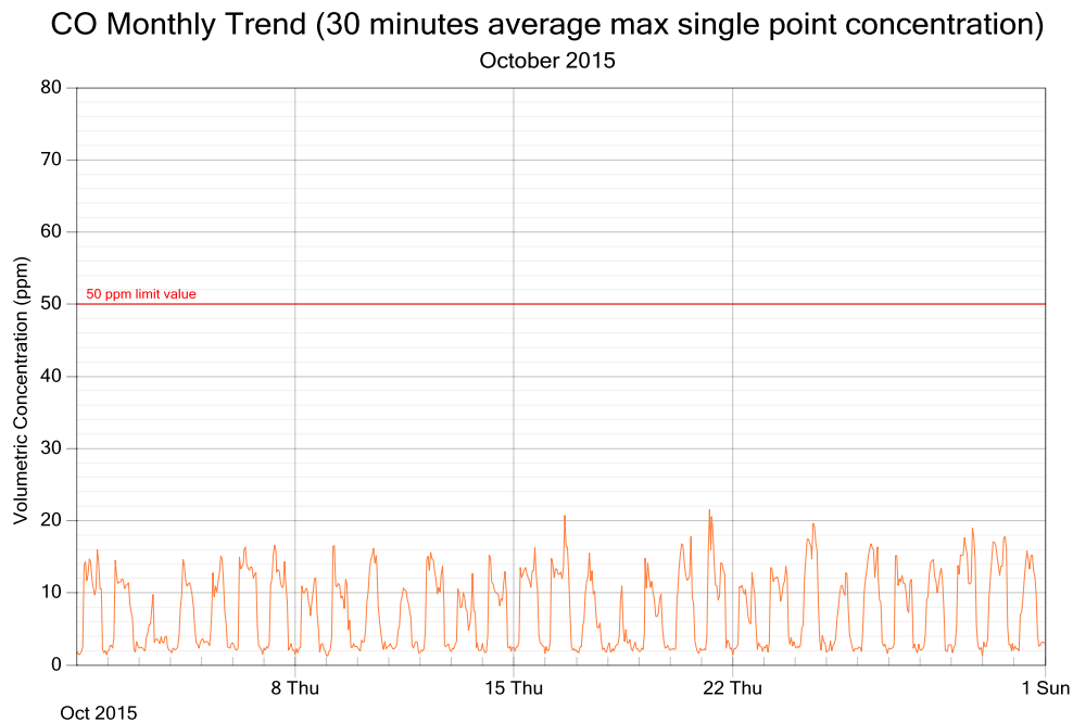
Figure 4: CO exposure and single point 30 minutes rolling averages for October 2015
