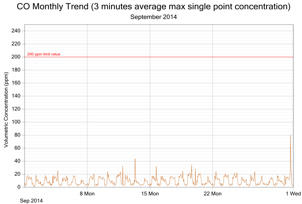
Figure 2: CO exposure and single point 3 minutes rolling averages for September 2014
