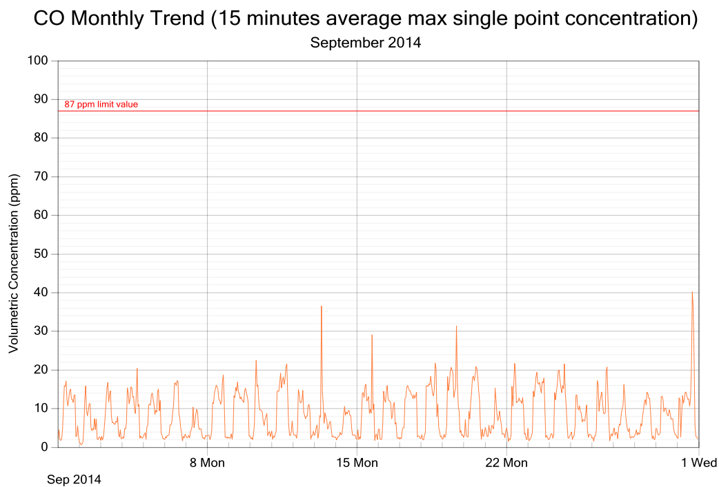
Figure 3: CO exposure and single point 15 minutes rolling averages for September 2014
