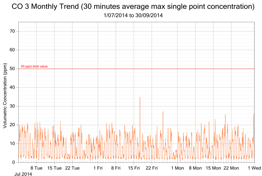
Figure 7: CO exposure and single point 30 minutes rolling averages from July to September 2014 (3 monthly trend)
