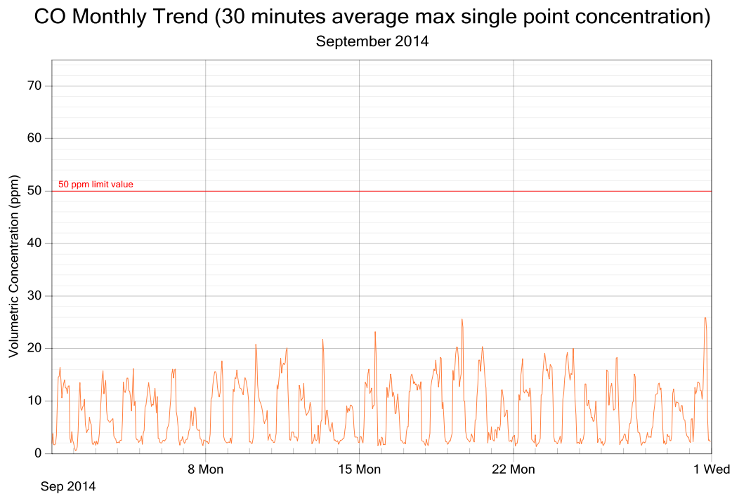
Figure 4: CO exposure and single point 30 minutes rolling averages for September 2014
