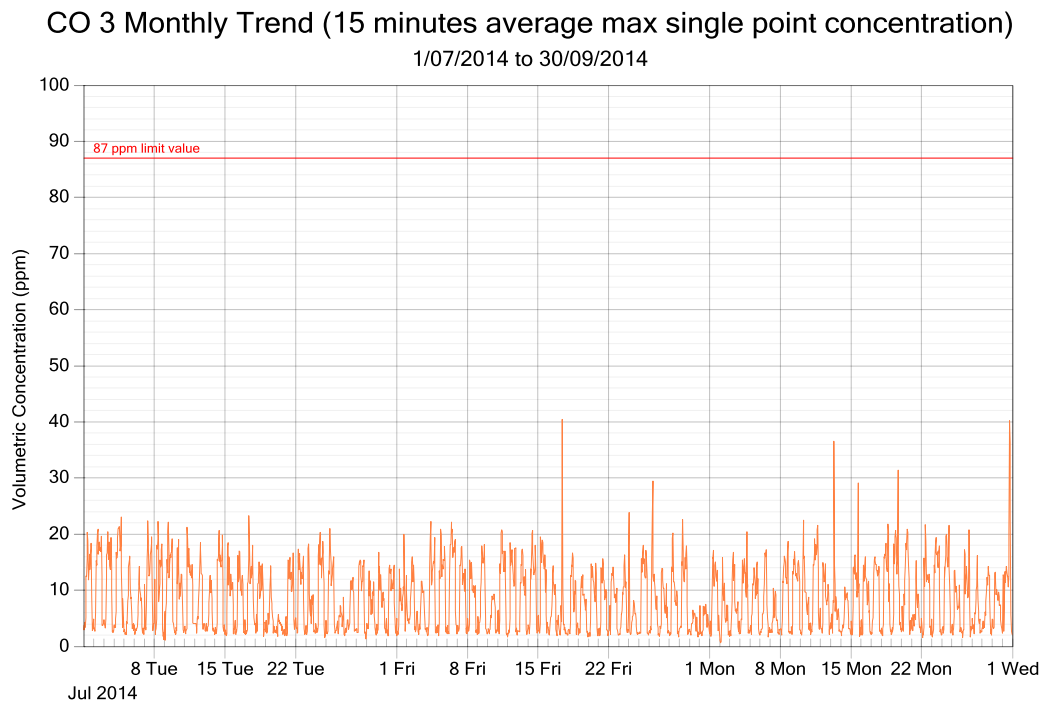
Figure 6: CO exposure and single point 15 minutes rolling averages from July to September 2014 (3 monthly trend)
