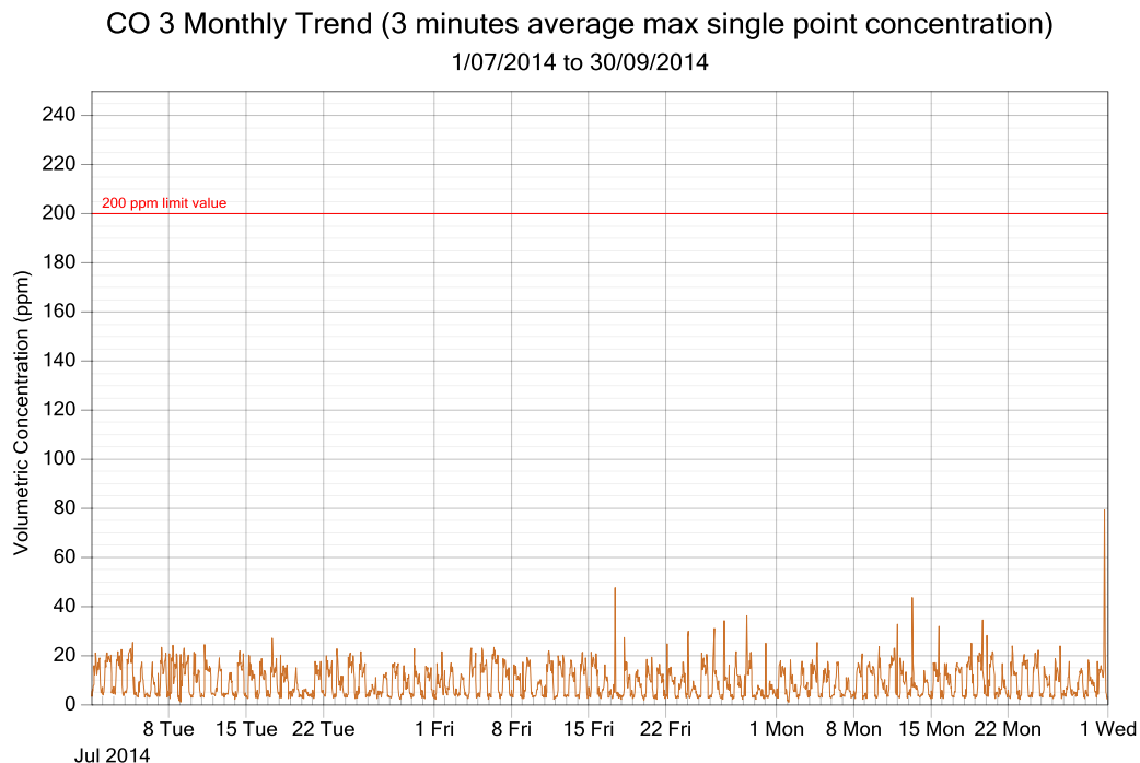
Figure 5: CO exposure and single point 3 minutes rolling averages from July to September 2014 (3 monthly trend)
