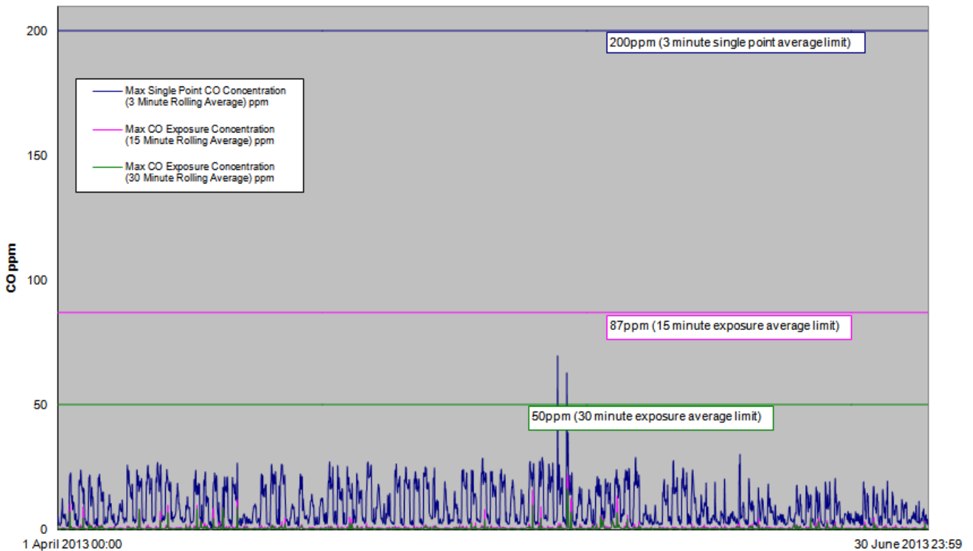
Figure 2: Graph of CO Exposure and Single Point Averages from 1 April 2013 to 30 June 2013
