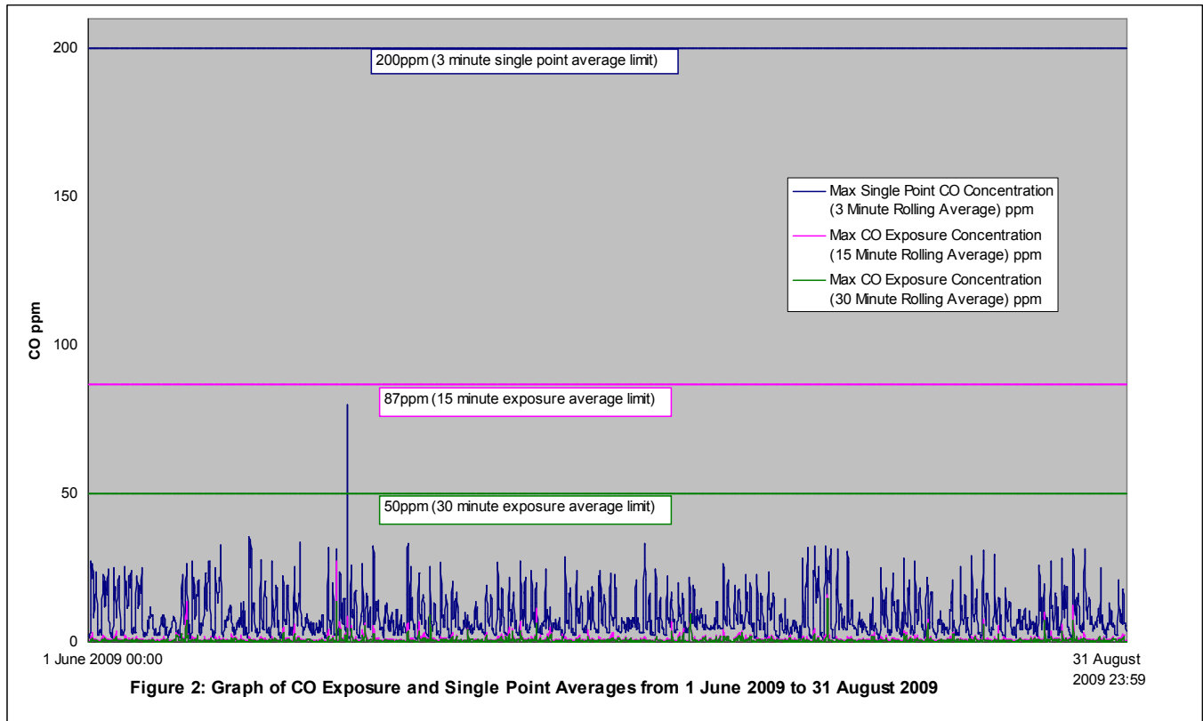
Figure 2: Graph of CO exposure and Single Point Averages from 01 June 2009 to 31 August 2009
